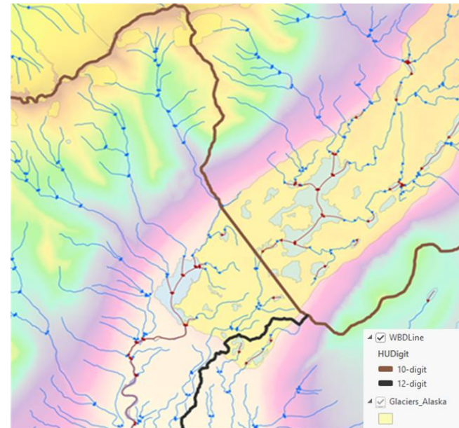
Break across at 1D tributary confluence
