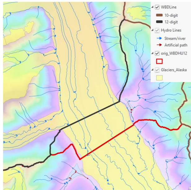
Move upstream to glacier confluence
