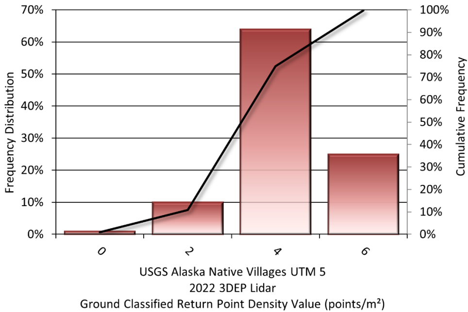
Figure 11: Frequency distribution of ground-classified return point density values per 100 x 100 m cell for UTM 5
