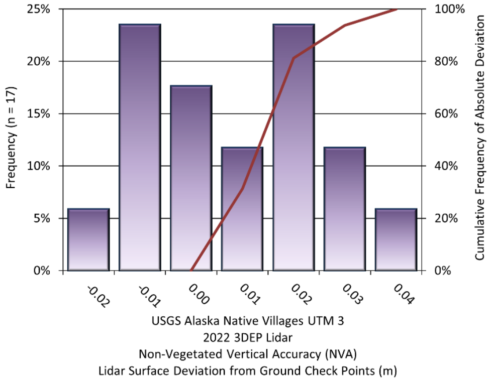
Figure 17: Frequency histogram for the lidar classified LAS deviation from ground check point values (NVA) for the zone UTM 3
