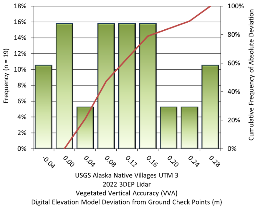
Figure 30: Frequency histogram for the lidar bare earth DEM deviation from vegetated check point values (VVA) for the zone UTM 3
