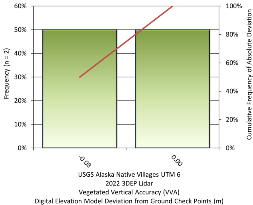
Figure 36: Frequency histogram for the lidar bare earth DEM deviation from vegetated check point values (VVA) for the zone UTM 6
