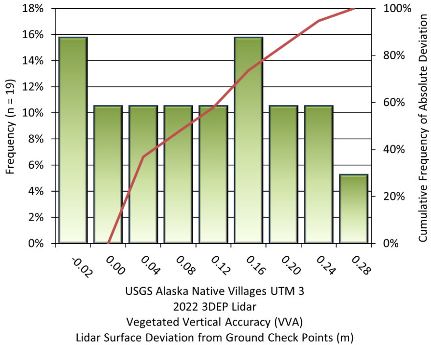
Figure 29: Frequency histogram for the lidar surface deviation from all land cover class point values (VVA) for the zone UTM 3
