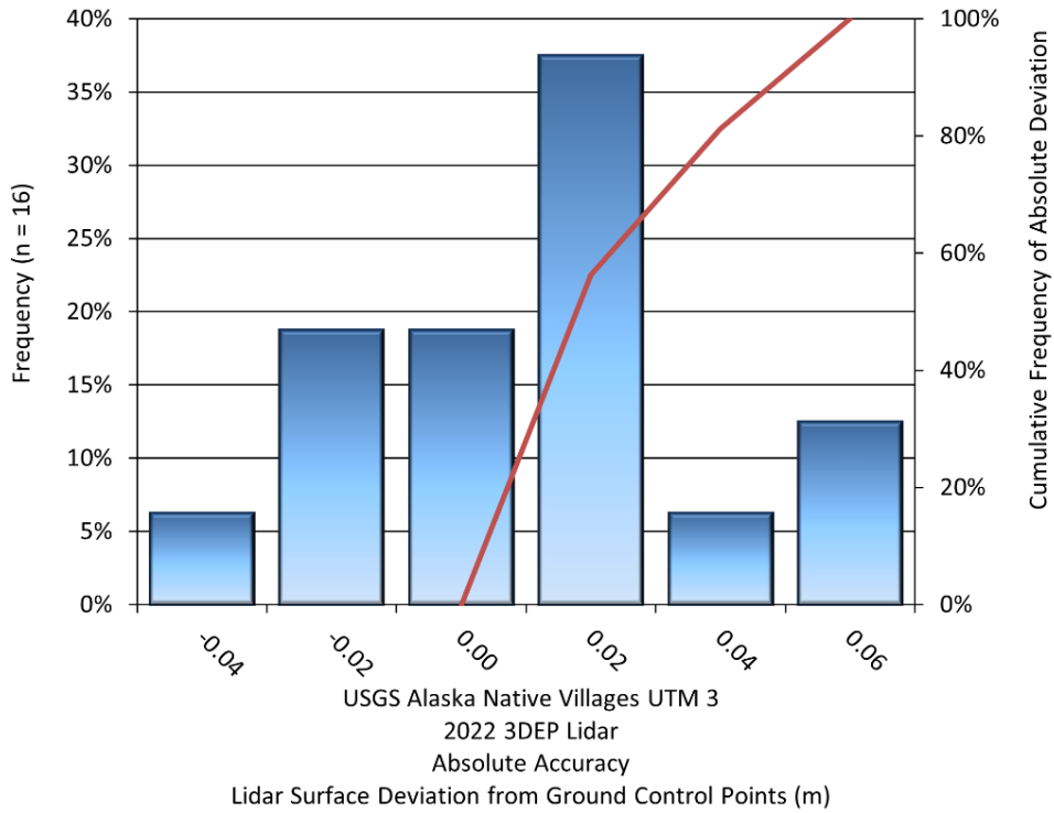
Figure 19: Frequency histogram for the lidar surface deviation from ground control point values for the zone UTM 3
