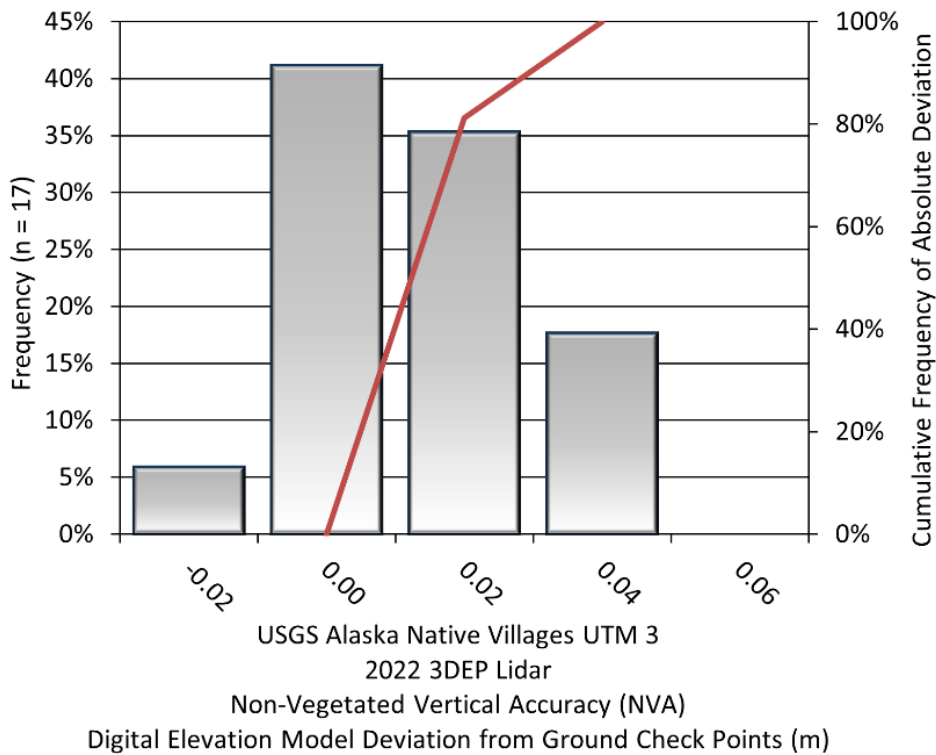
Figure 18: Frequency histogram for the lidar bare earth DEM surface deviation from ground check point values (NVA) for the zone UTM 3
