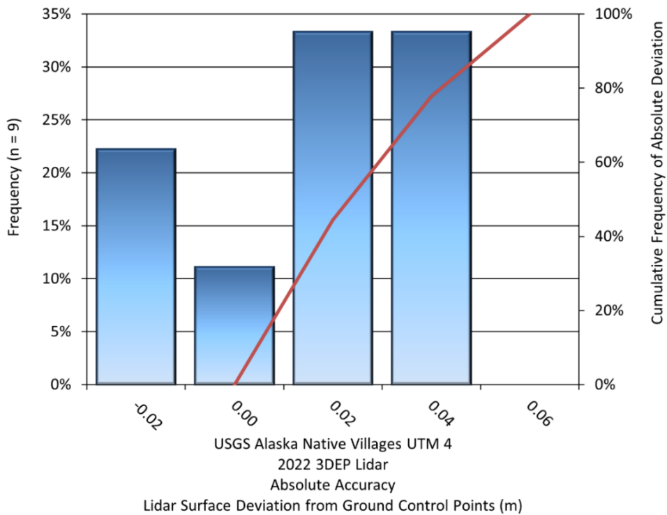
Figure 22: Frequency histogram for the lidar surface deviation from ground control point values for the zone UTM 4
