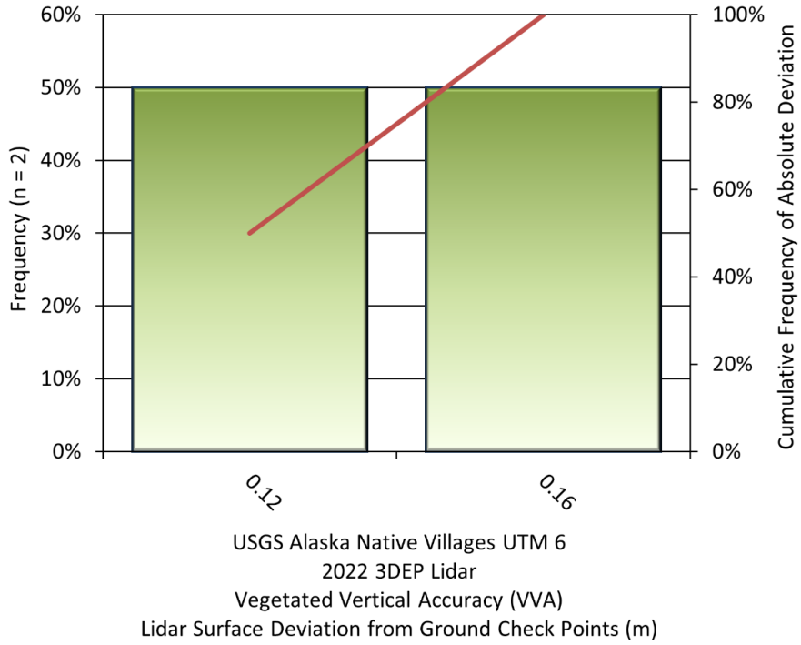
Figure 35: Frequency histogram for the lidar surface deviation from all land cover class point values (VVA) for the zone UTM 6
