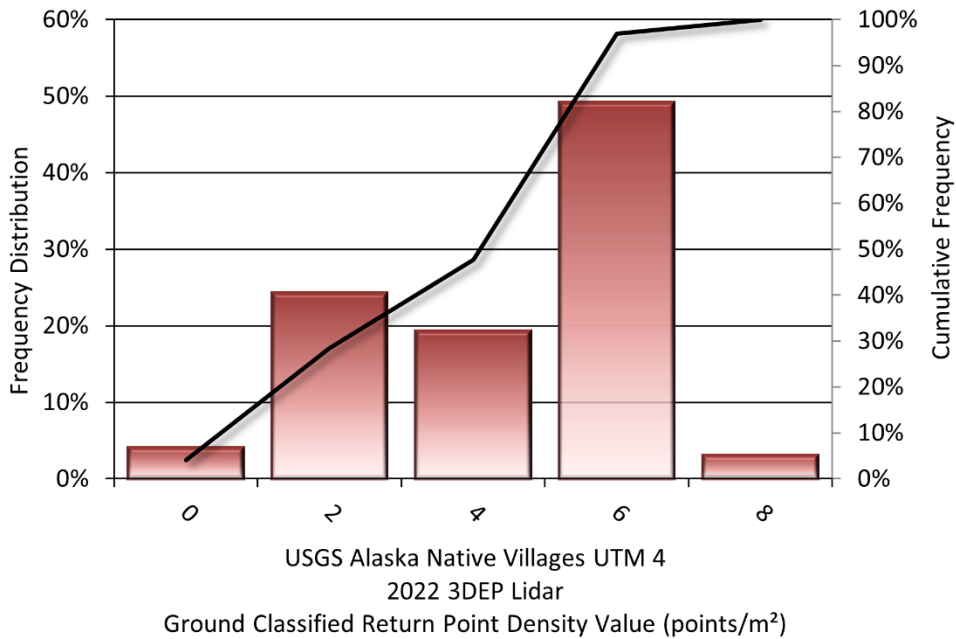
Figure 10: Frequency distribution of ground-classified return point density values per 100 x 100 m cell for UTM 4
