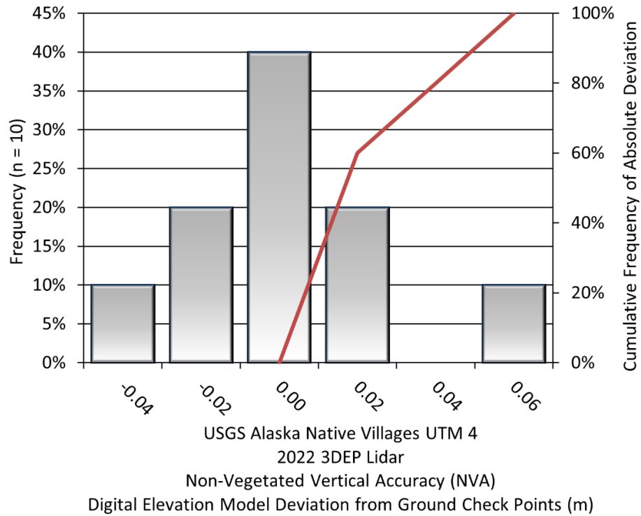
Figure 21: Frequency histogram for the lidar bare earth DEM surface deviation from ground check point values (NVA) for the zone UTM 4
