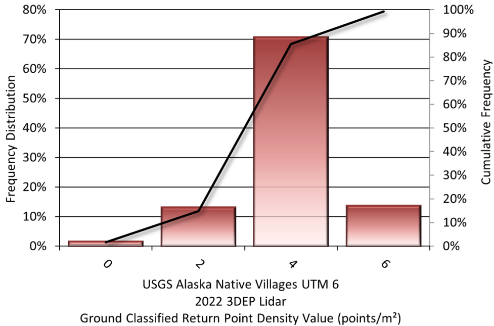
Figure 13: Frequency distribution of ground-classified return point density values per 100 x 100 m cell for UTM 6
