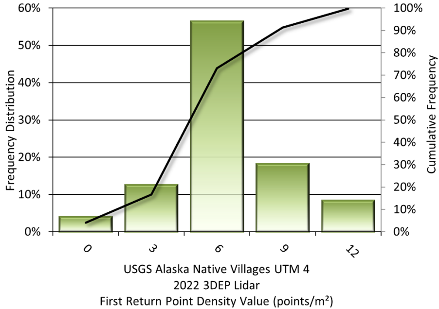
Figure 9: Frequency distribution of ground-classified return point density values per 100 x 100 m cell for UTM 4
