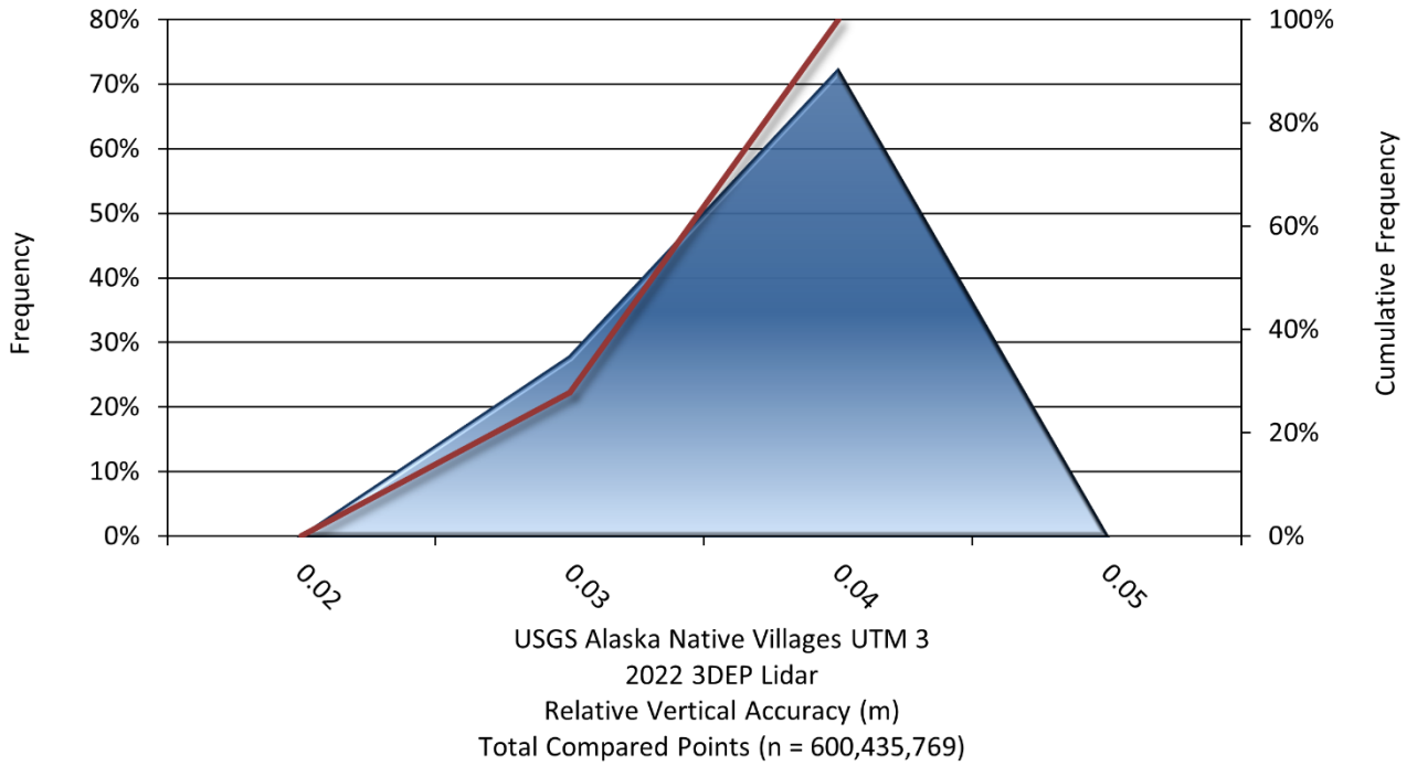
Figure 37: Frequency plot for the relative vertical accuracy between flight lines for UTM 3
