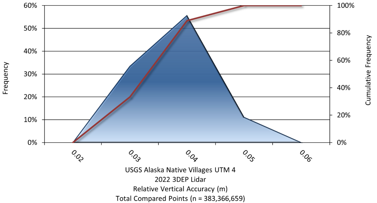
Figure 38: Frequency plot for the relative vertical accuracy between flight lines for UTM 4
