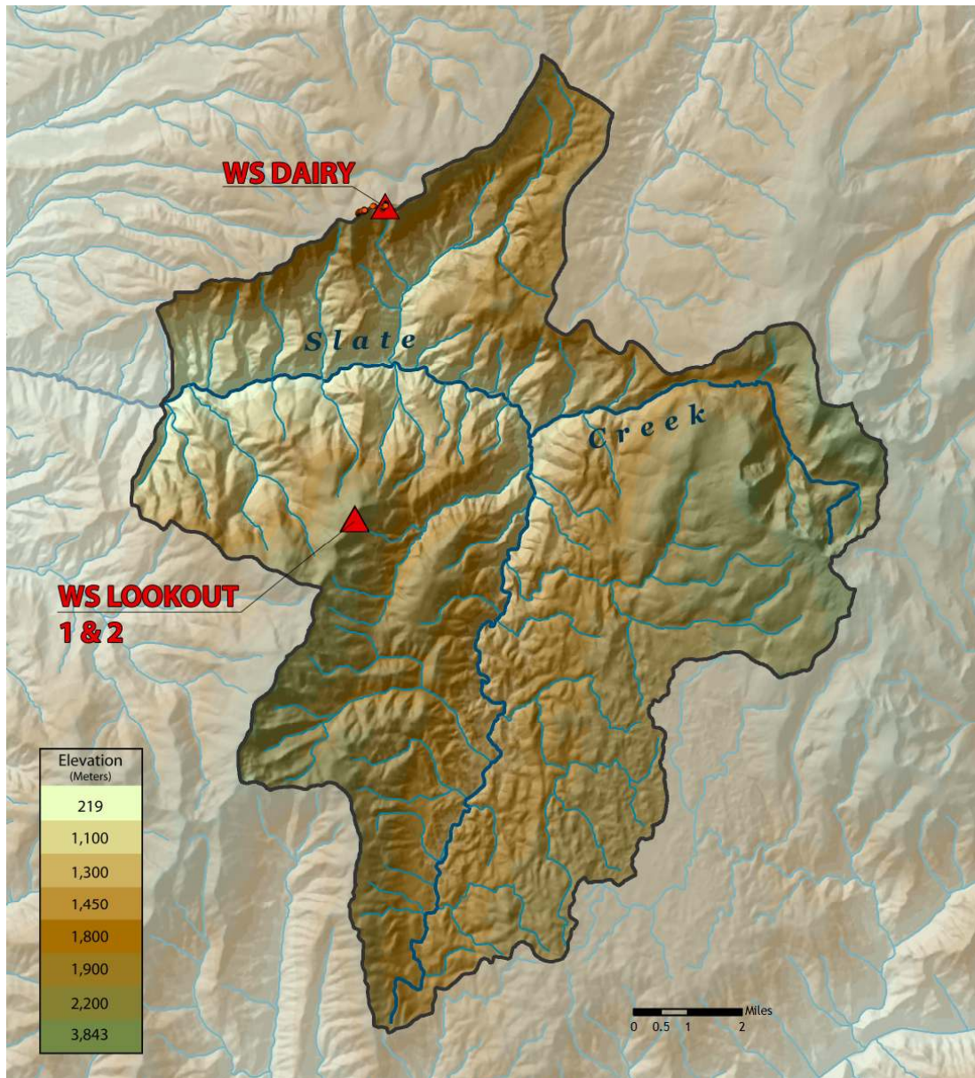
Figure 4. Locations of Base Stations and RTK Survey Point Collection in Slate Creek study area (3 Base Stations and 548 RTK Points).
