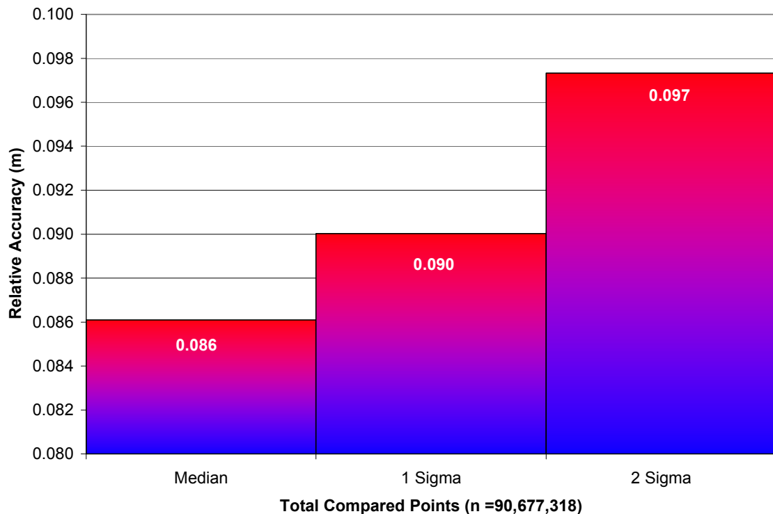
Figure 7. Statistical relative accuracies: Lolo Creek
