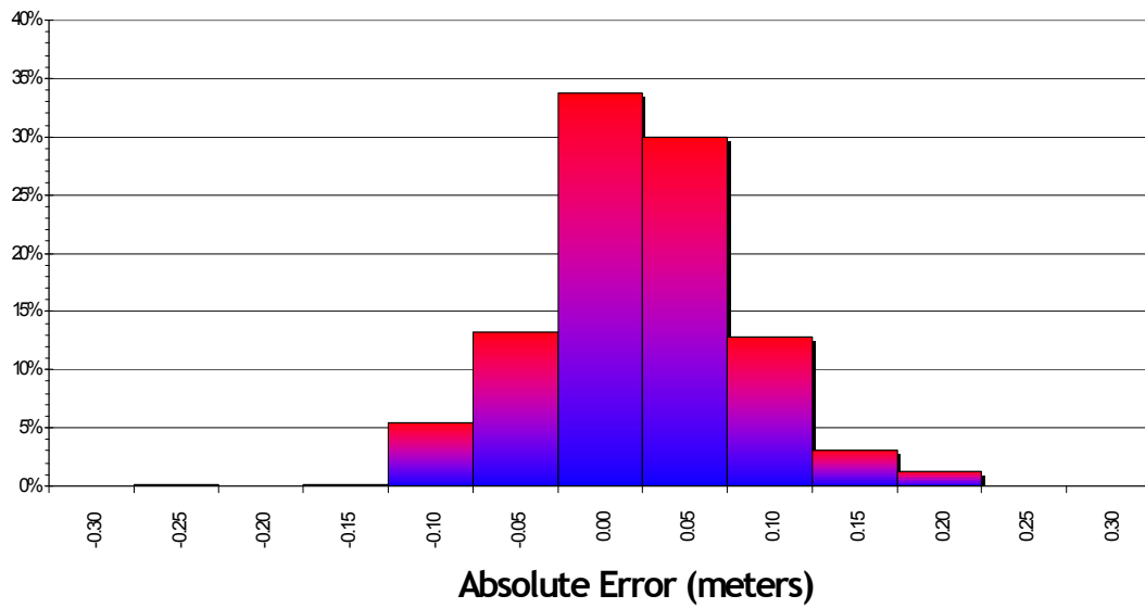
Figure 10. Point Absolute Deviation Statistics, Lolo Creek Study Area
