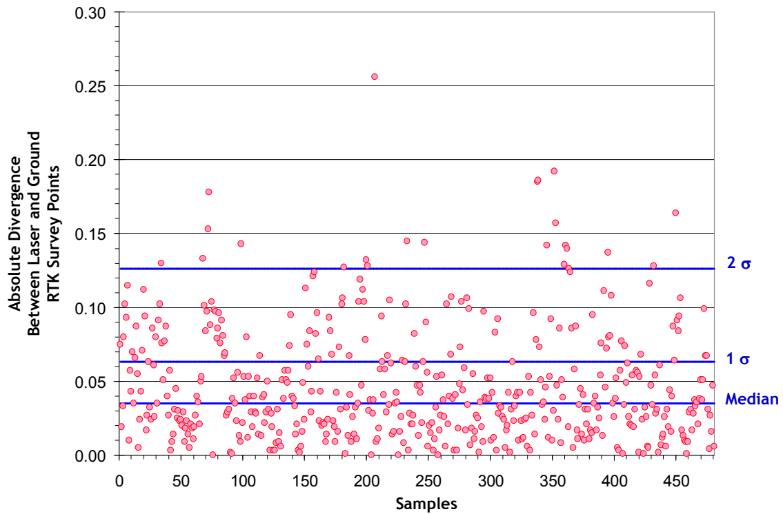
Figure 10. Point Absolute Deviation Statistics, Lolo Creek Study Area
