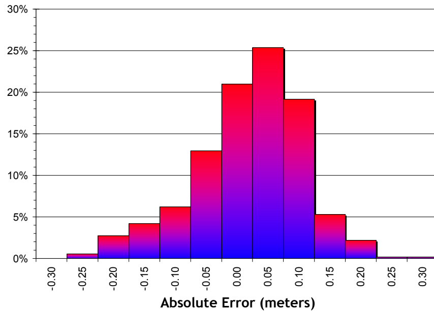
Figure 12. Point Absolute Deviation Statistics, Slate Creek Study Area
