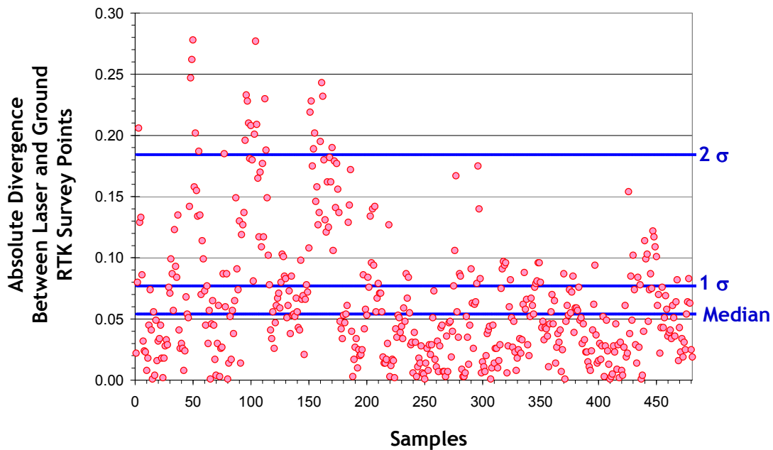
Figure 12. Point Absolute Deviation Statistics, Slate Creek Study Area
