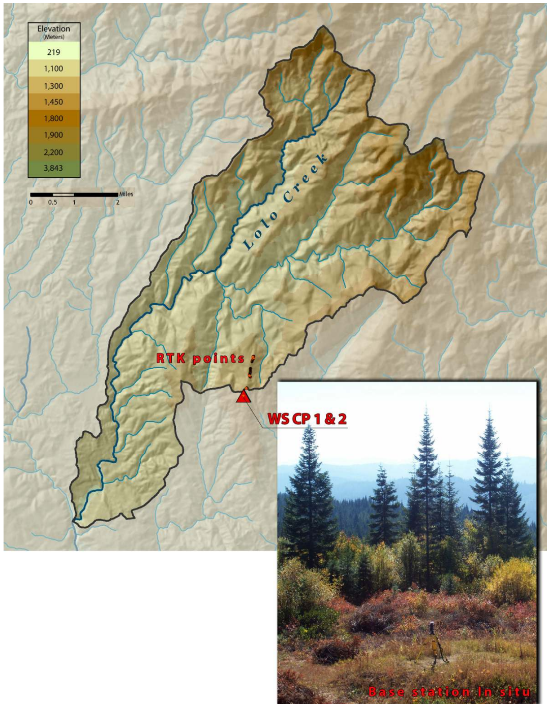
Figure 3. Locations of Base Stations and RTK Survey Point Collection in Lolo Creek study area (2 Base Stations and 481 RTK Points).
