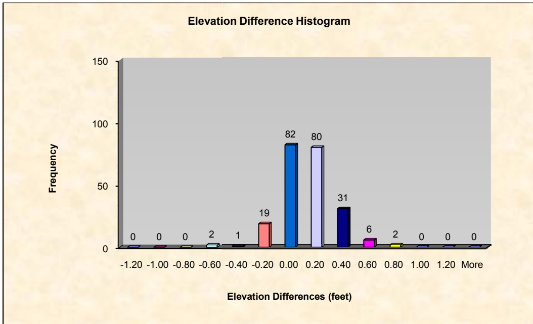
Figure 4: Histogram of Elevation Discrepancies within 0.2 ft bands
