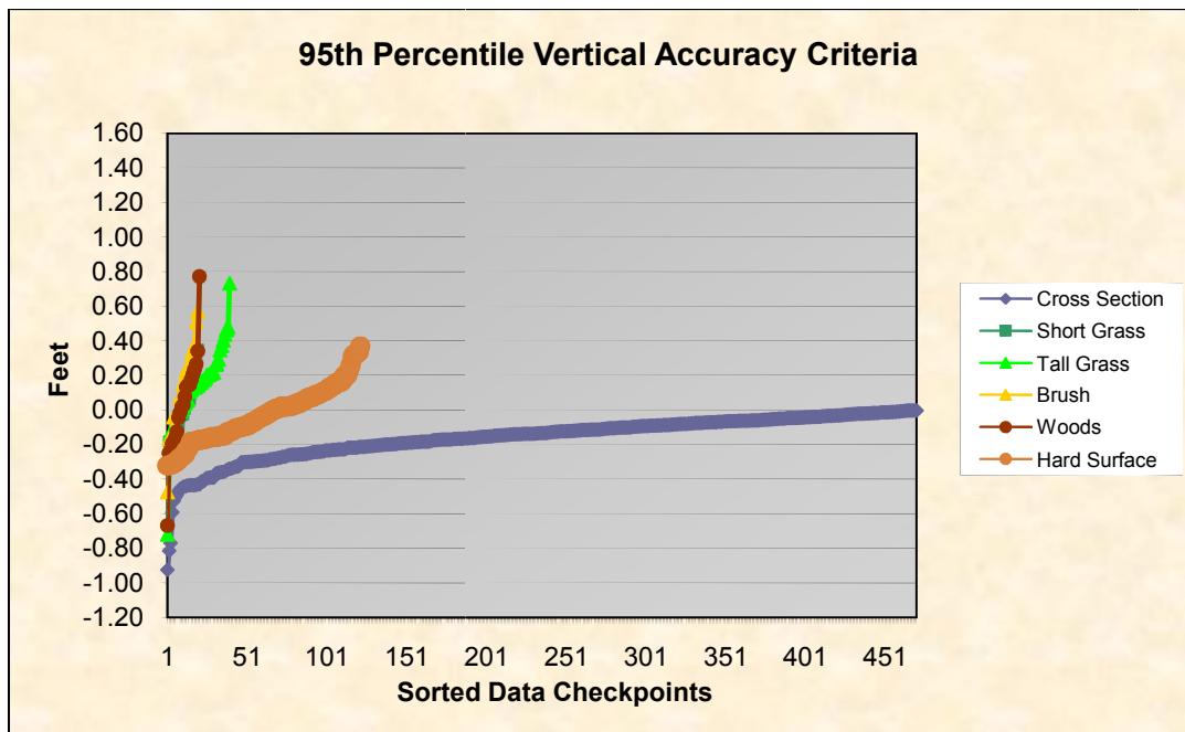
Figure 2: Magnitude of Elevation Discrepancies, Sorted from Largest Negative to Largest Positive
