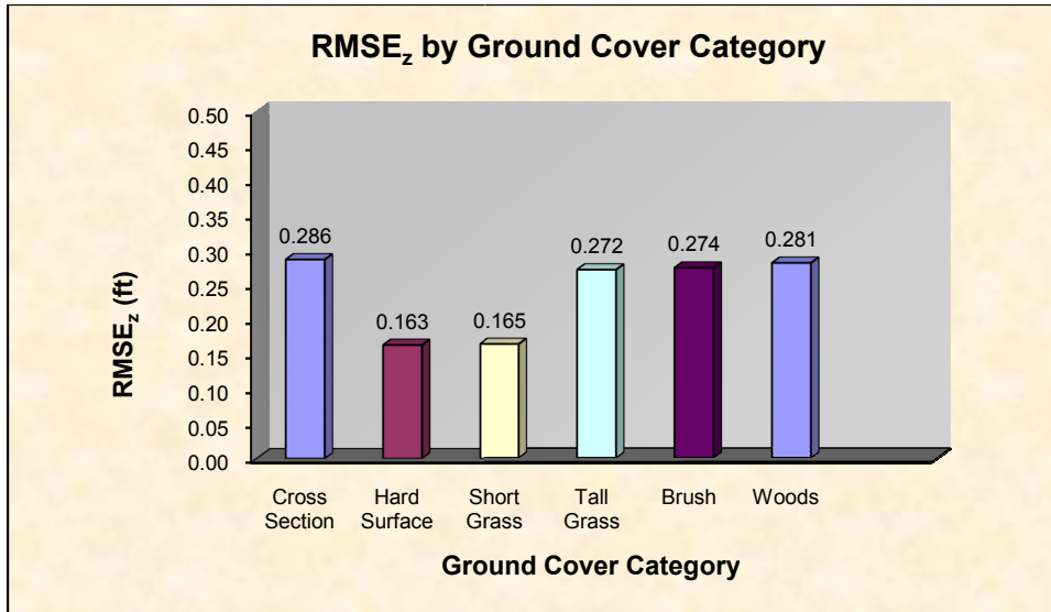
Figure 3: RMSE z statistics by Ground Cover Category
