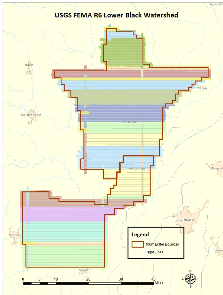
Figure 7: Lower Black Watershed Executed Flight Trajectories
