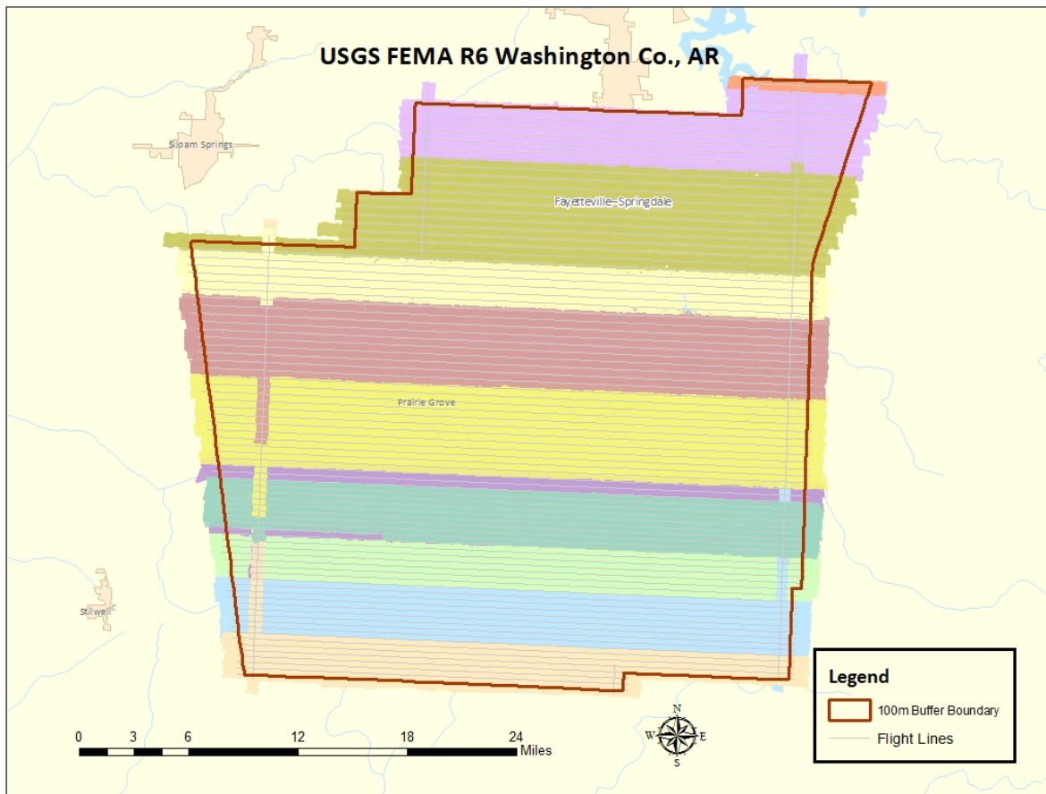
Figure 5: Washington County Executed Flight Trajectories
