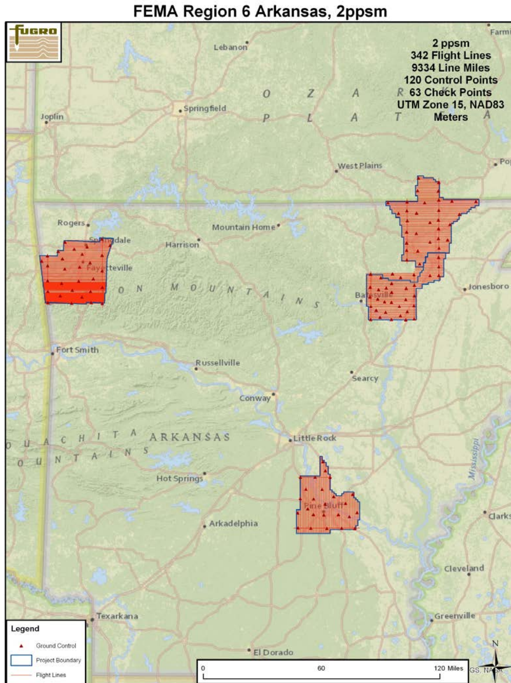
Figure 4: Planned Flight Diagram
