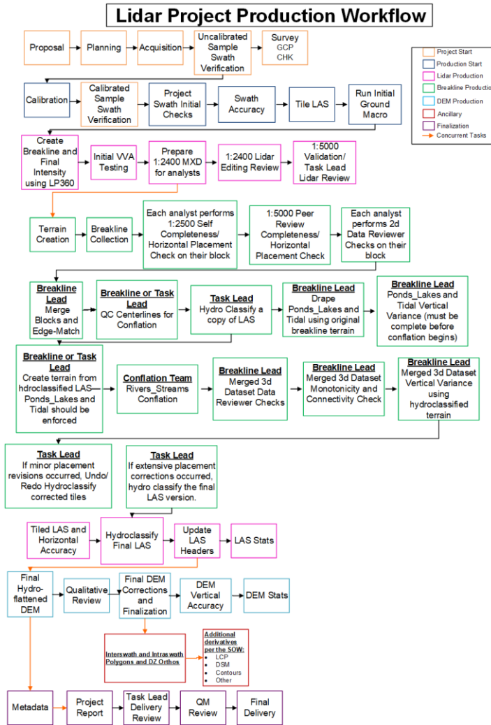
Figure 2 - Dewberry's lidar production workflow diagram.
