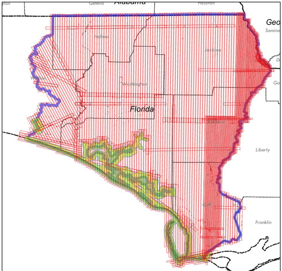
Figure 4 - Lidar swath output showing complete coverage.
