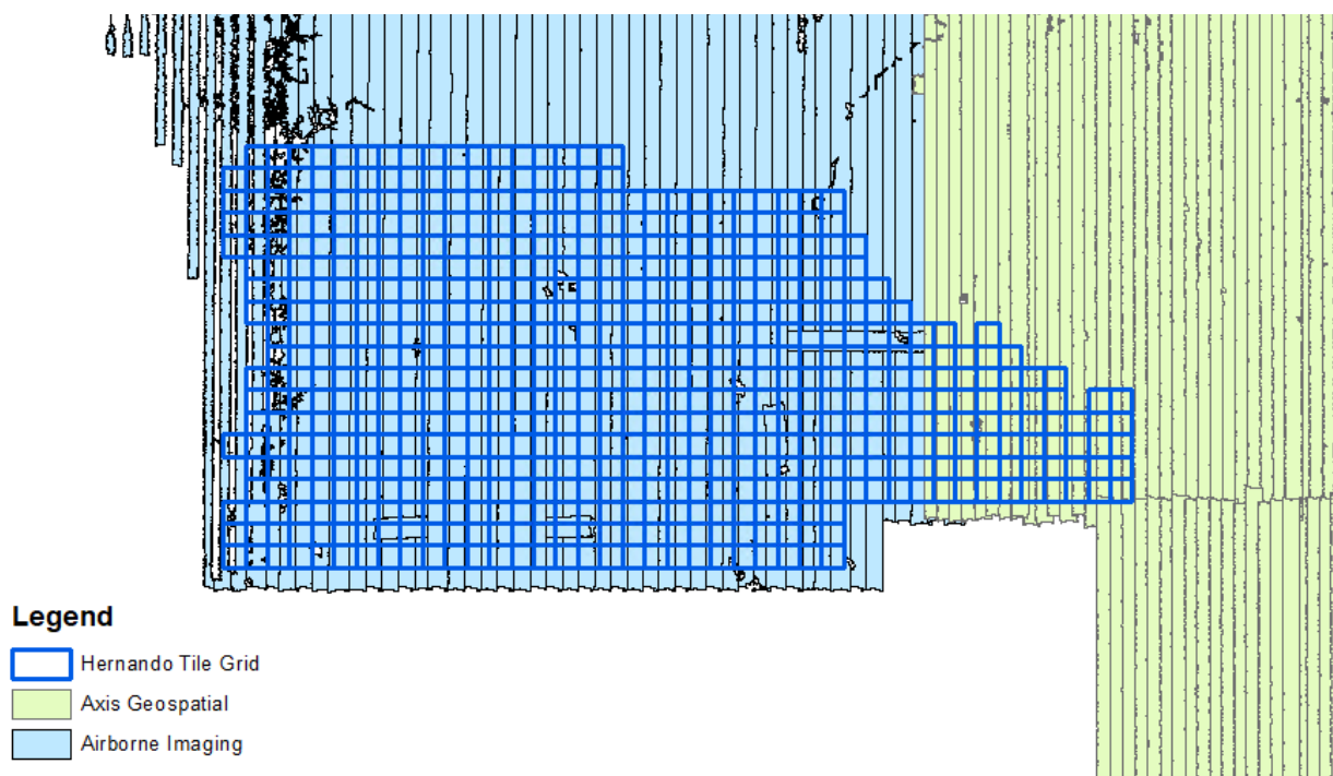
Figure 7- Flight lines flown by Axis Geospatial (green) and Airborne Imaging flight lines flown (light blue) overlaid with the Hernando delivery tile grid (blue), showing complete coverage.
