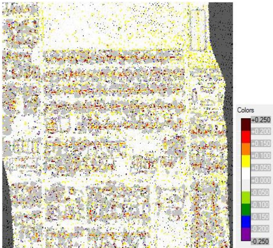
Figure 6a. QC block colored by vertical difference between swaths to check accuracy at swath edges by Airborne Imaging.
