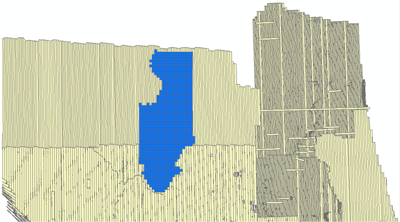
Figure 4 - Lidar swath output showing complete coverage.
