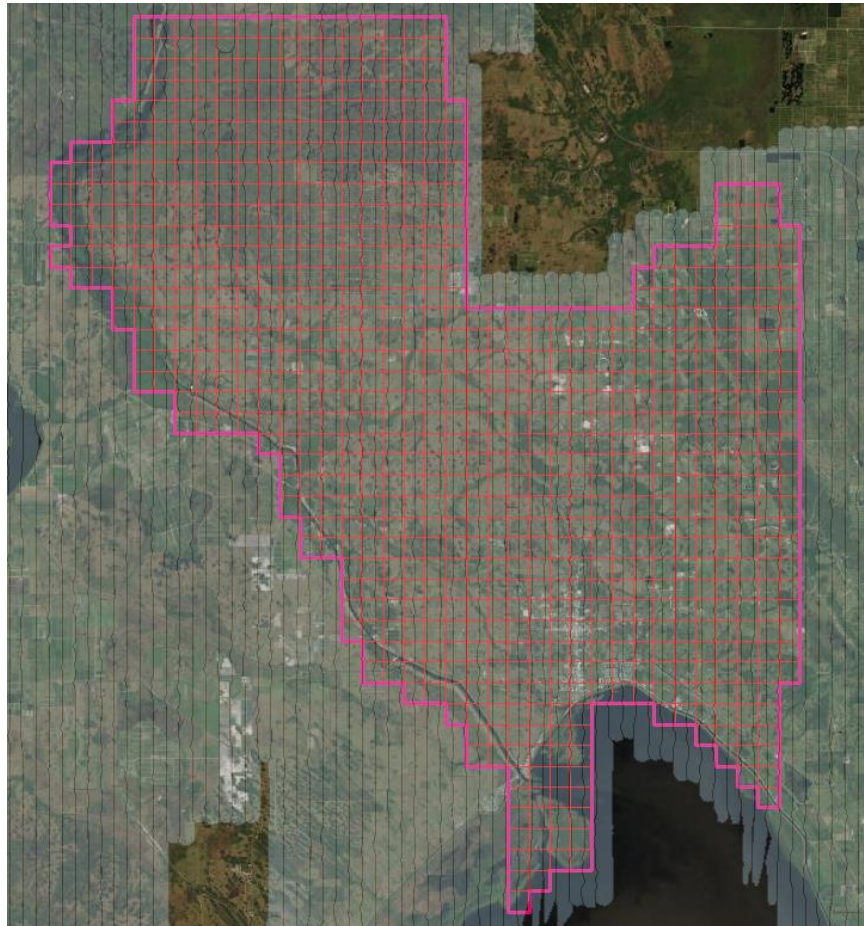
Figure 2. Lidar swath output showing complete coverage.
