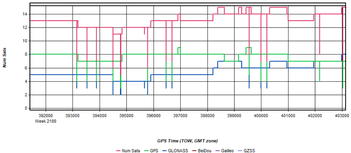
Figure 7: 20200409124226_13 [Smoothed TC Combined] - Number of Satellites Line Plot
