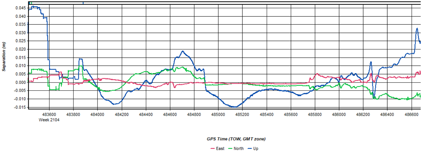
Figure 2: 20200508141615_26 [Smoothed TC Combined] - Forward/Reverse or Combined Separation Plot
