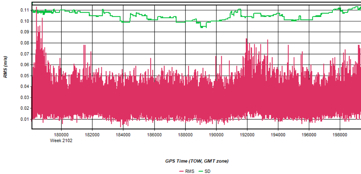
Figure 18: 20200421012658_23 [Smoothed TC Combined] - L1 Doppler Residual RMS Plot
