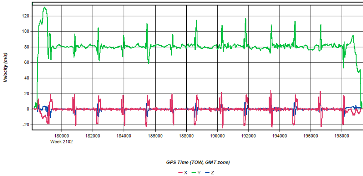
Figure 14: 20200421012658_23 [Smoothed TC Combined] - Body Frame Velocity Plot
