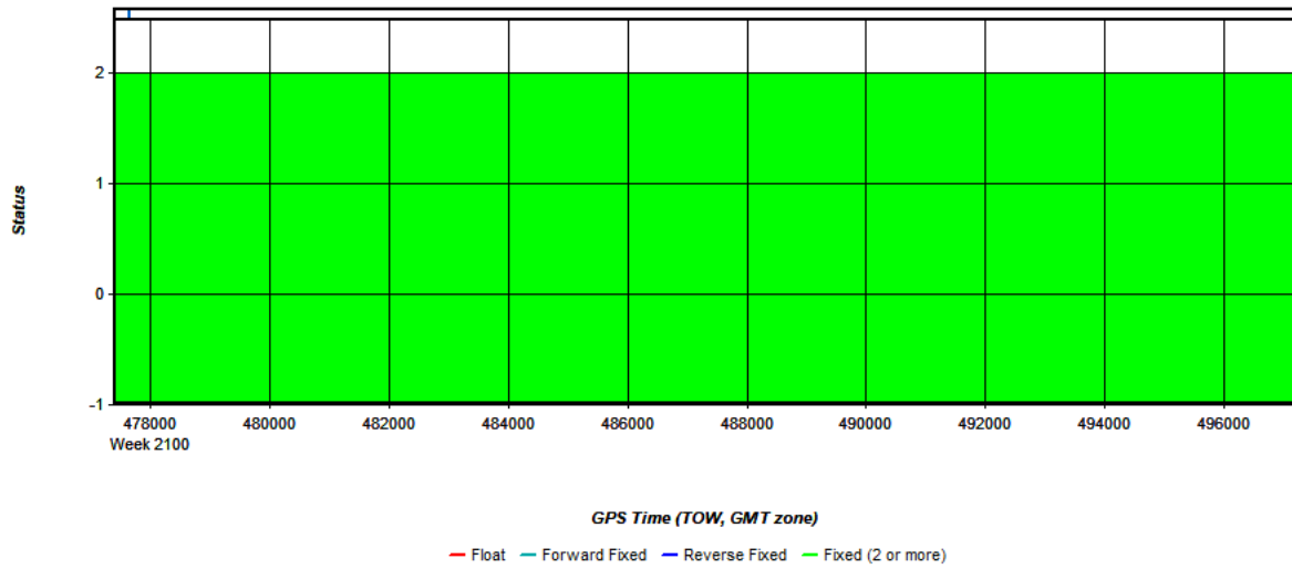
Figure 3: 20200410123525_15 [Smoothed TC Combined] - Float or Fixed Ambiguity
