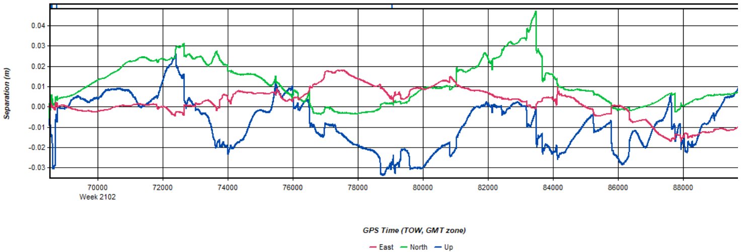
Figure 2: 20200419190050_22 [Smoothed TC Combined] - Forward/Reverse or Combined Separation Plot
