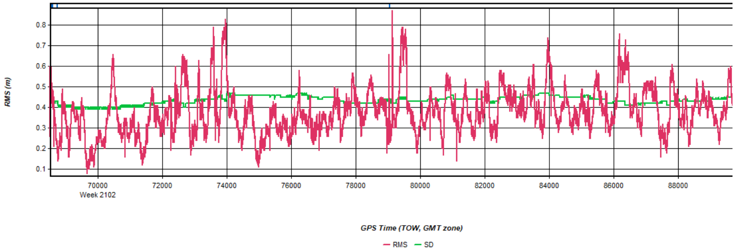
Figure 16: 20200419190050_22 [Smoothed TC Combined] - C/A Code Residual RMS Plot
