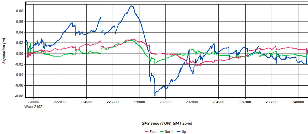
Figure 2: 20200421125525_24 [Smoothed TC Combined] - Forward/Reverse or Combined Separation Plot
