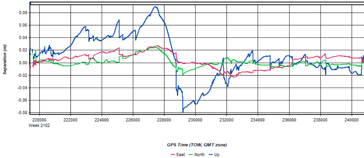
Figure 4: 20200421125525_24 [Smoothed TC Combined] - Forward/Reverse Separation Plot (Fixed)
