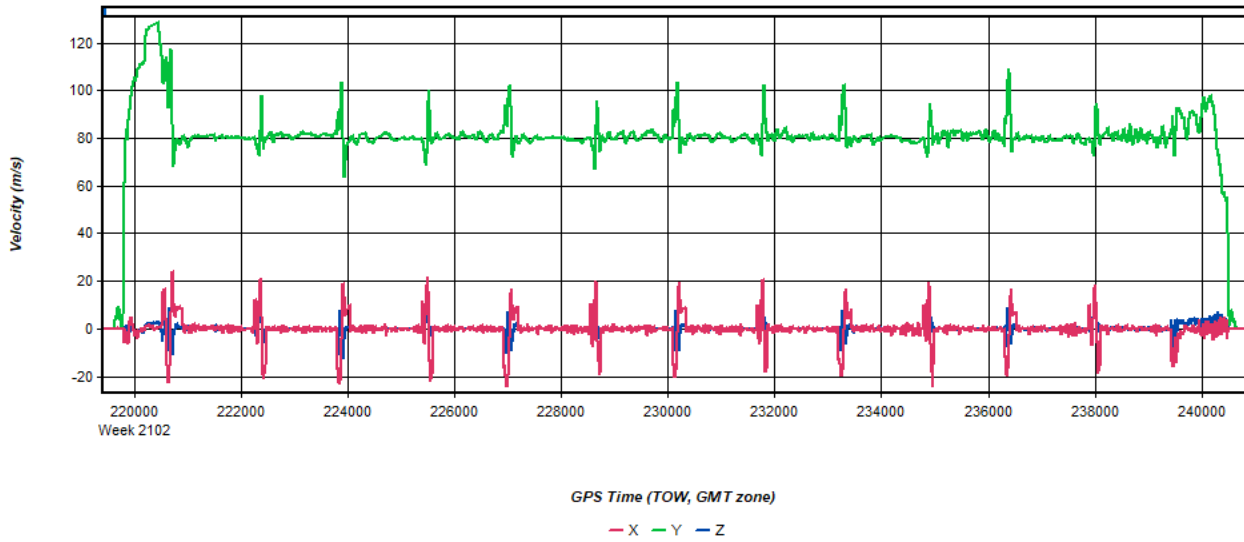
Figure 14: 20200421125525_24 [Smoothed TC Combined] - Body Frame Velocity Plot
