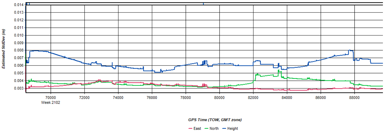
Figure 5: 20200419190050_22 [Smoothed TC Combined] - Estimated Position Accuracy Plot
