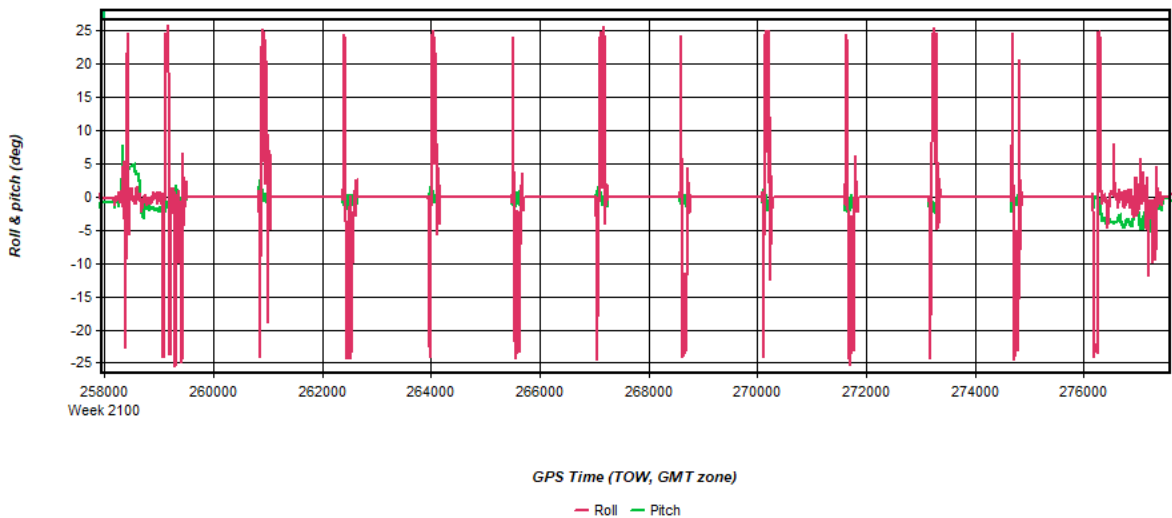
Figure 12: 20200407233739_11 [Smoothed TC Combined] - Roll & Pitch Plot
