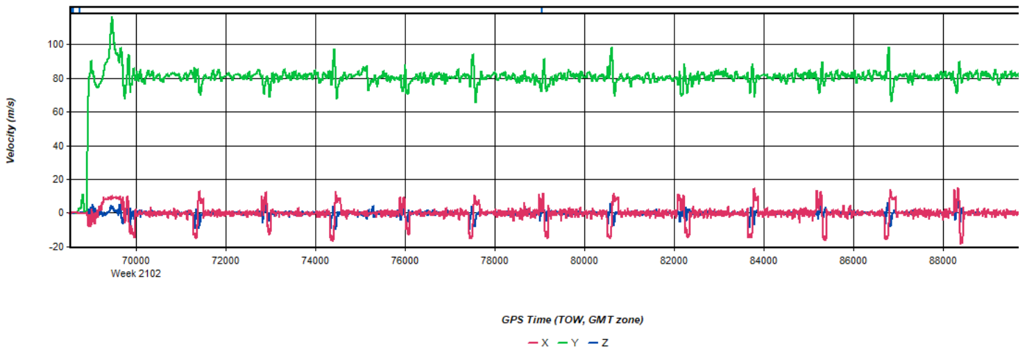
Figure 14: 20200419190050_22 [Smoothed TC Combined] - Body Frame Velocity Plot
