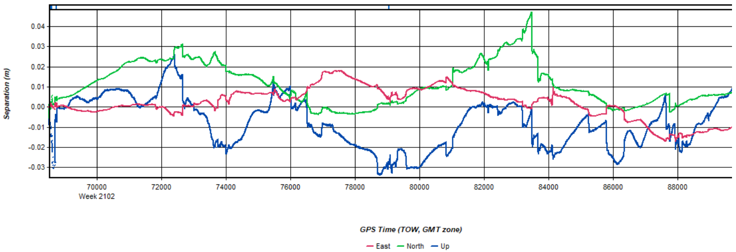
Figure 4: 20200419190050_22 [Smoothed TC Combined] - Forward/Reverse Separation Plot (Fixed)
