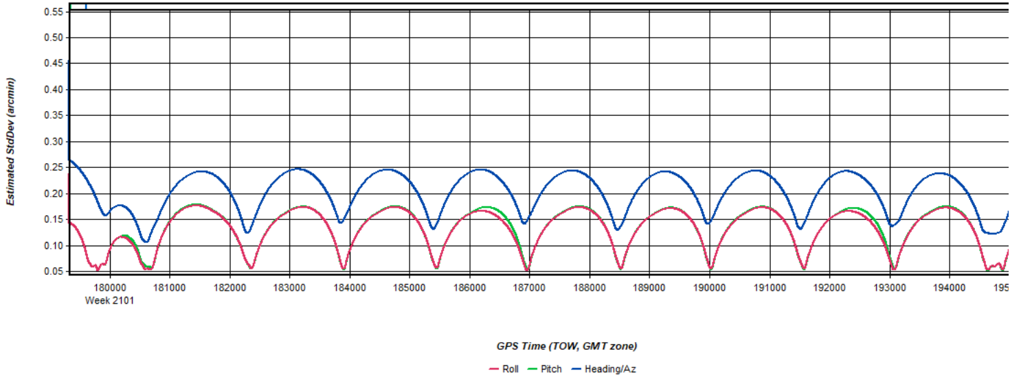
Figure 10: 20200414014741_17 [Smoothed TC Combined] - Estimated Attitude Accuracy Plot
