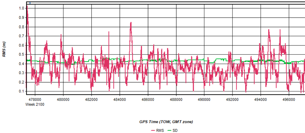
Figure 16: 20200410123525_15 [Smoothed TC Combined] - C/A Code Residual RMS Plot
