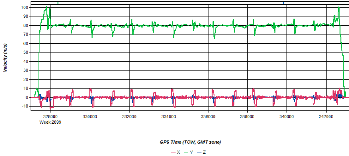
Figure 14: 20200401184852_5 [Smoothed TC Combined] - Body Frame Velocity Plot
