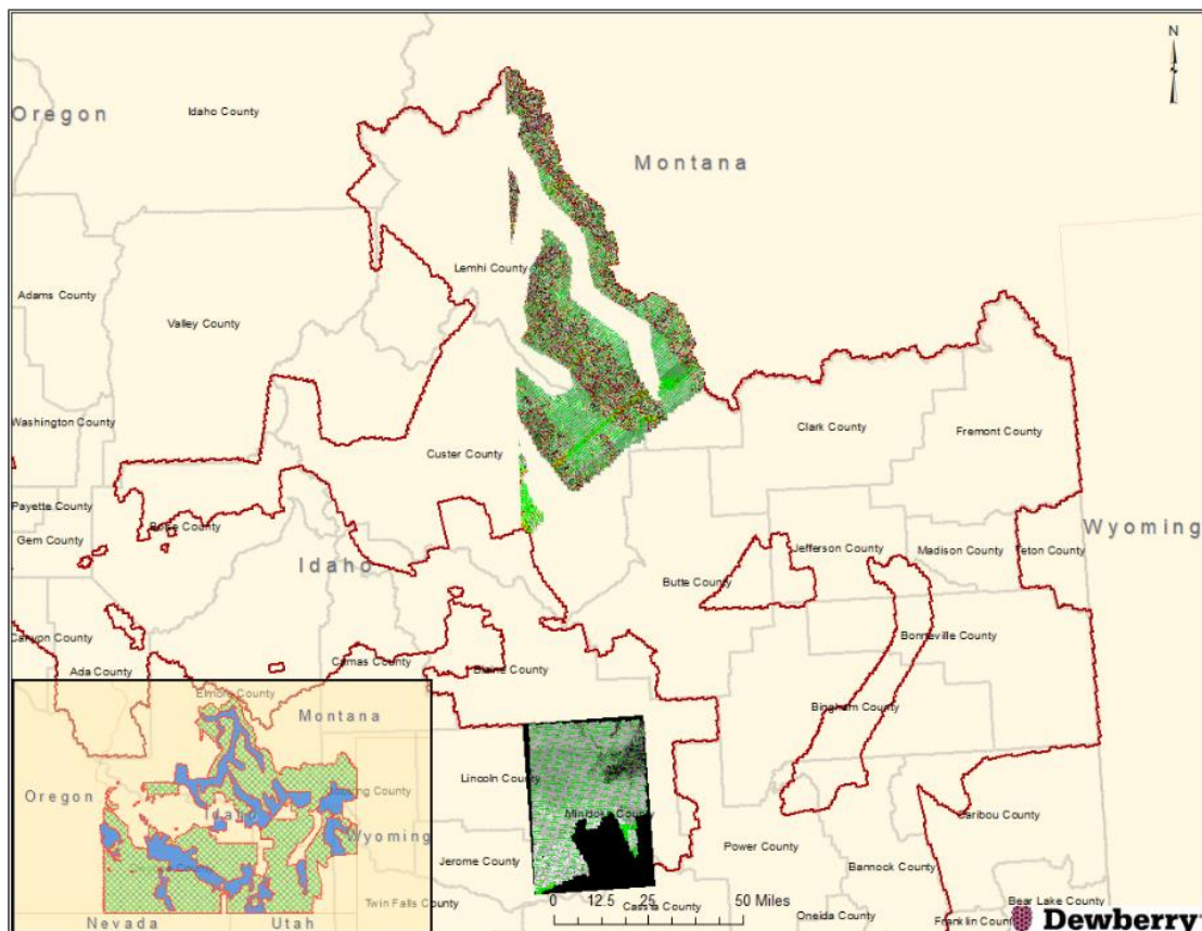
Figure 5. Swath Separation Images (SSIs) generated for WUID 300075.
