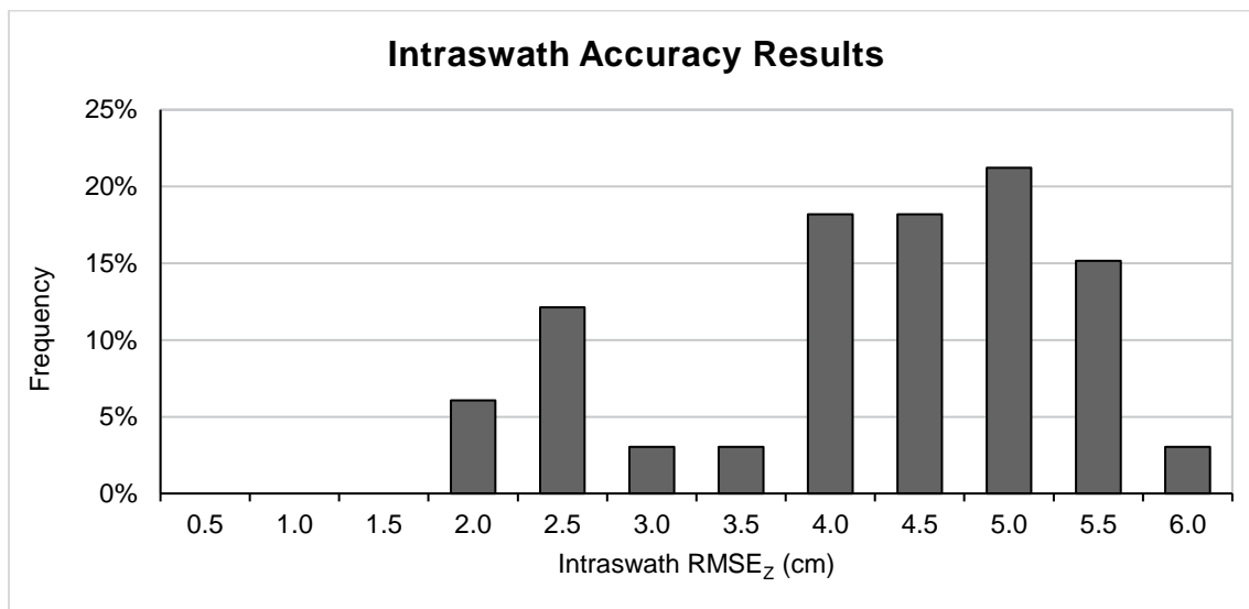
Figure 9. Example test polygon for intraswath testing, and its results
