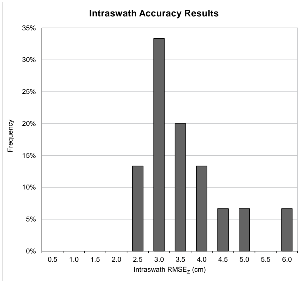
Figure 10. Frequency distribution of intraswath RMSD z results for WUID 300187.
