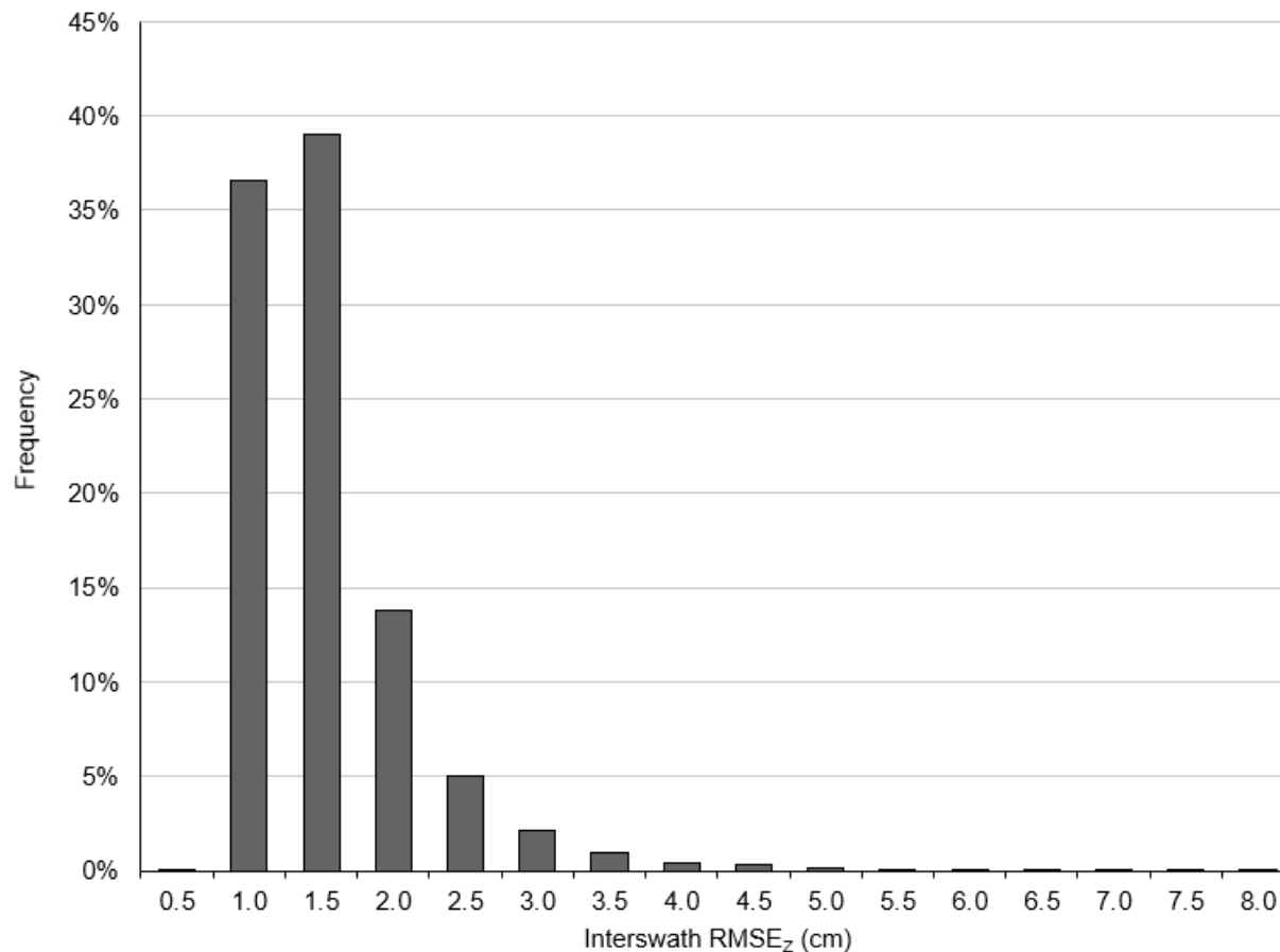
Figure 7. Frequency distribution of interswath RMSDz results for WUID 300189.
