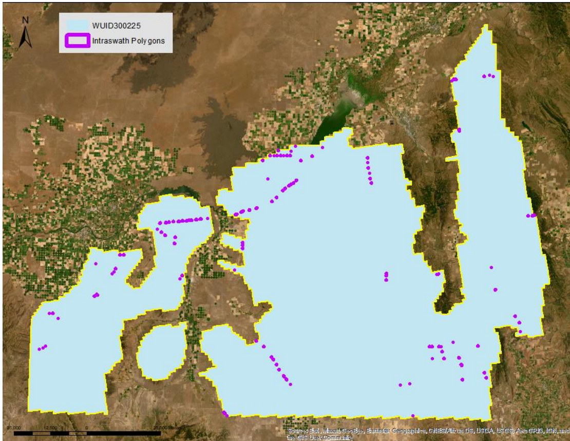
Figure 7. Intraswath polygons used to test intraswath vertical accuracy
