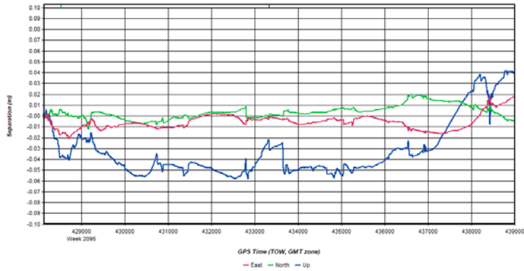
Figure 4: HicksDome_20200305_225309 [Smoothed TC Combined] - Forward/Reverse or Combined Separation Plot
