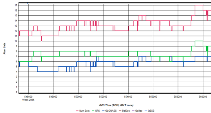
Figure 3: HicksDome_20200307_072436 [Smoothed TC Combined] - Number of Satellites Line Plot
