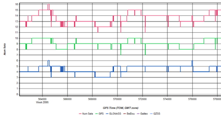
Figure 3: HicksDome_20200307_120639 [Smoothed TC Combined] - Number of Satellites Line Plot
