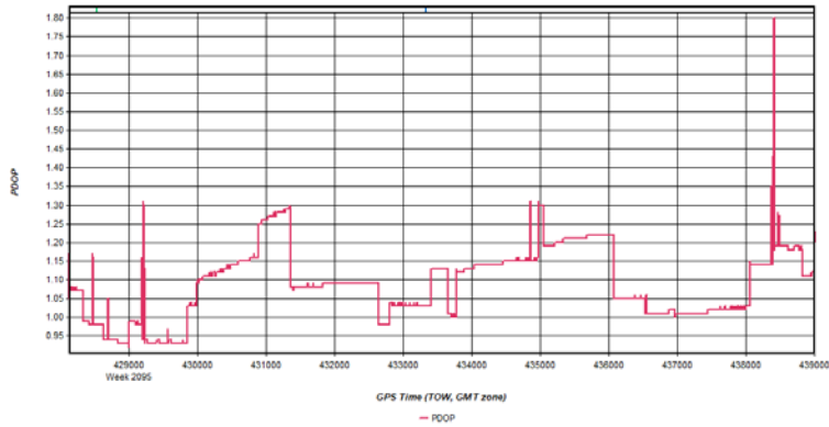
Figure 5: HicksDome_20200305_225309 [Smoothed TC Combined] - PDOP Plot
