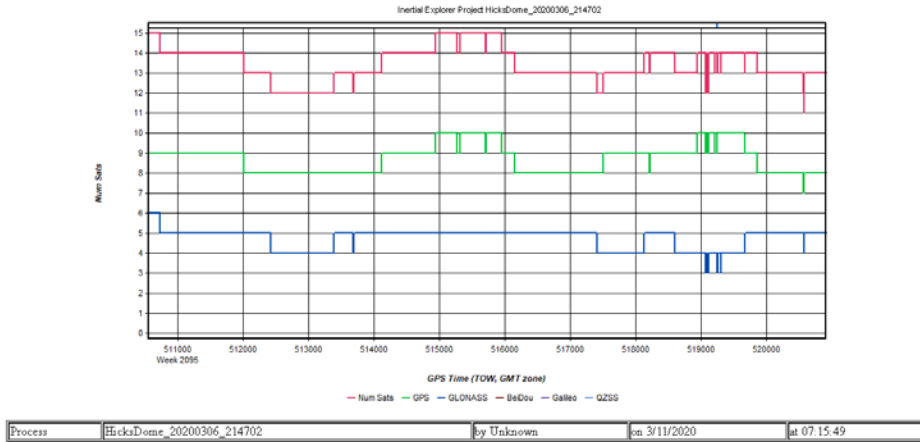
Figure 4: HicksDome_20200306_214702 [Smoothed TC Combined] - Forward/Reverse or Combined Separation Plot
