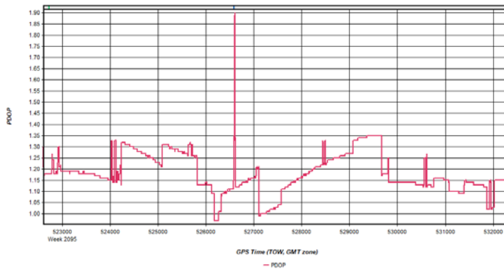
Figure 5: HicksDome_20200307_010807 [Smoothed TC Combined] - PDOP Plot
