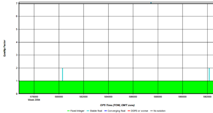
Figure 2: HicksDome_20200229_161043 [Smoothed TC Combined] - Quality Factor Plot
