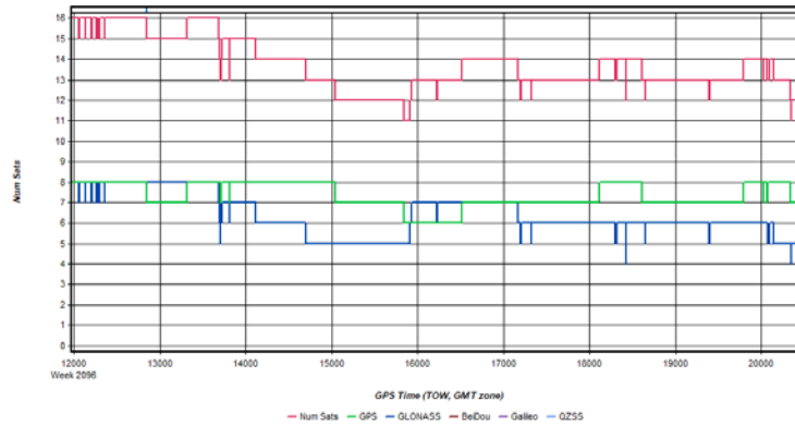
Figure 3: HicksDome_20200308_031434 [Smoothed TC Combined] - Number of Satellites Line Plot
