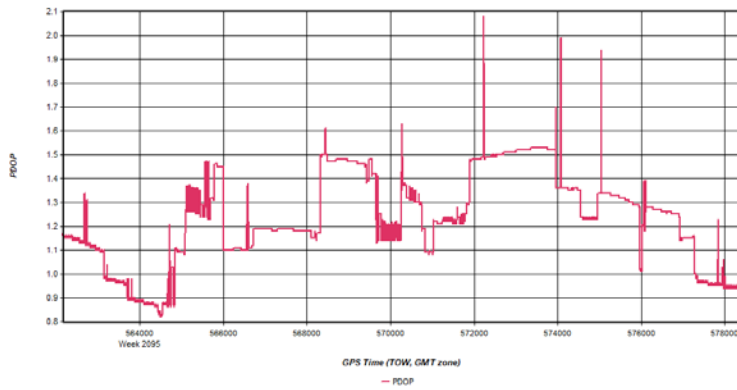
Figure 5: HicksDome_20200307_120639 [Smoothed TC Combined] - PDOP Plot
