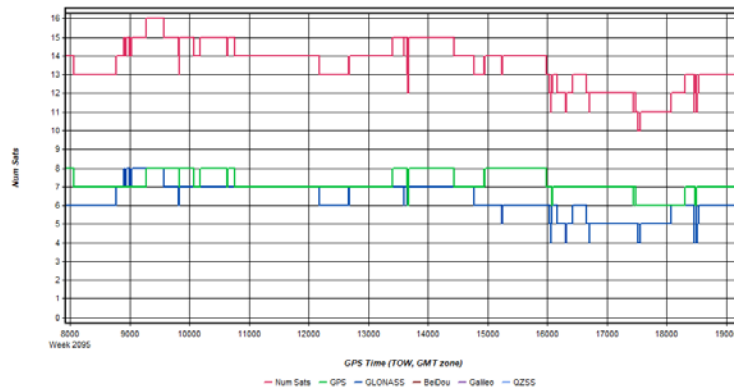
Figure 3: HicksDome_20200301_020914 [Smoothed TC Combined] - Number of Satellites Line Plot
