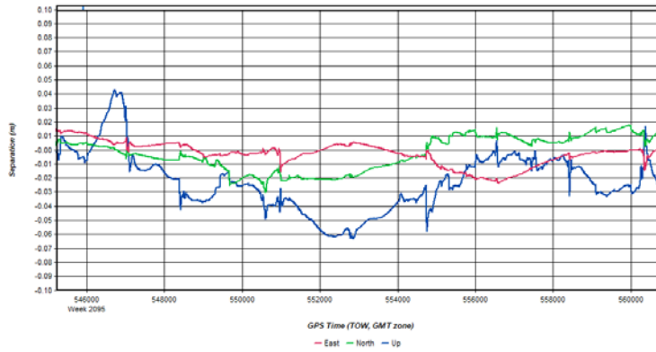
Figure 4: HicksDome_20200307_072436 [Smoothed TC Combined] - Forward/Reverse or Combined Separation Plot
