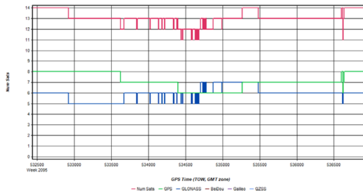
Figure 3: HicksDome_20200307_010807pt2 [Smoothed TC Combined] - Number of Satellites Line Plot
