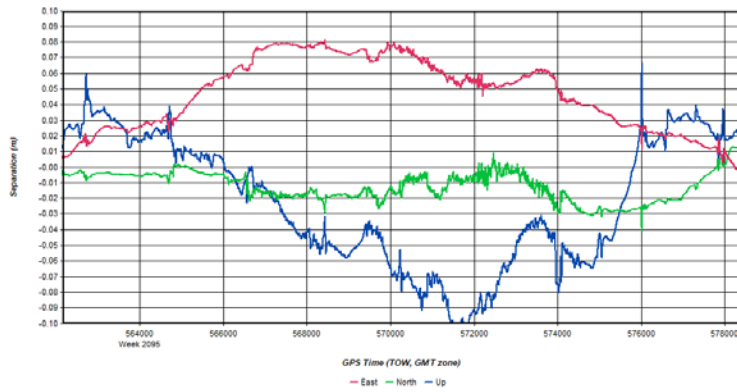
Figure 4: HicksDome_20200307_120639 [Smoothed TC Combined] - Forward/Reverse or Combined Separation Plot
