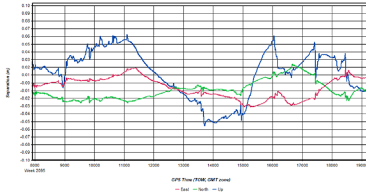
Figure 4: HicksDome_20200301_020914 [Smoothed TC Combined] - Forward/Reverse or Combined Separation Plot
