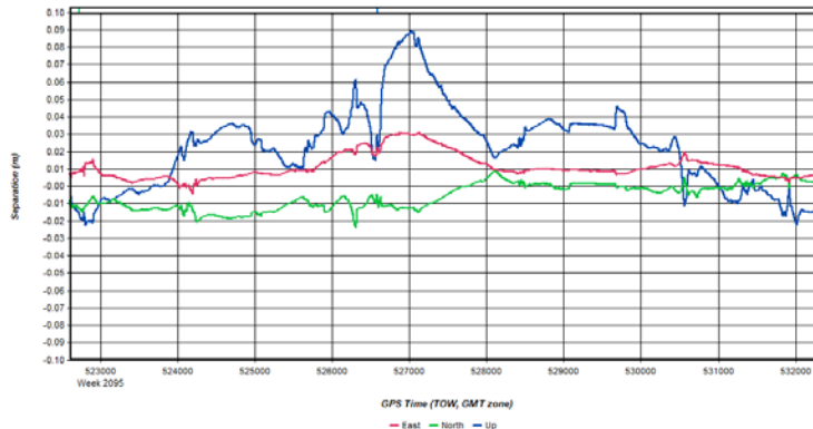
Figure 4: HicksDome_20200307_010807 [Smoothed TC Combined] - Forward/Reverse or Combined Separation Plot
