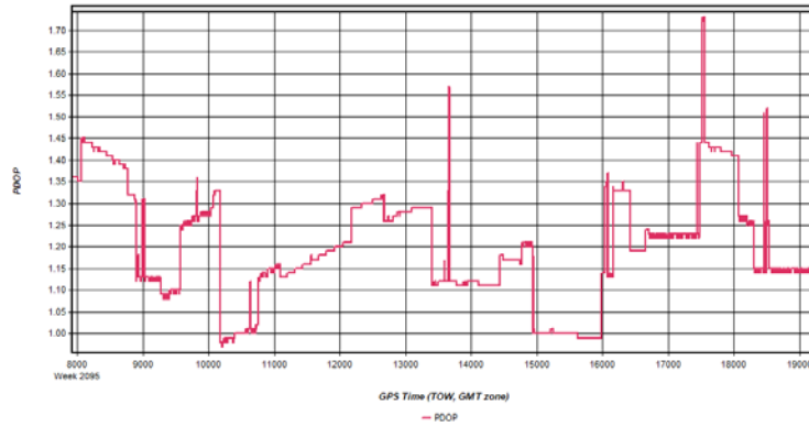
Figure 5: HicksDome_20200301_020914 [Smoothed TC Combined] - PDOP Plot
