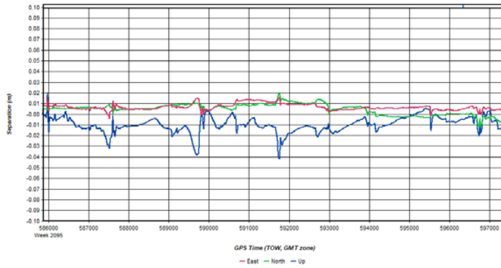
Figure 4: HicksDome_20200307_184217 [Smoothed TC Combined] - Forward/Reverse or Combined Separation Plot
