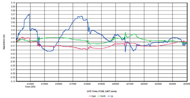
Figure 3: HicksDome_20200305_184142 [Smoothed TC Combined] - Forward/Reverse or Combined Separation Plot
