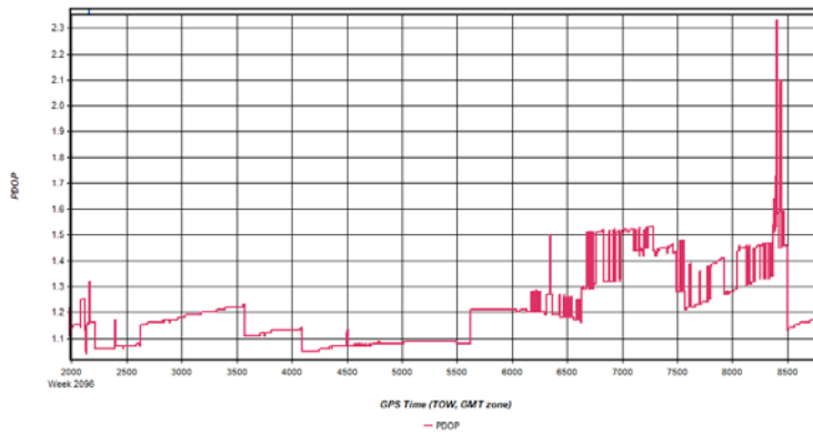
Figure 5: HicksDome_20200308_003052 [Smoothed TC Combined] - PDOP Plot
