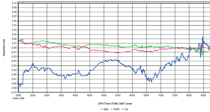
Figure 4: HicksDome_20200308_003052 [Smoothed TC Combined] - Forward/Reverse or Combined Separation Plot
