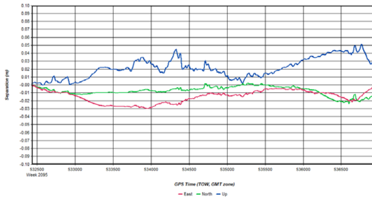
Figure 4: HicksDome_20200307_010807pt2 [Smoothed TC Combined] - Forward/Reverse or Combined Separation Plot
