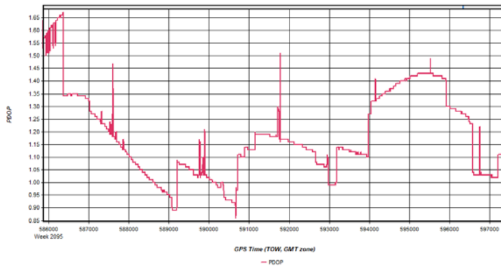
Figure 5: HicksDome_20200307_184217 [Smoothed TC Combined] - PDOP Plot
