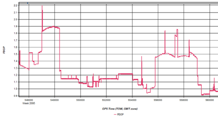
Figure 5: HicksDome_20200307_072436 [Smoothed TC Combined] - PDOP Plot
