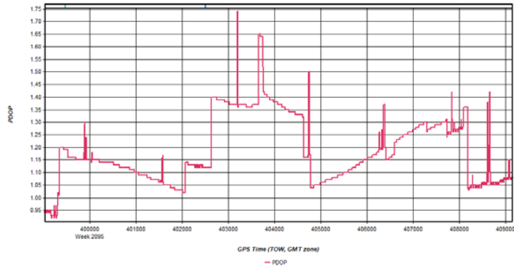
Figure 5: HicksDome_20200305_144800 [Smoothed TC Combined] - PDOP Plot
