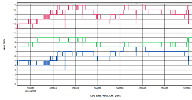
Figure 3: HicksDome_20200229_161043 [Smoothed TC Combined] - Number of Satellites Line Plot
