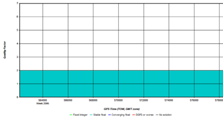
Figure 2: HicksDome_20200307_120639 [Smoothed TC Combined] - Quality Factor Plot
