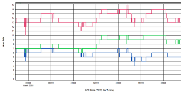
Figure 3: HicksDome_20200301_093540 [Smoothed TC Combined] - Number of Satellites Line Plot
