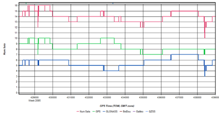
Figure 3: HicksDome_20200305_225309 [Smoothed TC Combined] - Number of Satellites Line Plot
