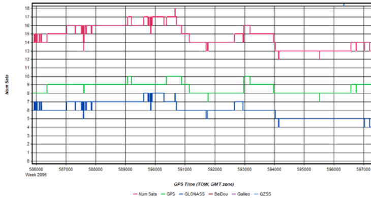
Figure 3: HicksDome_20200307_184217 [Smoothed TC Combined] - Number of Satellites Line Plot
