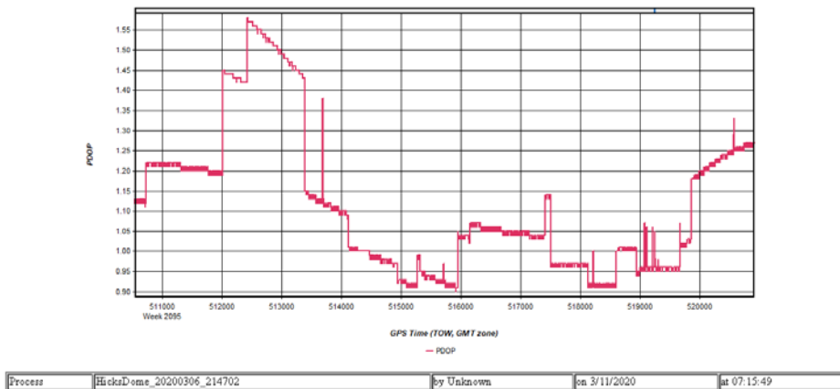
Figure 5: HicksDome_20200306_214702 [Smoothed TC Combined] - PDOP Plot
