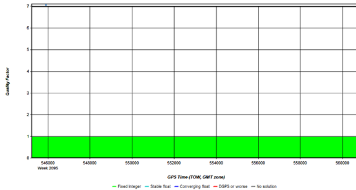
Figure 2: HicksDome_20200307_072436 [Smoothed TC Combined] - Quality Factor Plot
