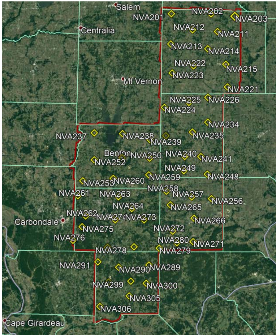
Figure 14 – Location of Block_1_HicksDome_FluorsparDistrict LiDAR NVA Checkpoints
