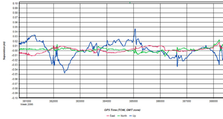
Figure 4: HicksDome_20200305_094110 [Smoothed TC Combined] - Forward/Reverse or Combined Separation Plot
