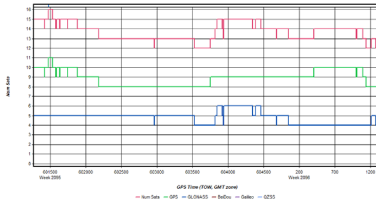
Figure 3: HicksDome_20200307_225857 [Smoothed TC Combined] - Number of Satellites Line Plot
