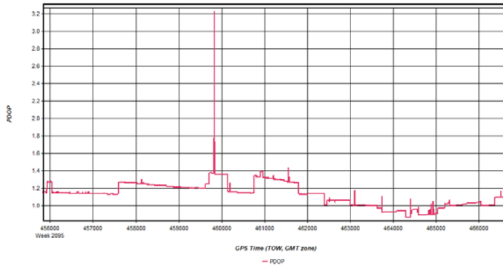
Figure 5: HicksDome_20200306_063204 [Smoothed TC Combined] - PDOP Plot
