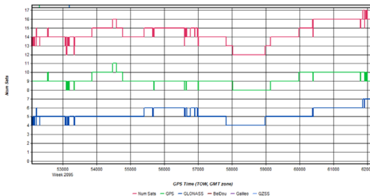
Figure 3: HicksDome_20200301_142548 [Smoothed TC Combined] - Number of Satellites Line Plot
