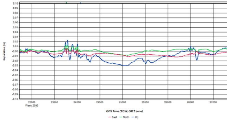
Figure 4: HicksDome_20200301_061551 [Smoothed TC Combined] - Forward/Reverse or Combined Separation Plot
