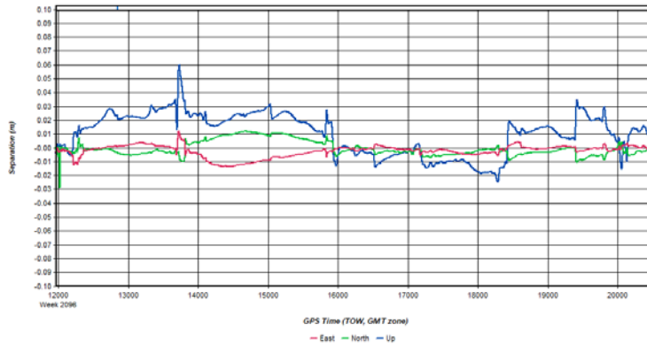
Figure 4: HicksDome_20200308_031434 [Smoothed TC Combined] - Forward/Reverse or Combined Separation Plot
