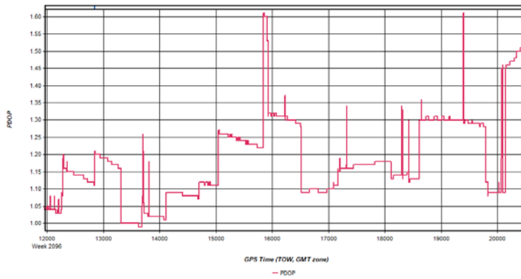
Figure 5: HicksDome_20200308_031434 [Smoothed TC Combined] - PDOP Plot
