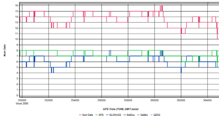
Figure 3: HicksDome_20200305_010608 [Smoothed TC Combined] - Number of Satellites Line Plot
