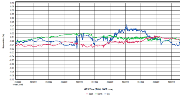
Figure 4: HicksDome_20200306_063204 [Smoothed TC Combined] - Forward/Reverse or Combined Separation Plot
