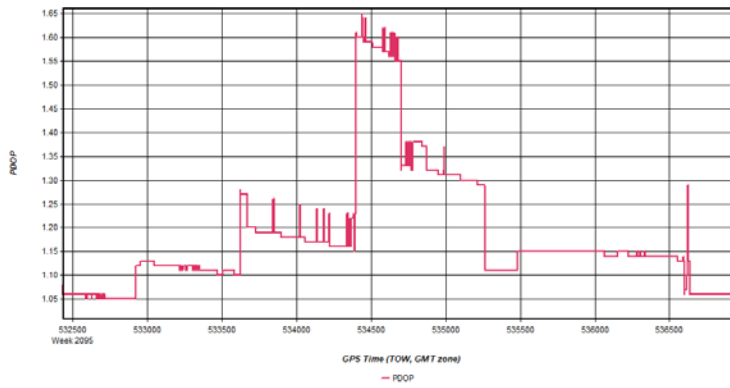
Figure 5: HicksDome_20200307_010807pt2 [Smoothed TC Combined] - PDOP Plot
