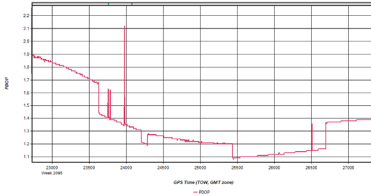
Figure 5: HicksDome_20200301_061551 [Smoothed TC Combined] - PDOP Plot
