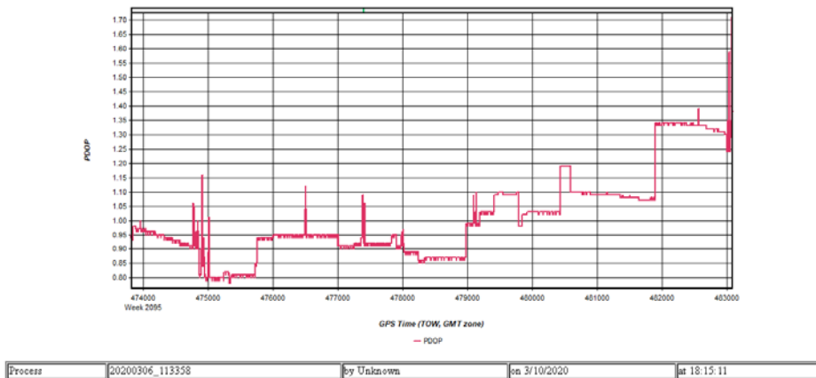
Figure 5: 20200306_113358 [Smoothed TC Combined] - PDOP Plot
