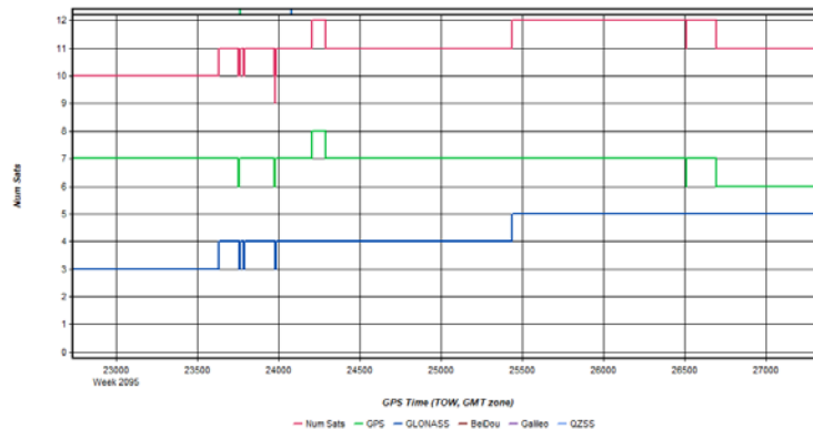
Figure 3: HicksDome_20200301_061551 [Smoothed TC Combined] - Number of Satellites Line Plot
