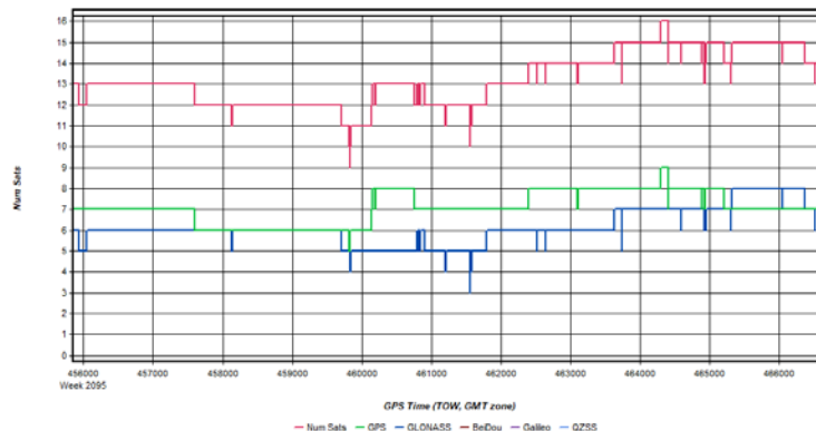
Figure 3: HicksDome_20200306_063204 [Smoothed TC Combined] - Number of Satellites Line Plot
