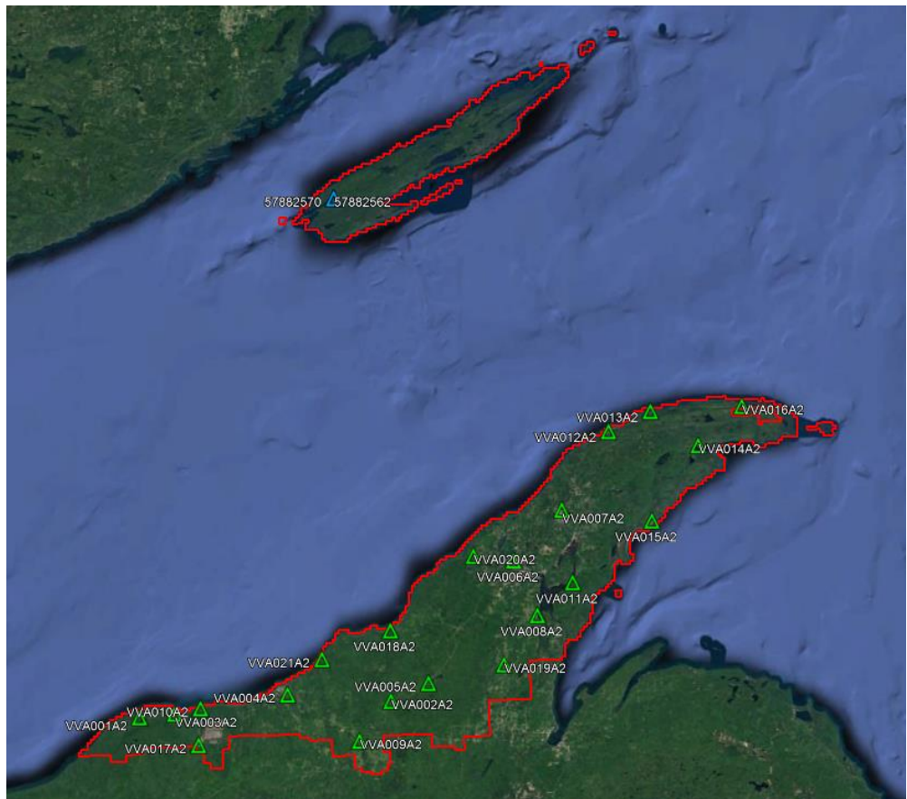
Figure 6: Vegetated Check Point Distribution (State of MI control in Blue)
