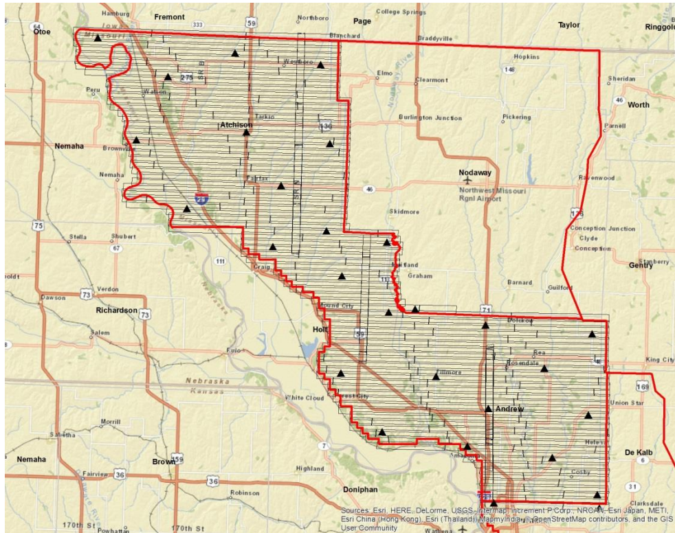
Figure 2 Atchison-Holt-Andrew Co. Swath LiDAR Control
