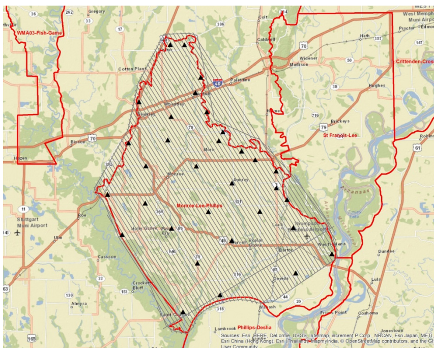
Figure 2 Monroe-Lee-Phillips Co. Swath LiDAR Control
