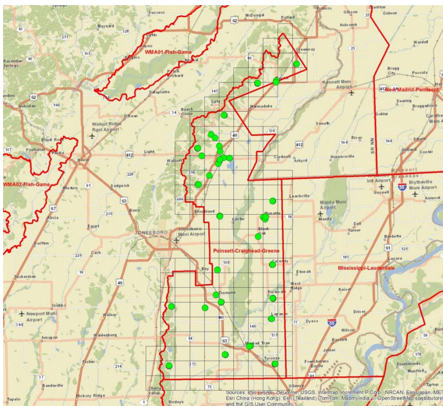
Figure 3 Poinsett-Craighead-Greene Co. LiDAR QC Check
