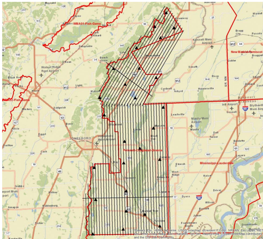
Figure 2 Poinsett-Craighead-Greene Co. Swath LiDAR Control
