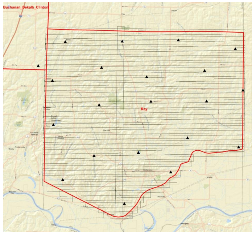
Figure 2 Ray Co. Swath LiDAR Control
