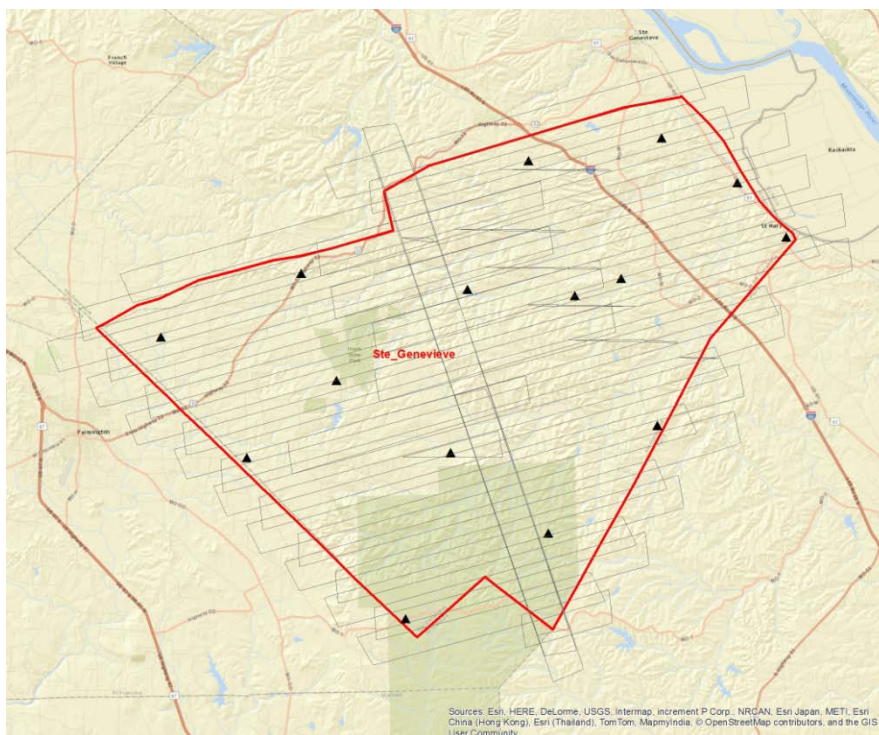
Figure 2 Ste Genevieve Co. Swath LiDAR Control
