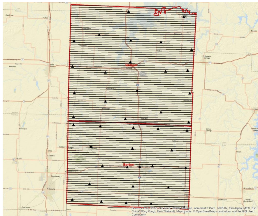
Figure 2 Vernon-Barton Co. Swath LiDAR Control
