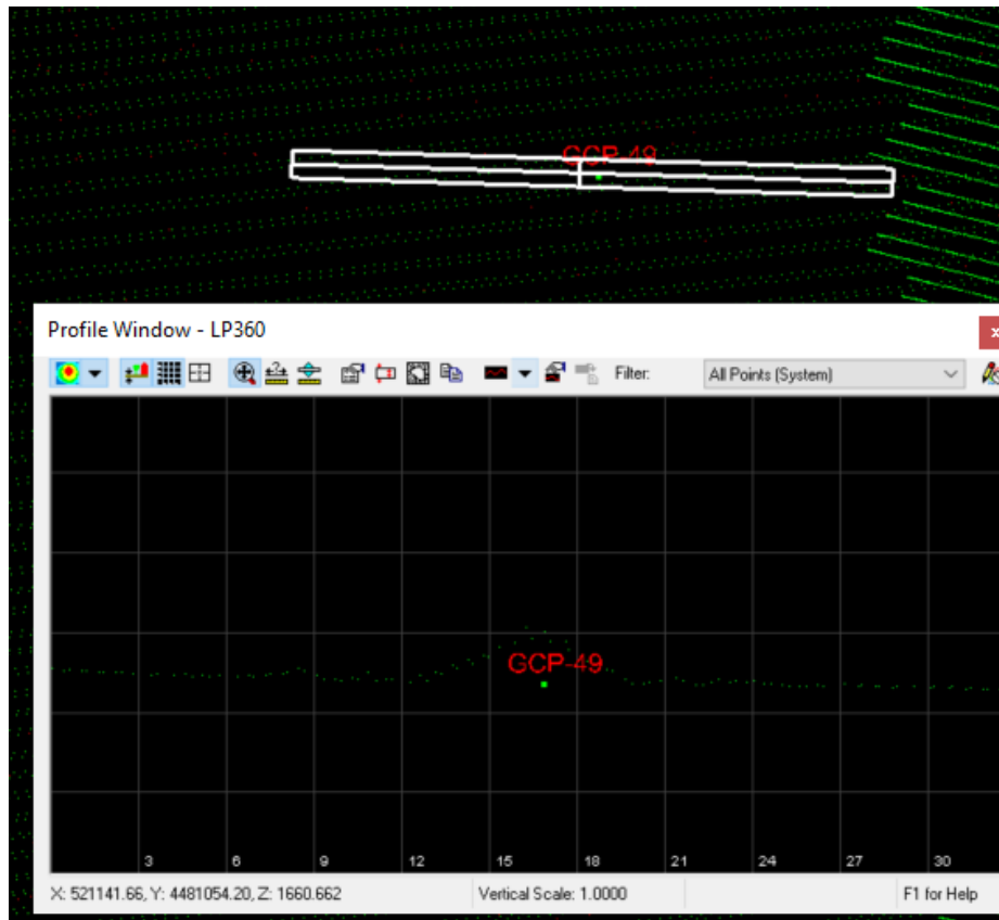
Figure 5. Ground Control Point 49, shown in green, is located underneath some vegetation. This point was removed calibrated swath vertical accuracy testing because above ground features have not been separated from the ground classification yet.
