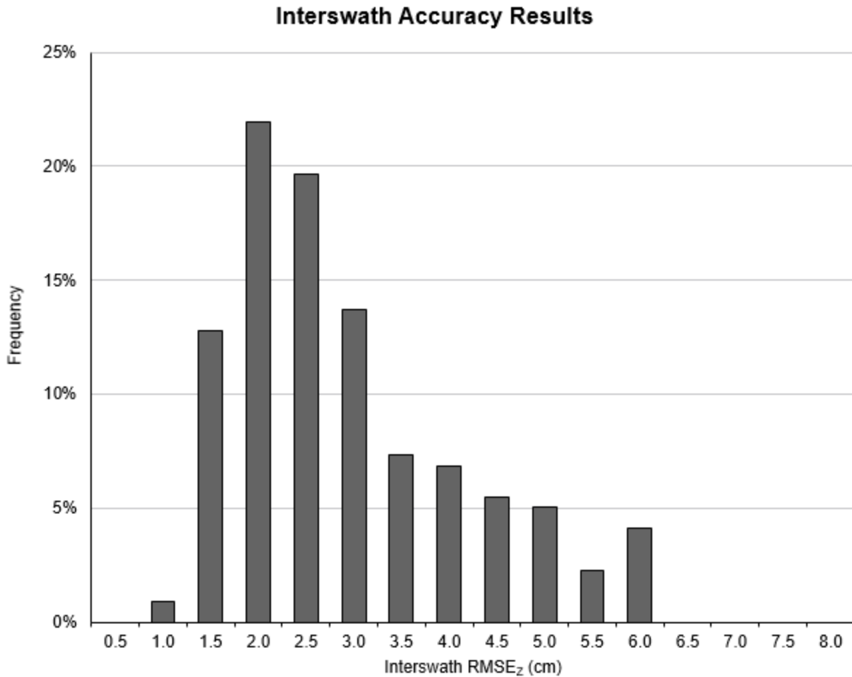
Figure 11. Frequency distribution of interswath RMSDz results for the Nevada NorthWest Elko project.
