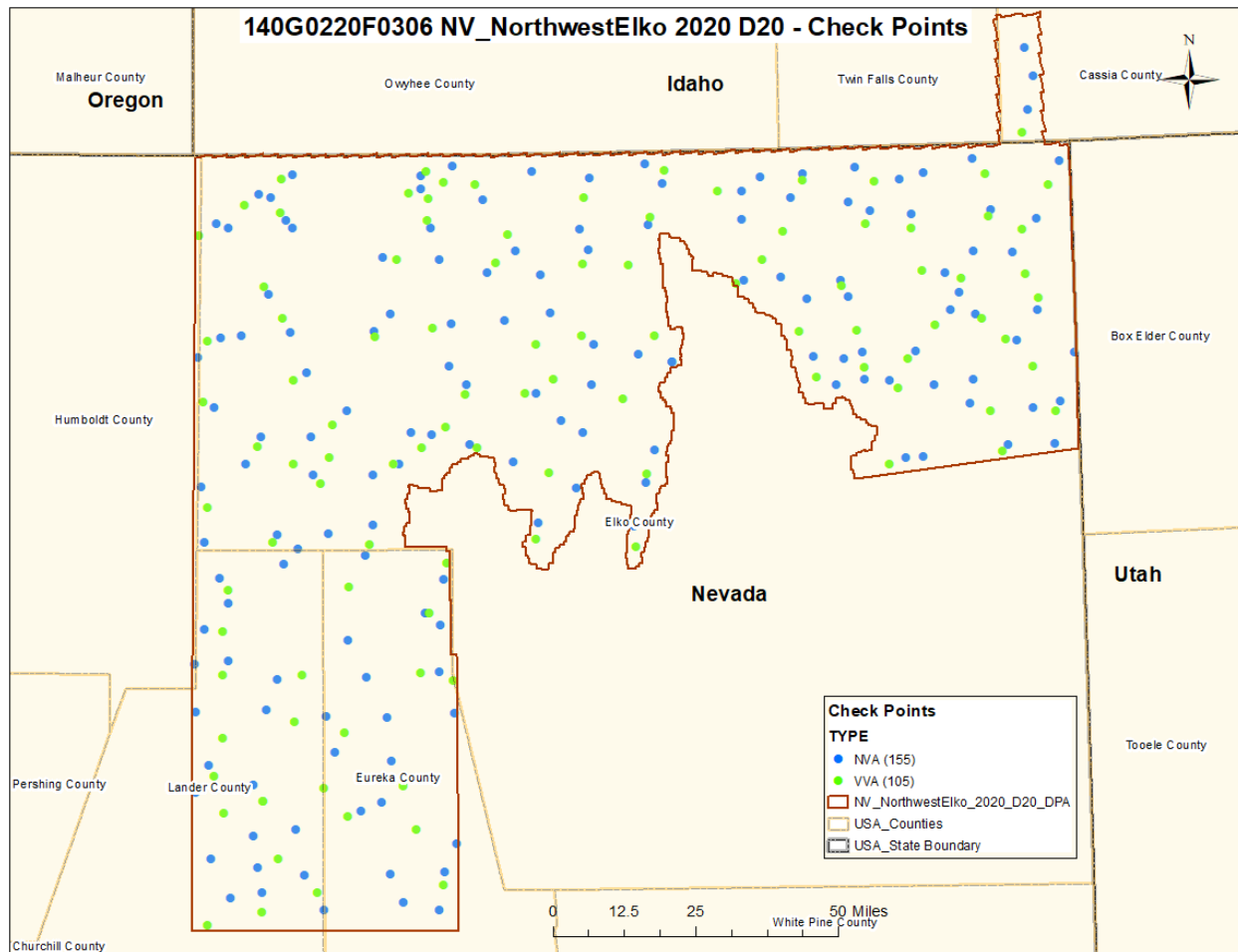
Figure 7. Project map with state plane zones outlined and checkpoints in each state plane zone displayed.
