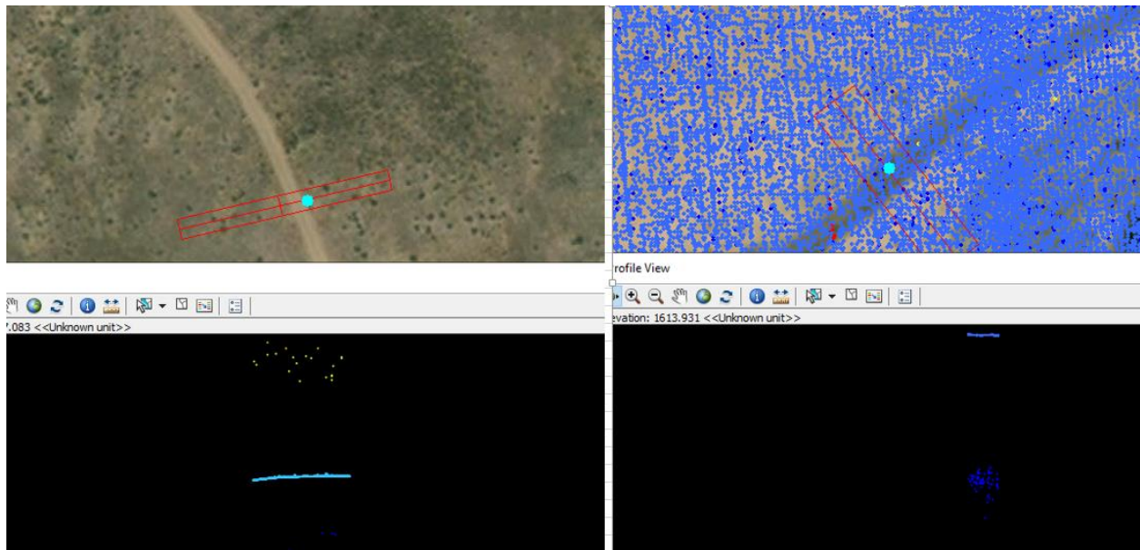
Figure 8. Checkpoints NVA-50 and NVA-56, shown as the as teal dots, located with noise. These points were removed from raw swath vertical accuracy testing because artifacts, including noise, have not been separated from the ground classification yet.
