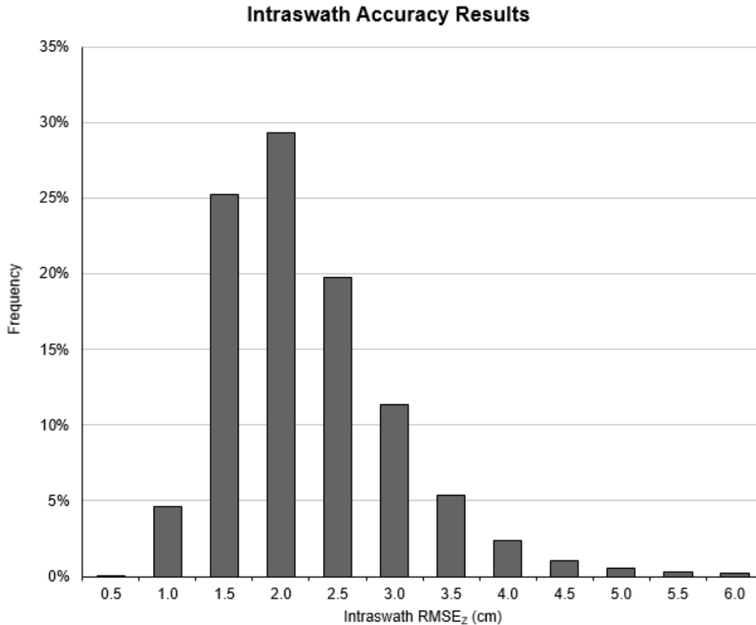
Figure 14. Frequency distribution of intraswath RMSDz results for the Nevada NorthWest Elko project
