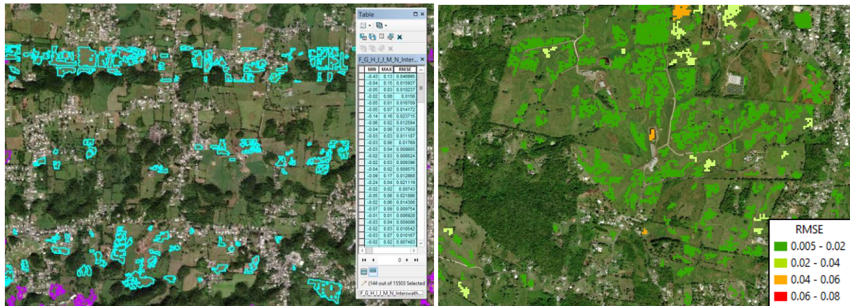
Figure 10. Left: Example interswath polygons and example statistics. Right: Example interswath polygons colored by RMSDz values.
