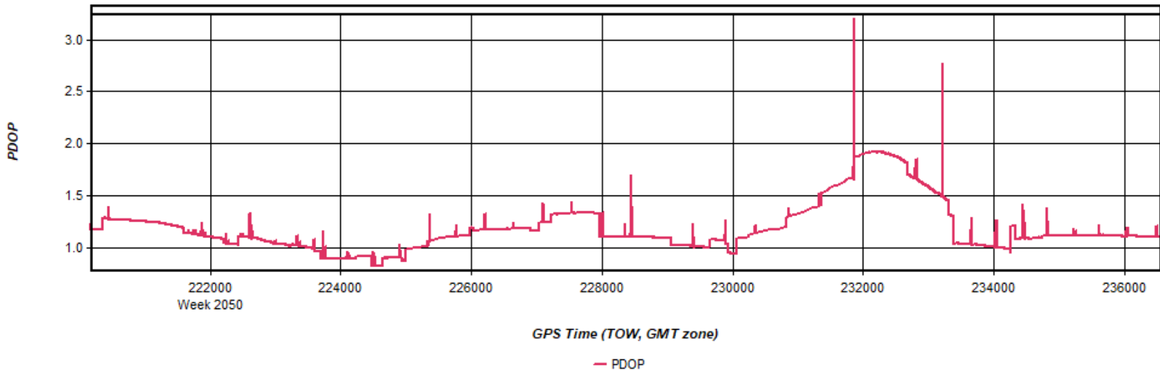
Figure 5: Dewberry_NY_3DEP_20190423_130623 [Smoothed TC Combined] - PDOP Plot
