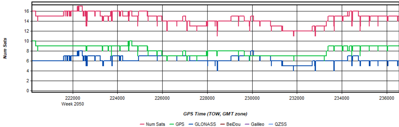
Figure 3: Dewberry_NY_3DEP_20190423_130623 [Smoothed TC Combined] - Number of Satellites Line Plot
