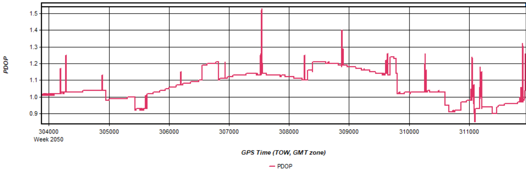
Figure 5: Dewberry_NY_3DEP_20190424_122231 [Smoothed TC Combined] - PDOP Plot
