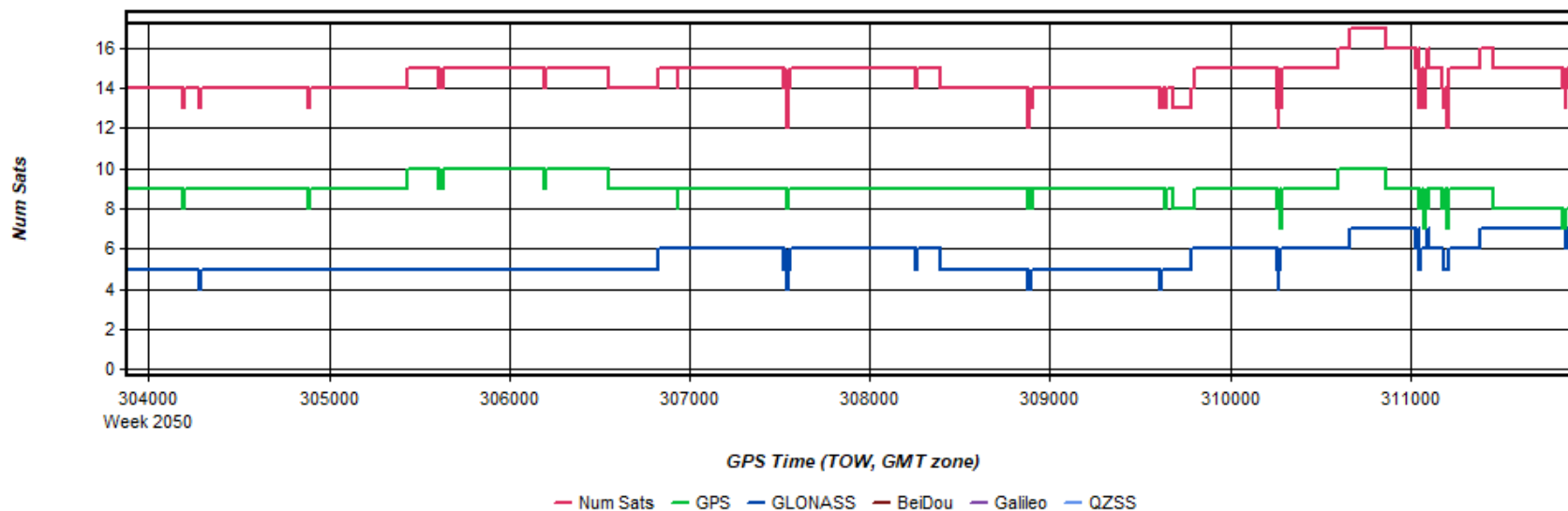
Figure 3: Dewberry_NY_3DEP_20190424_122231 [Smoothed TC Combined] - Number of Satellites Line Plot
