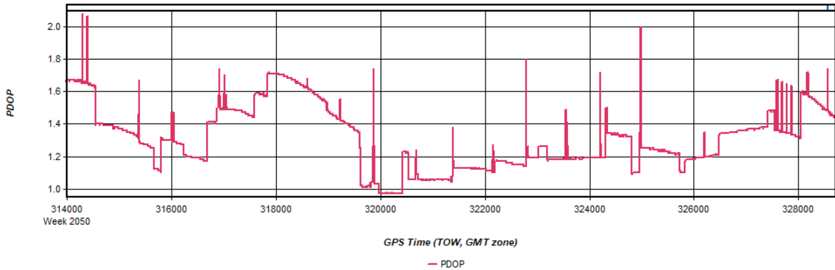
Figure 5: Dewberry_NY_3DEP_20190424_151109 [Smoothed TC Combined] - PDOP Plot
