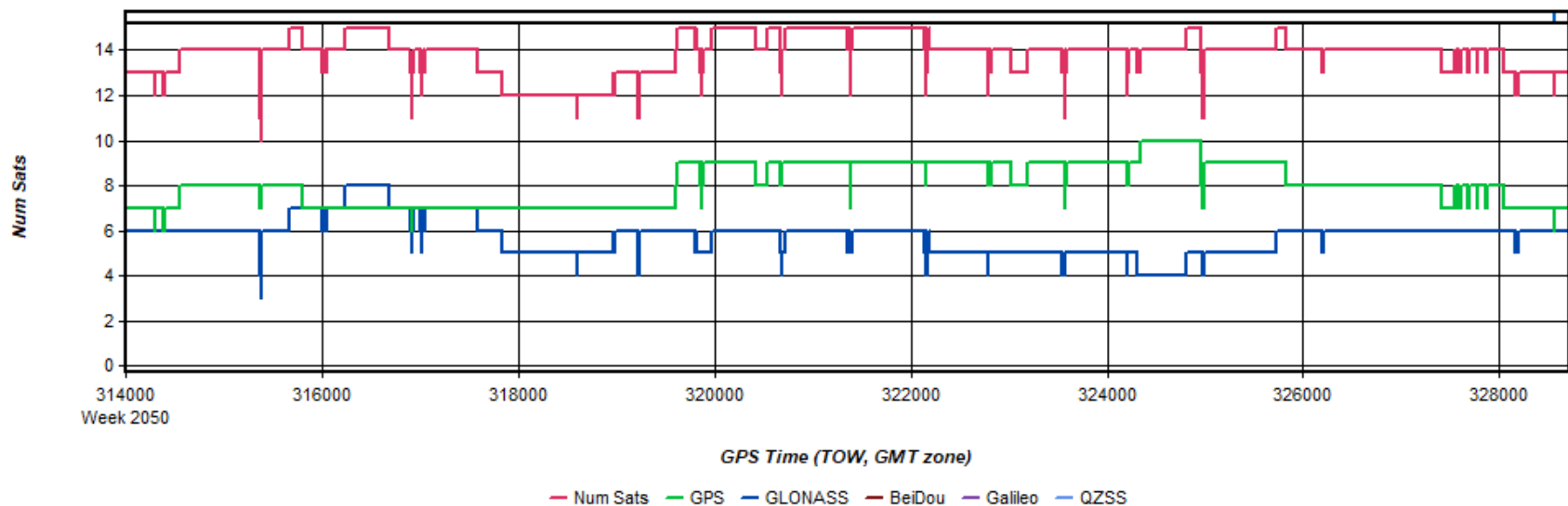
Figure 3: Dewberry_NY_3DEP_20190424_151109 [Smoothed TC Combined] - Number of Satellites Line Plot
