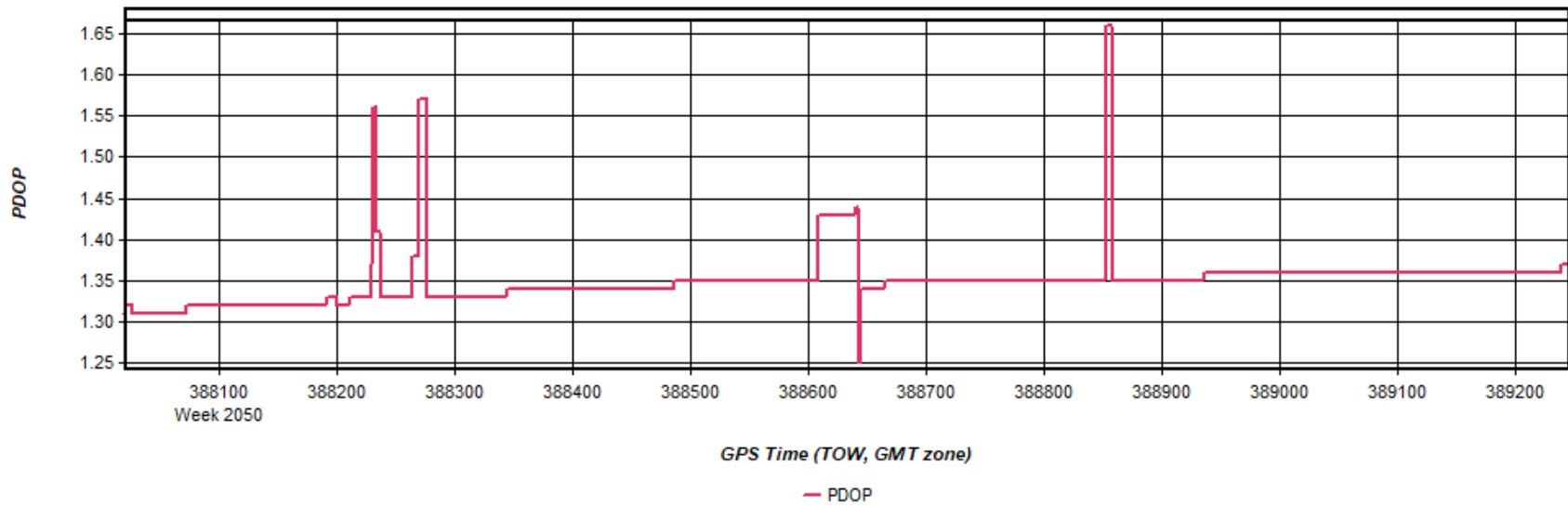
Figure 5: Dewberry_NY_3DEP_20190425_114434 [Smoothed TC Combined] - PDOP Plot
