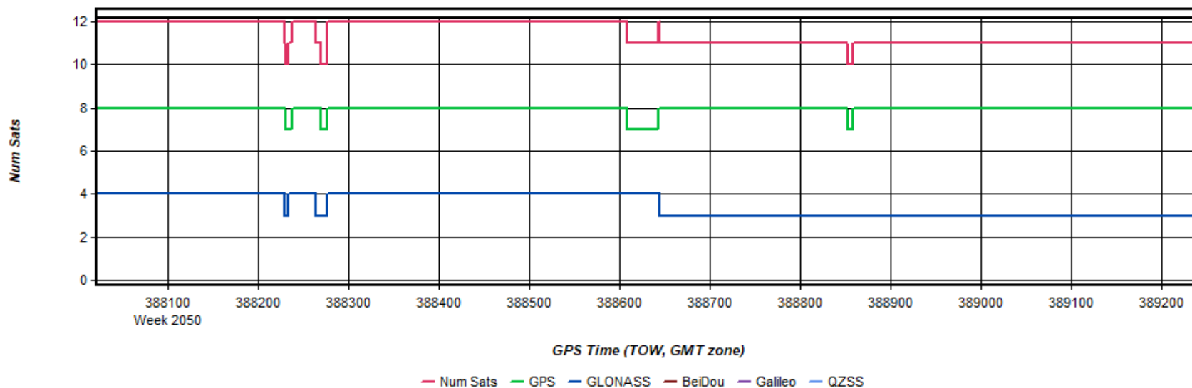
Figure 3: Dewberry_NY_3DEP_20190425_114434 [Smoothed TC Combined] - Number of Satellites Line Plot
