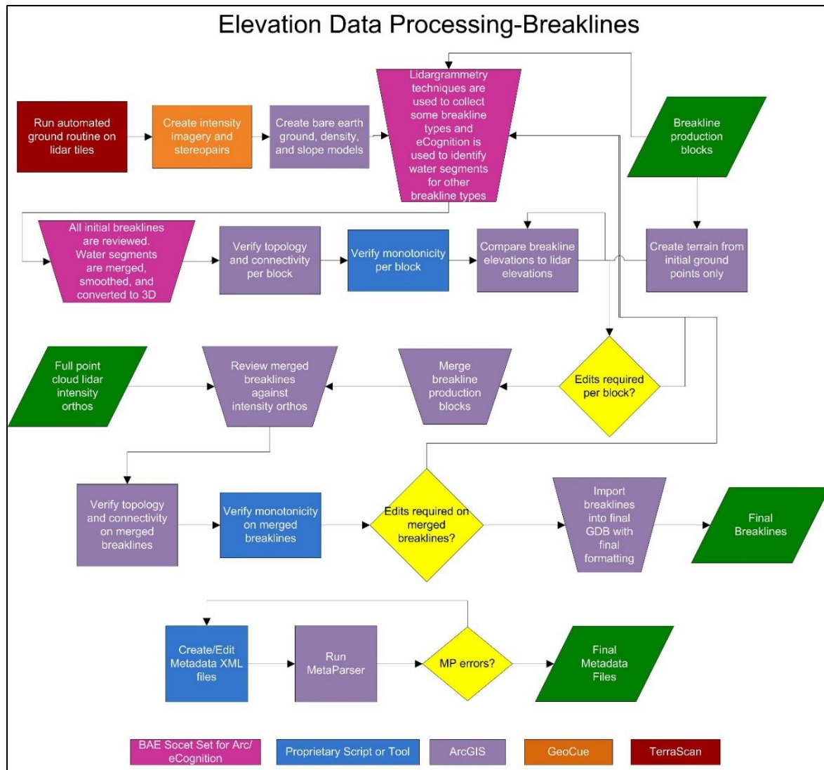
Figure 20-Breakline QA/QC workflow
