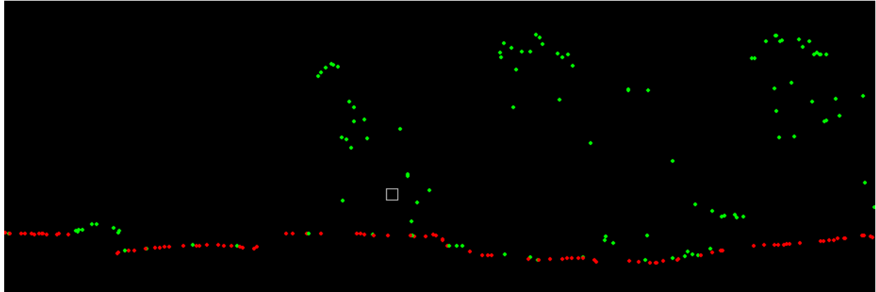
Figure 15 – Forest checkpoint 45-1-2, shown as the white box in the profile, is located in a forest stand. This checkpoint was removed from all vertical accuracy calculations due to its probable unreliability.
