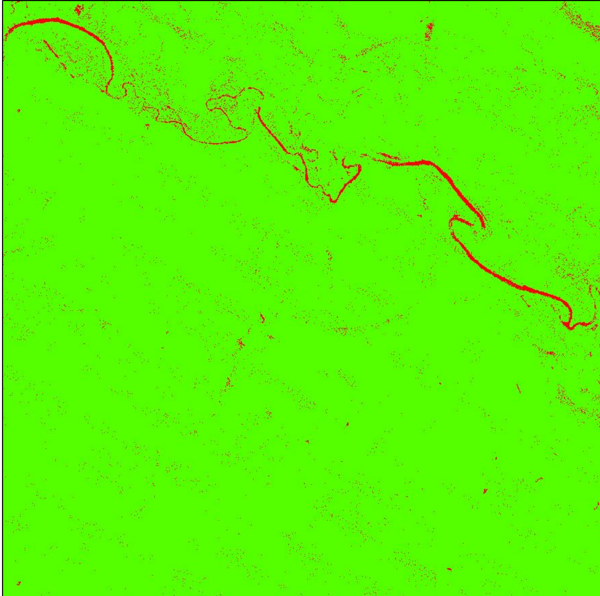
Figure 9 Spatial Distribution. All cells (2*NPS cellsize) containing at least one lidar point are colored green. Cells that do not contain a lidar point, including water bodies which are acceptable NoData area, are colored red. Without removing acceptable NoData areas due to water, 98.7% of cells contain at least one lidar point.
