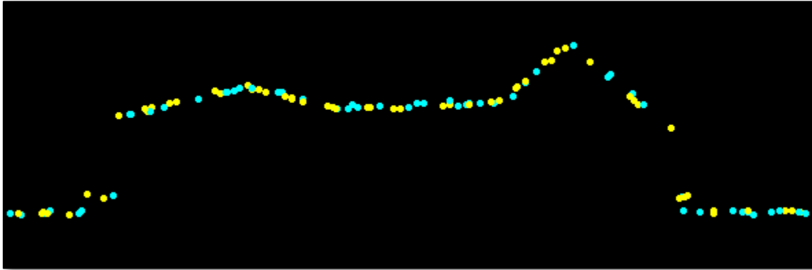
Figure 7– Horizontal Alignment. Two separate flight lines differentiated by color (cyan/yellow) are shown in this profile. There is no visible offset between these two flight lines. No horizontal alignment issues were identified.
