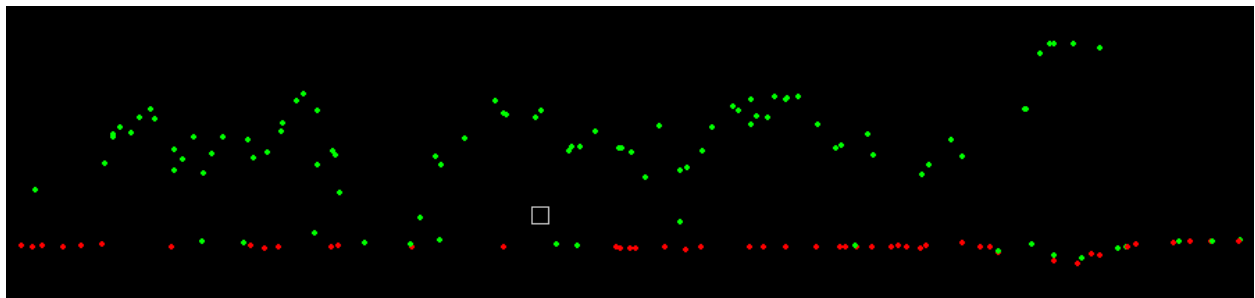
Figure 16 – Forest checkpoint 45-7-7 shown as the white box in the profile, is located in a forest stand. This checkpoint was removed from all vertical accuracy calculations due to its probable unreliability.
