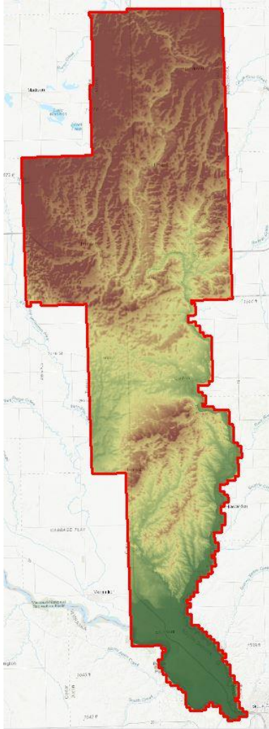
Figure 2: Block 2 Shaded Relief
