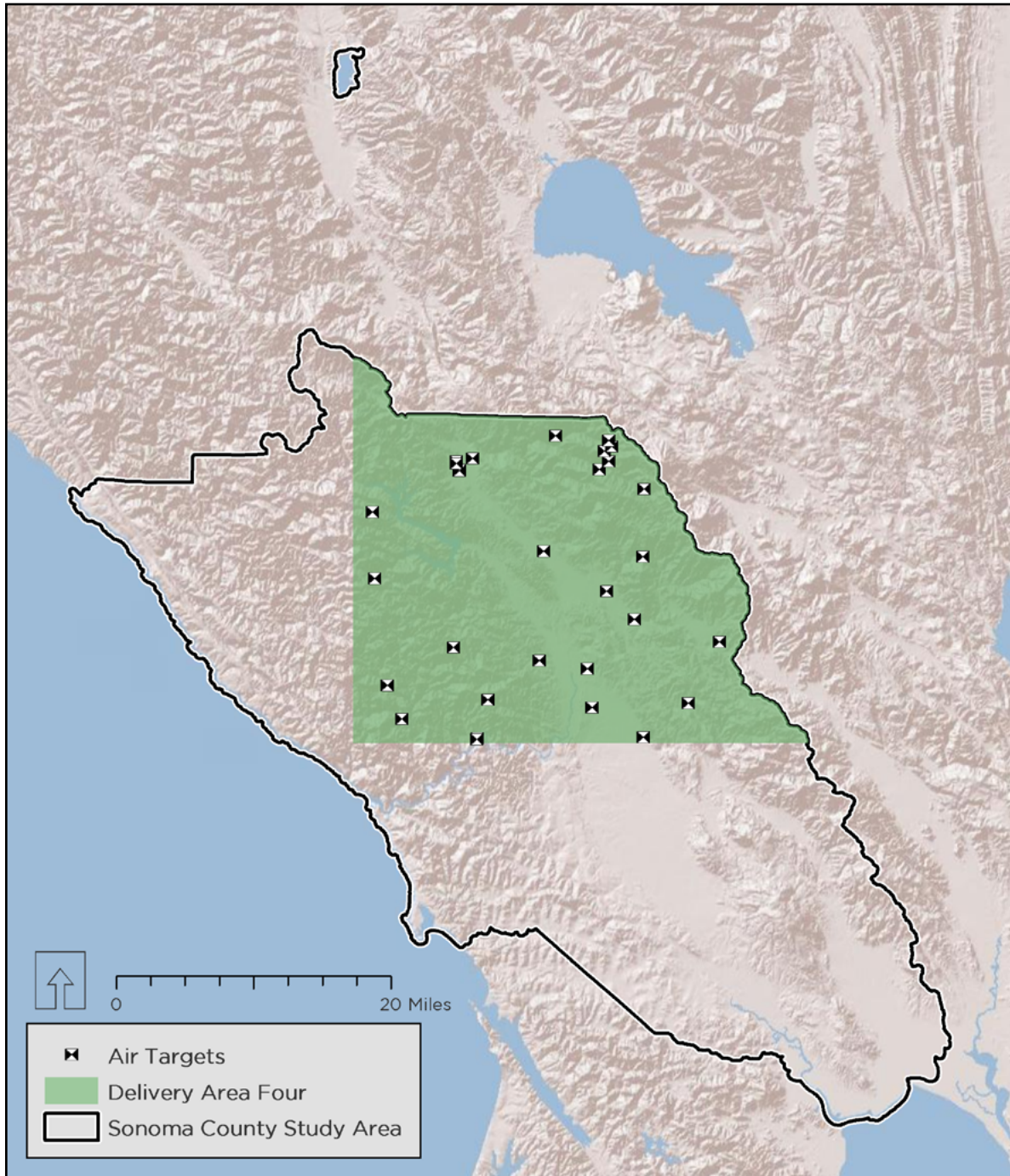
Placement of air targets, permanent and temporary, within Delivery Area Four
