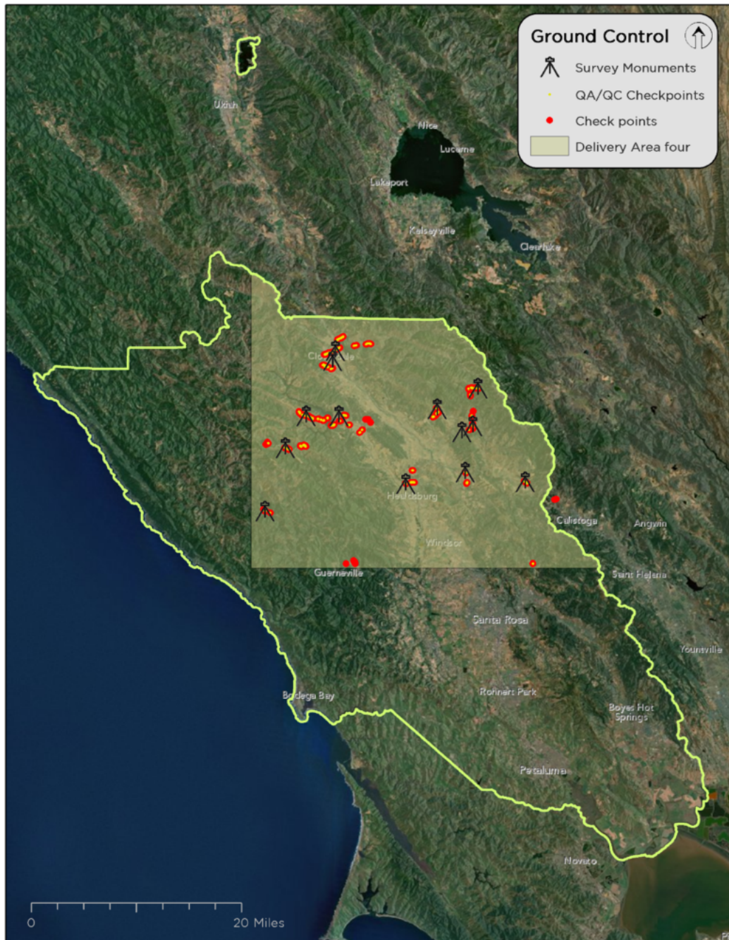
Ground Control and GCP positions for Delivery Area Four.
