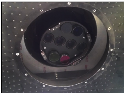
UltraCam Eagle lens configuration as viewed from the Cessna Caravan.
