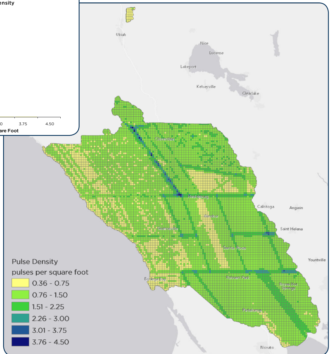
Sonoma County pulse density map and distribution graph.
