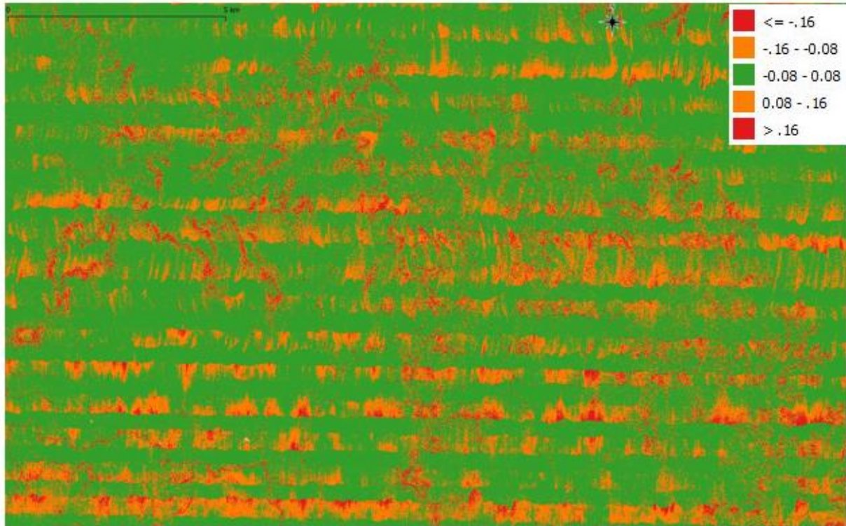
Figure 30 – QC block colored by separation demonstrating uncalibrated accuracy at swath edges (16cm max range).
