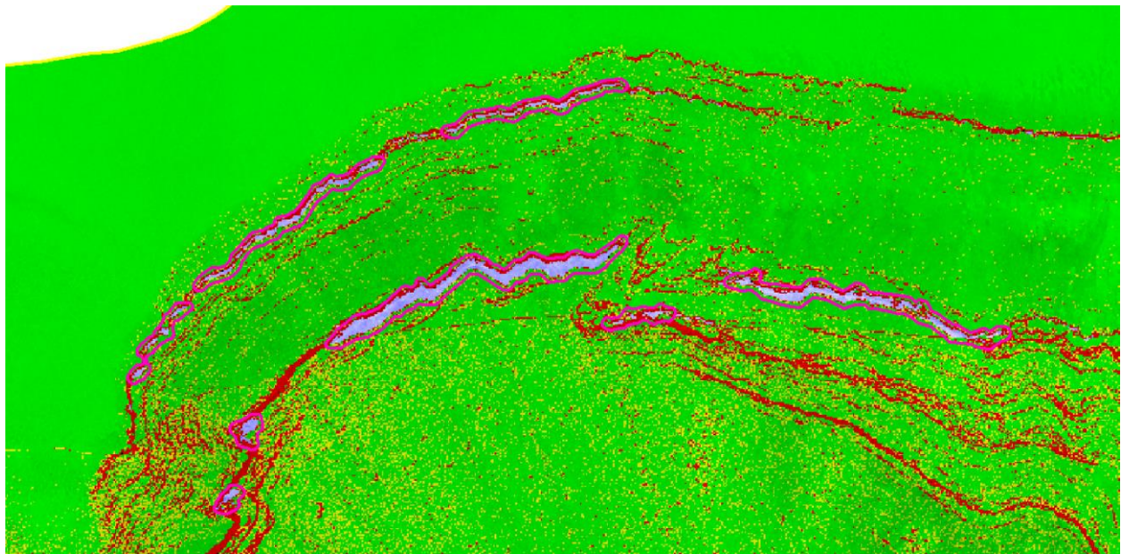
Figure 12. The top image shows a raster colored by the number of overlapping flightlines and the bottom image shows the SSI of the same location. The DPA is shown as the yellow outline (northwest corner of images) and areas of single coverage polygonised by Dewberry are shown as pink outlines. This example is near the DPA, where at least two flightline coverages (blue areas in top image) extend all the way to the DPA. Areas of single coverages (brown areas in top image and delineated with pink polygons in both images) exist in very steep terrain, as narrow bands along cliff faces. These areas appear as red or single coverage in the SSIs. The top raster shows that these areas were correctly acquired with at least two coverages, sometimes even three or more, but laser shadowing may still exist due to the very steep terrain of this WU.
