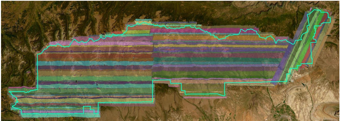
Figure 3. WUID 300243 swaths
