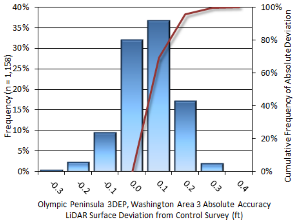
Figure 10: Frequency histogram for LiDAR surface deviation from ground control point values
