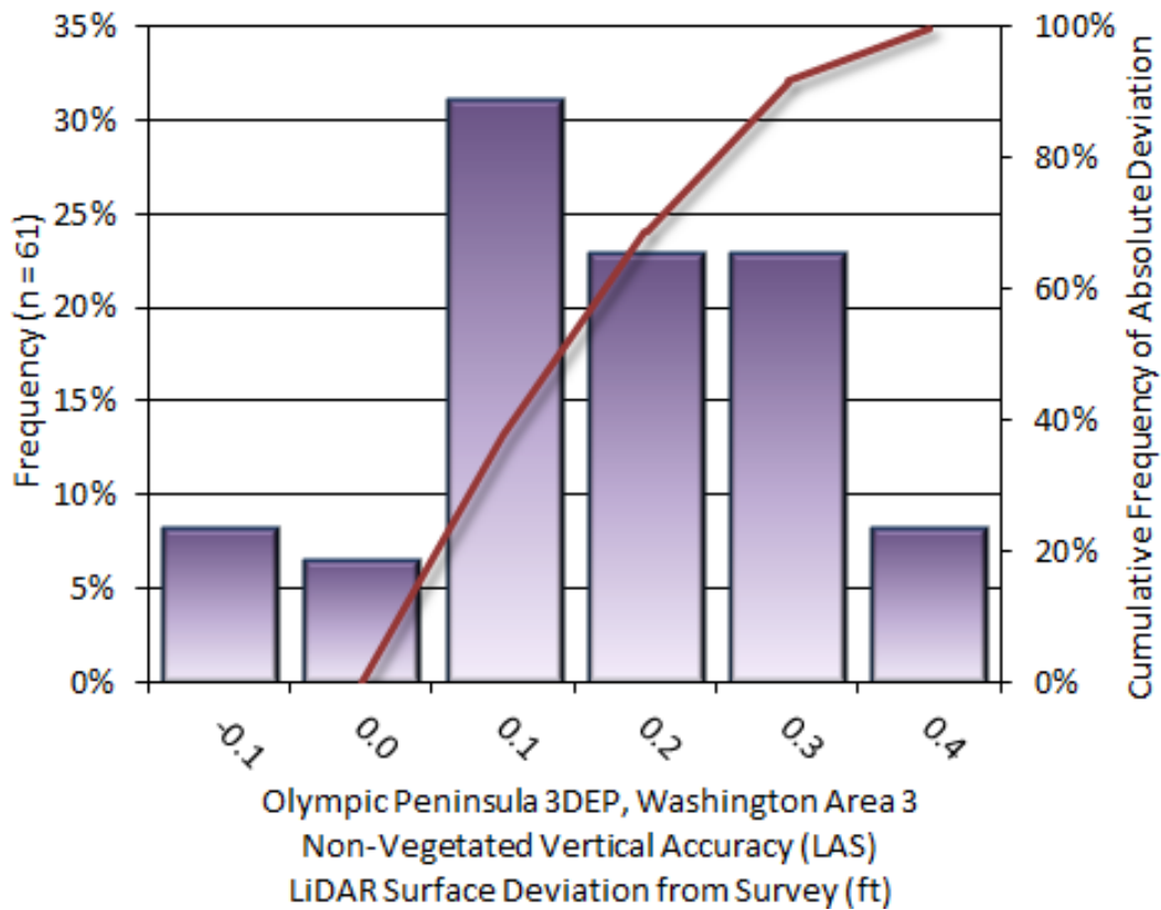
Figure 8: Frequency histogram for LiDAR unclassified point deviation from non-vegetated quality assurance point values
