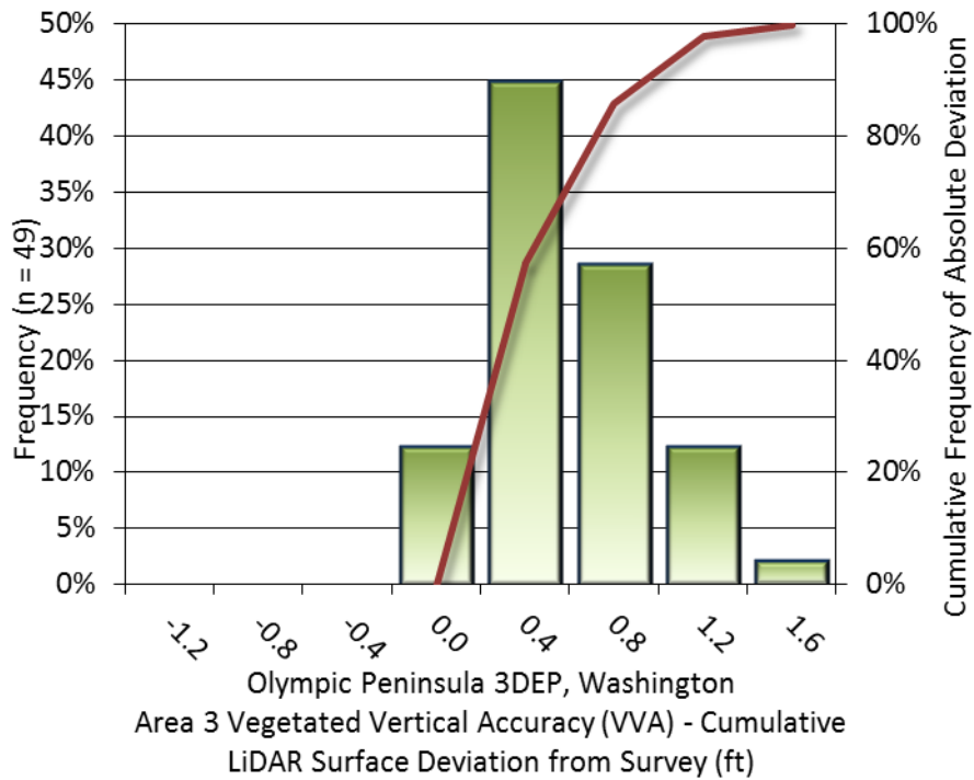
Figure 12: Frequency histogram for LiDAR surface deviation from all land cover class point values (VVA)
