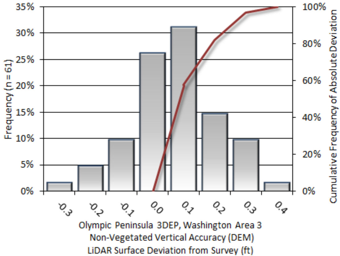
Figure 9: Frequency histogram for LiDAR DEM surface deviation from non-vegetated quality assurance point values
