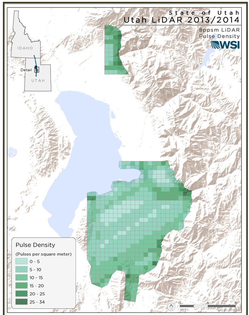
Pulse Density Map for Delivery 5
