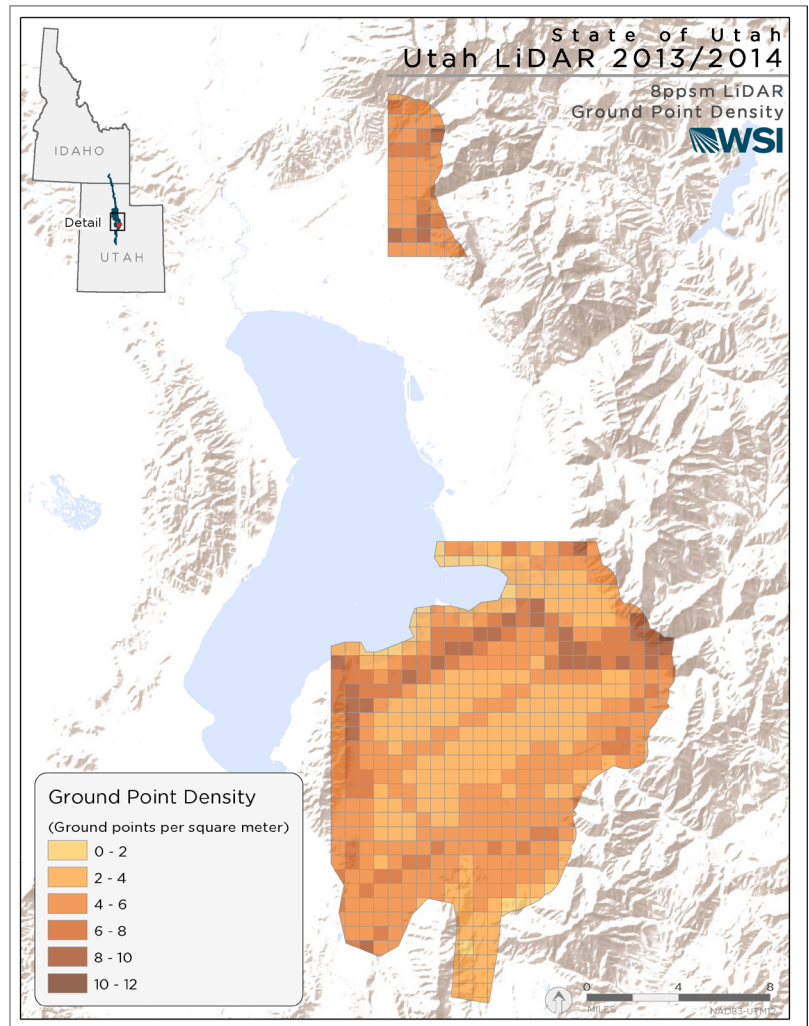
Ground Point Density Map for Delivery 5
