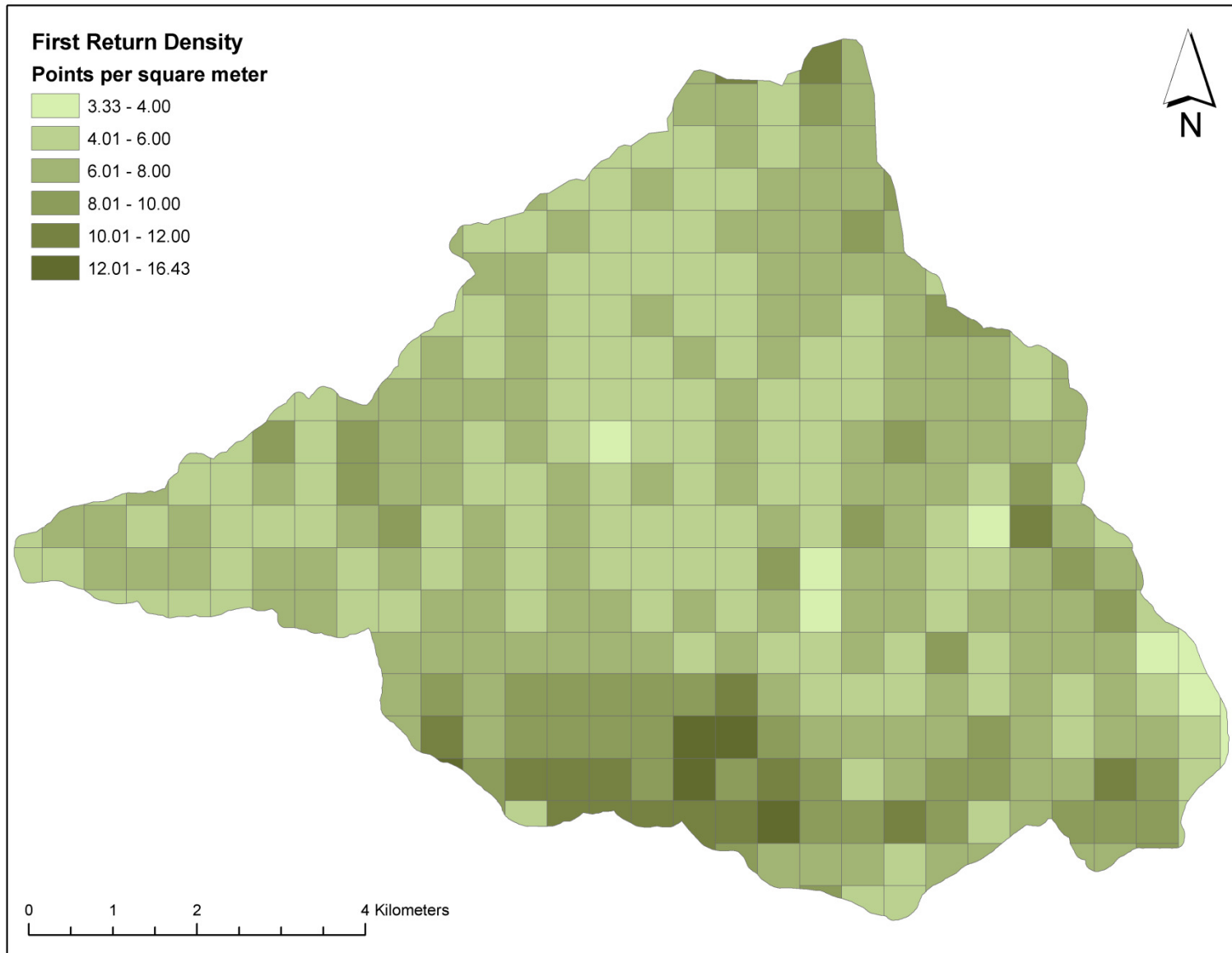
Figure 12. Density distribution map for first return points by processing bin
