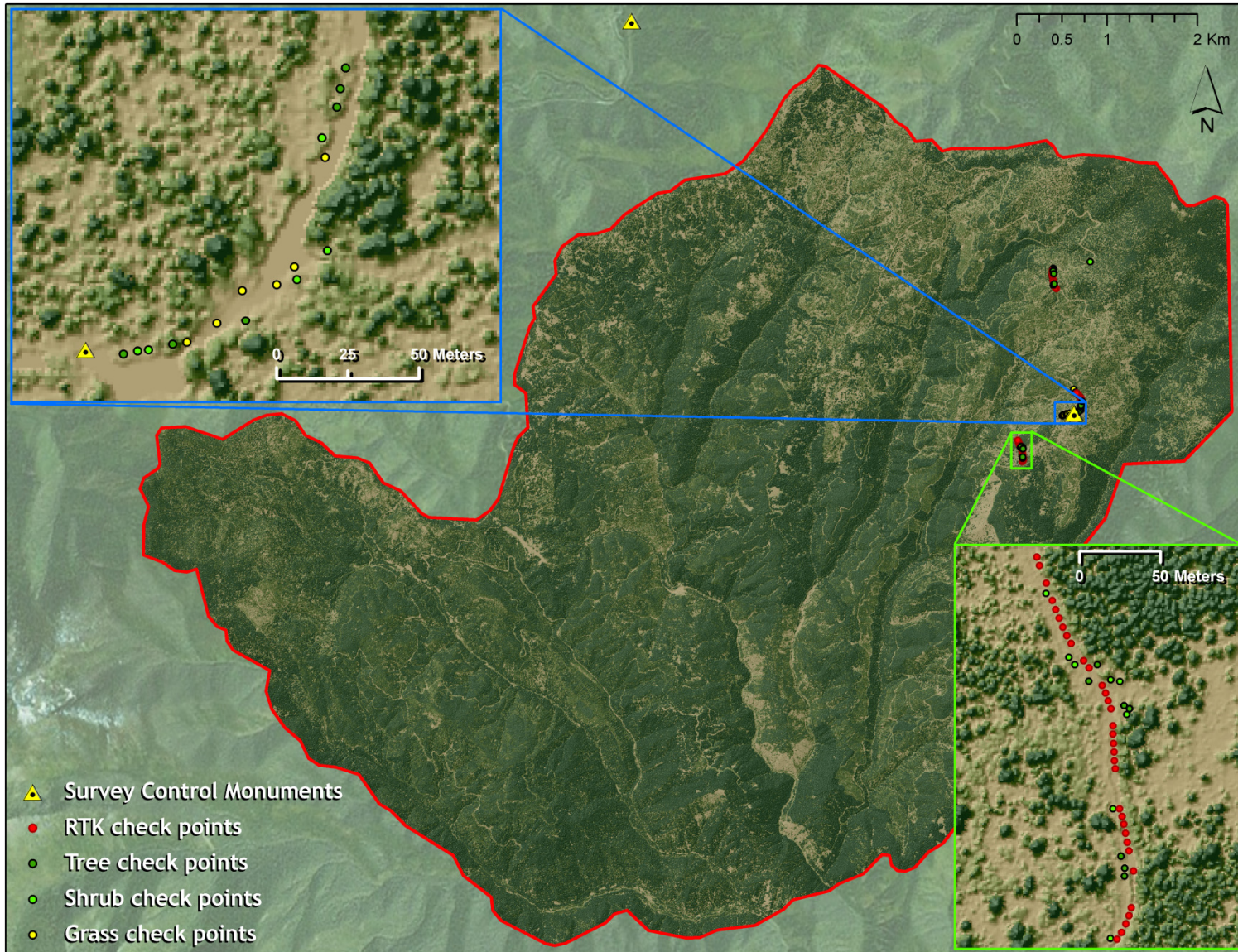
Figure 2. RTK check point, land cover check points, and control monument locations used in the Laundry China Osier AOI
