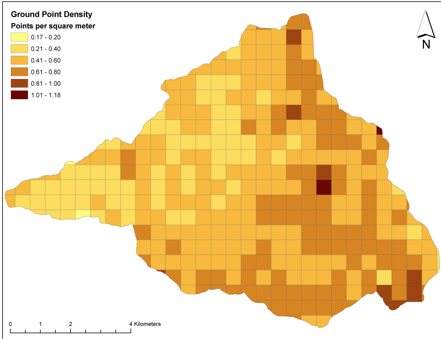
Figure 13. Density distribution map for ground return points by processing bin
