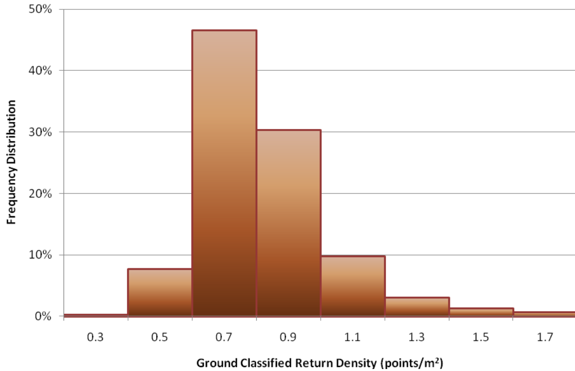
Figure 5. Density distribution for ground classified laser points
