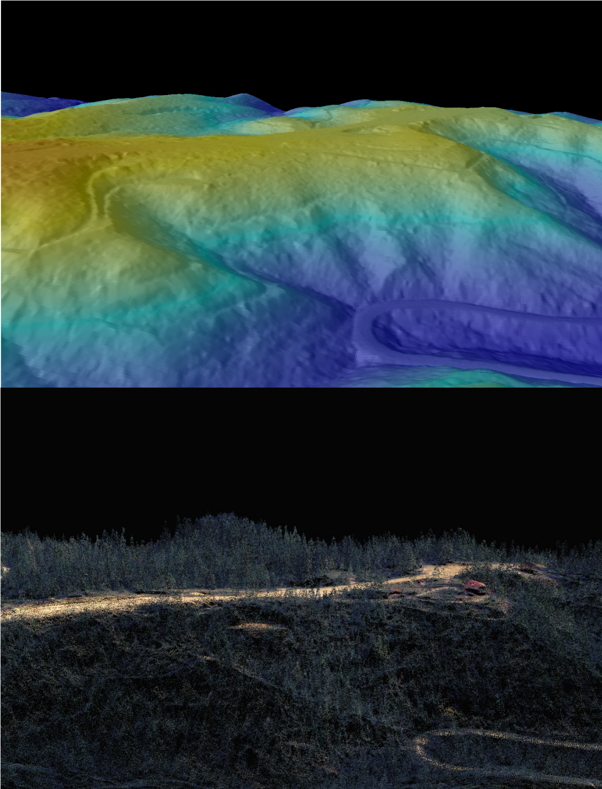
Figure 18. Clearing at the intersection of Moose Creek Rd and County Rd 754 in the China AOI. Top image is bare earth DEM colored by elevation, bottom image is 3D LiDAR point cloud colored by 2009 NAIP imagery.
