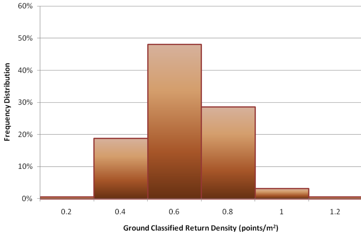
Figure 11. Density distribution for ground classified laser points
