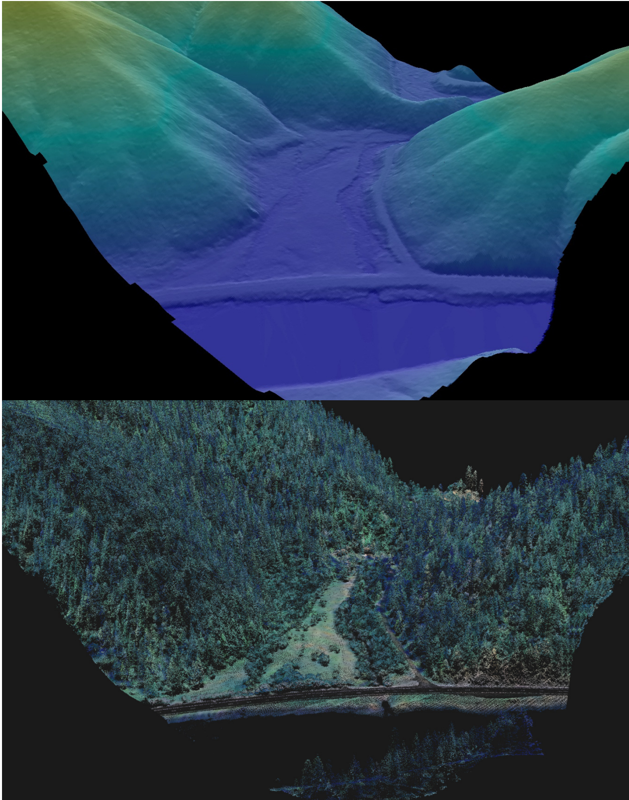
Figure 17. . Intersection of Pete King Road and Hwy 12, looking northwest. Top image is bare earth DEM colored by elevation, bottom image is 3D LiDAR point cloud colored by 2009 NAIP imagery.
