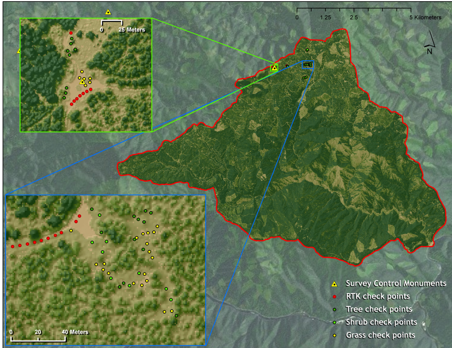
Figure 3. RTK check point, land cover check points, and control monument locations used in the Walde Pete King AOI
