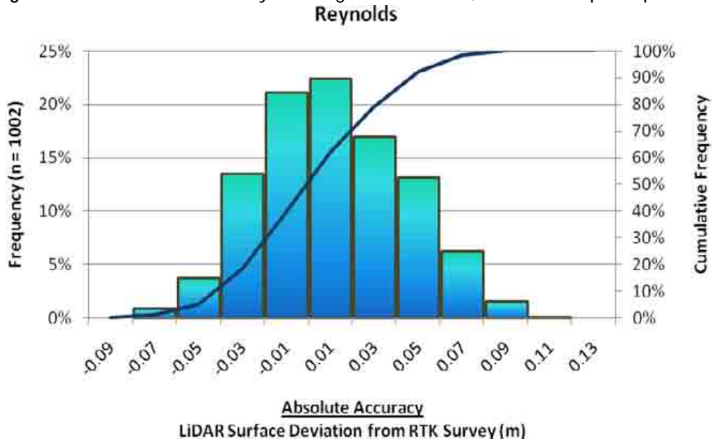
Figure 13. Absolute Accuracy - Absolute Deviation, based on asphalt points
