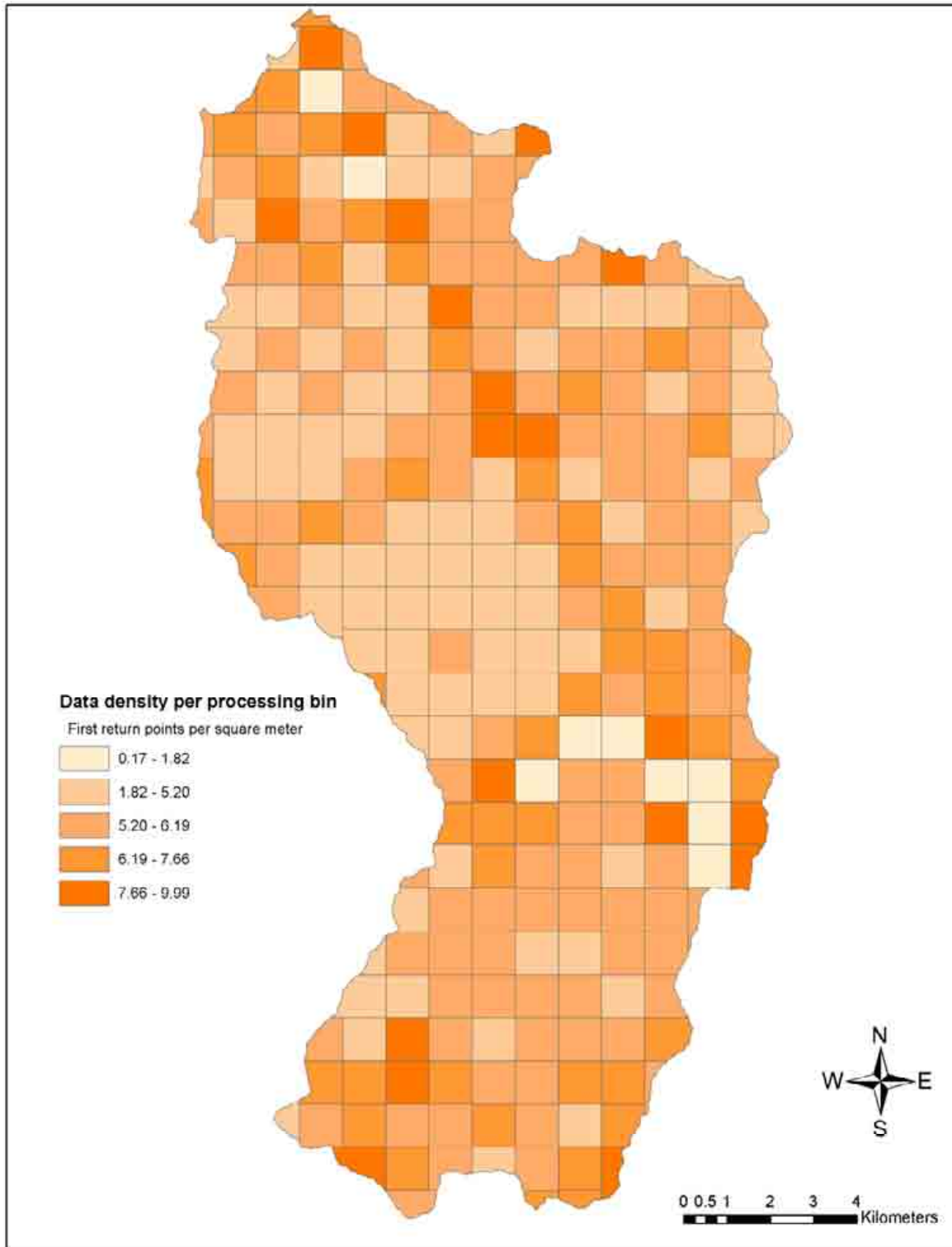
Figure 10. First return data density in the Reynolds Creek AOI, per processing bin.
