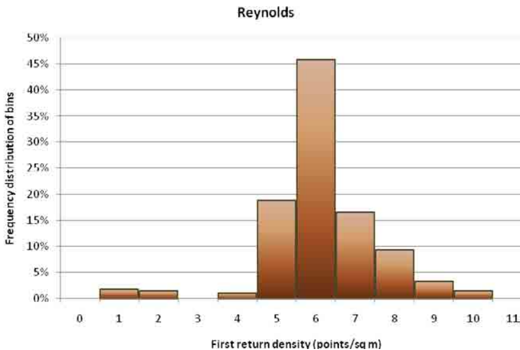
Figure 9. Density distribution for first return laser points.
