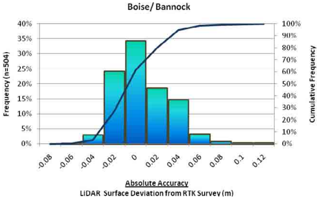
Figure 7. Absolute Accuracy - Absolute Deviation, based on asphalt points
