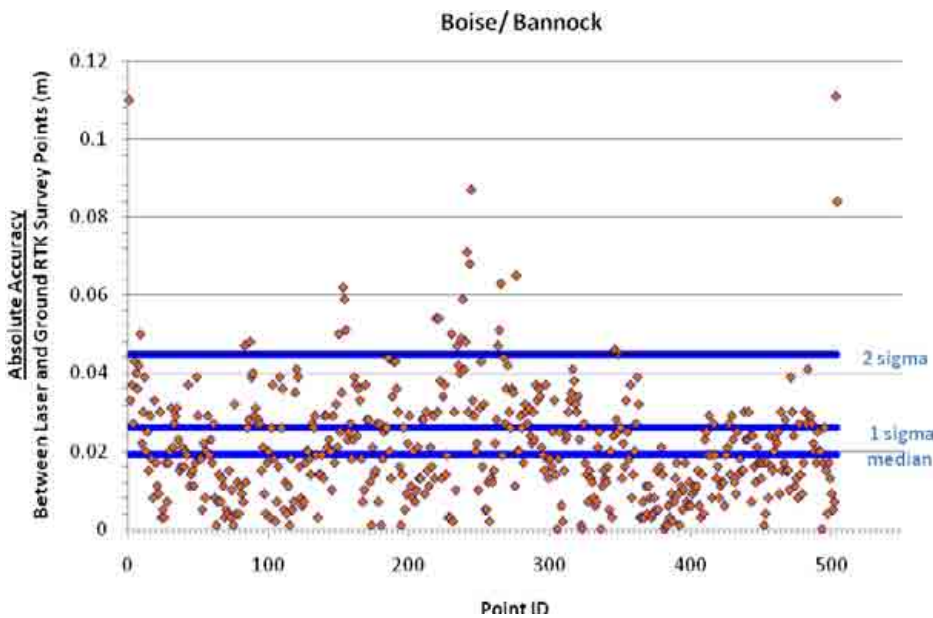
Figure 7. Absolute Accuracy - Absolute Deviation, based on asphalt points
