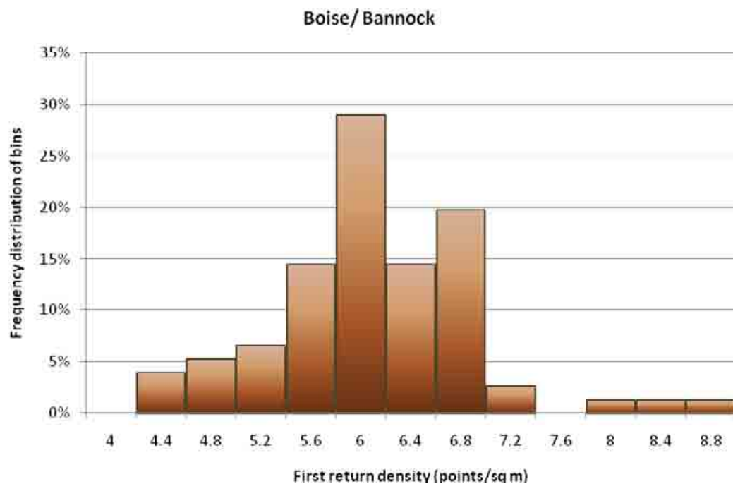
Figure 3. Density distribution for first return laser points.
