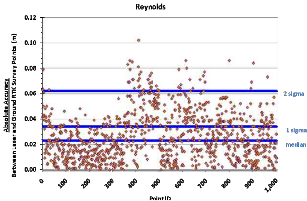
Figure 13. Absolute Accuracy - Absolute Deviation, based on asphalt points
