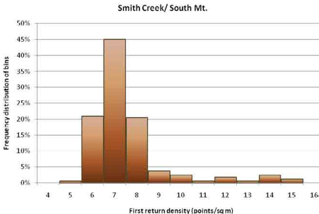
Figure 15. Density distribution for first return laser points.
