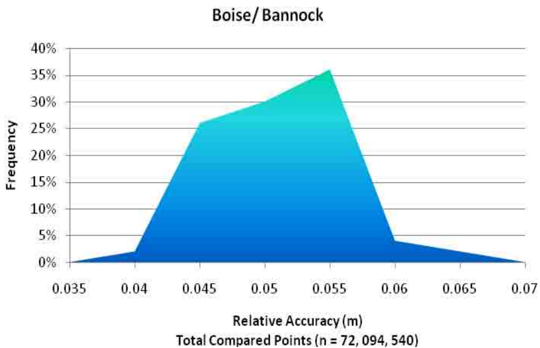
Figure 5. Distribution of relative accuracies per flight line, non slope-adjusted.
