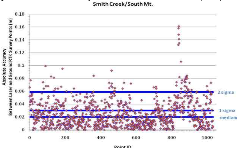
Figure 19. Absolute Accuracy - Absolute Deviation, based on asphalt points
