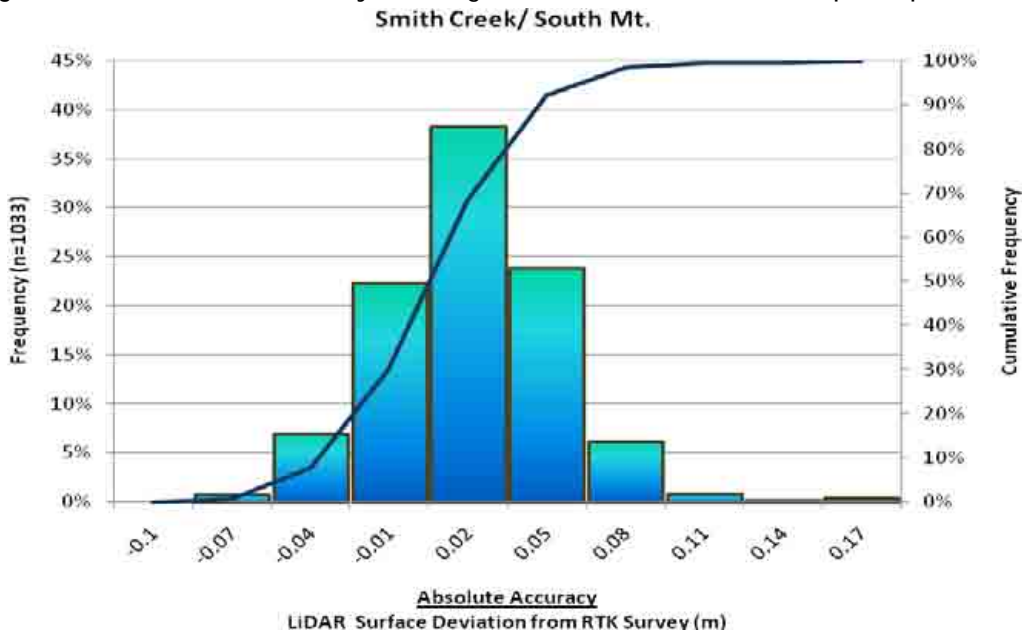
Figure 19. Absolute Accuracy - Absolute Deviation, based on asphalt points
