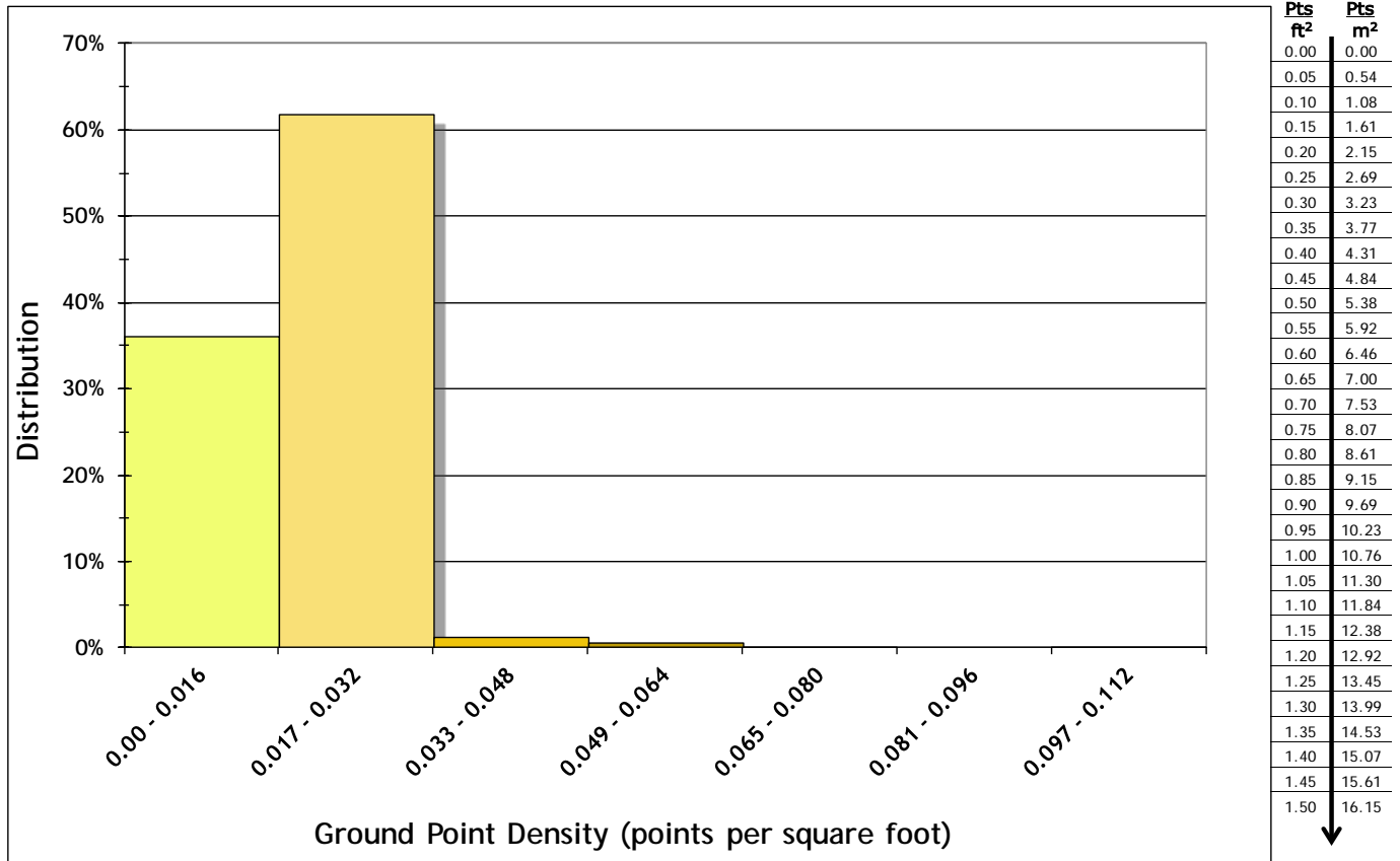
Figure 4.3. Histogram of ground-classified laser point density for entire study area.
