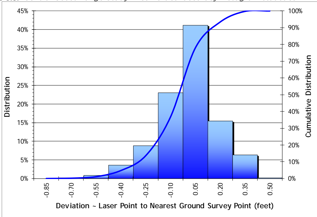
Figure 3.6. Central Coast Range Study Area point absolute deviation statistics.
