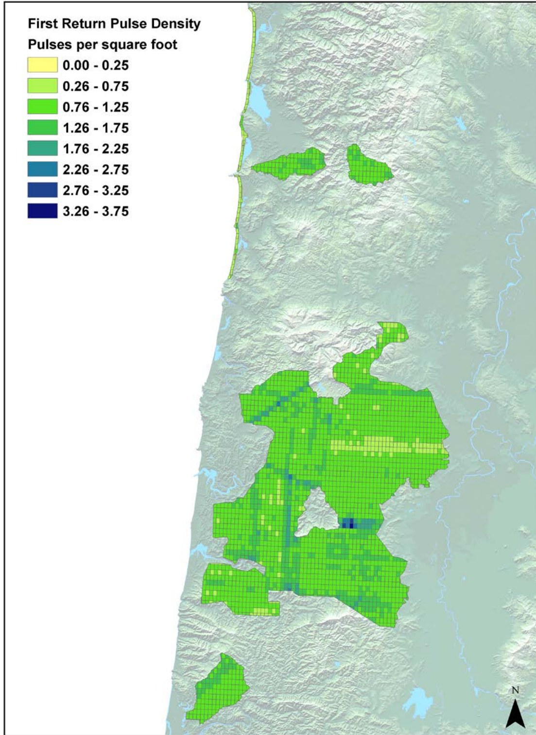
Figure 4.2. First return laser point densities per 0.75' USGS Quad.
