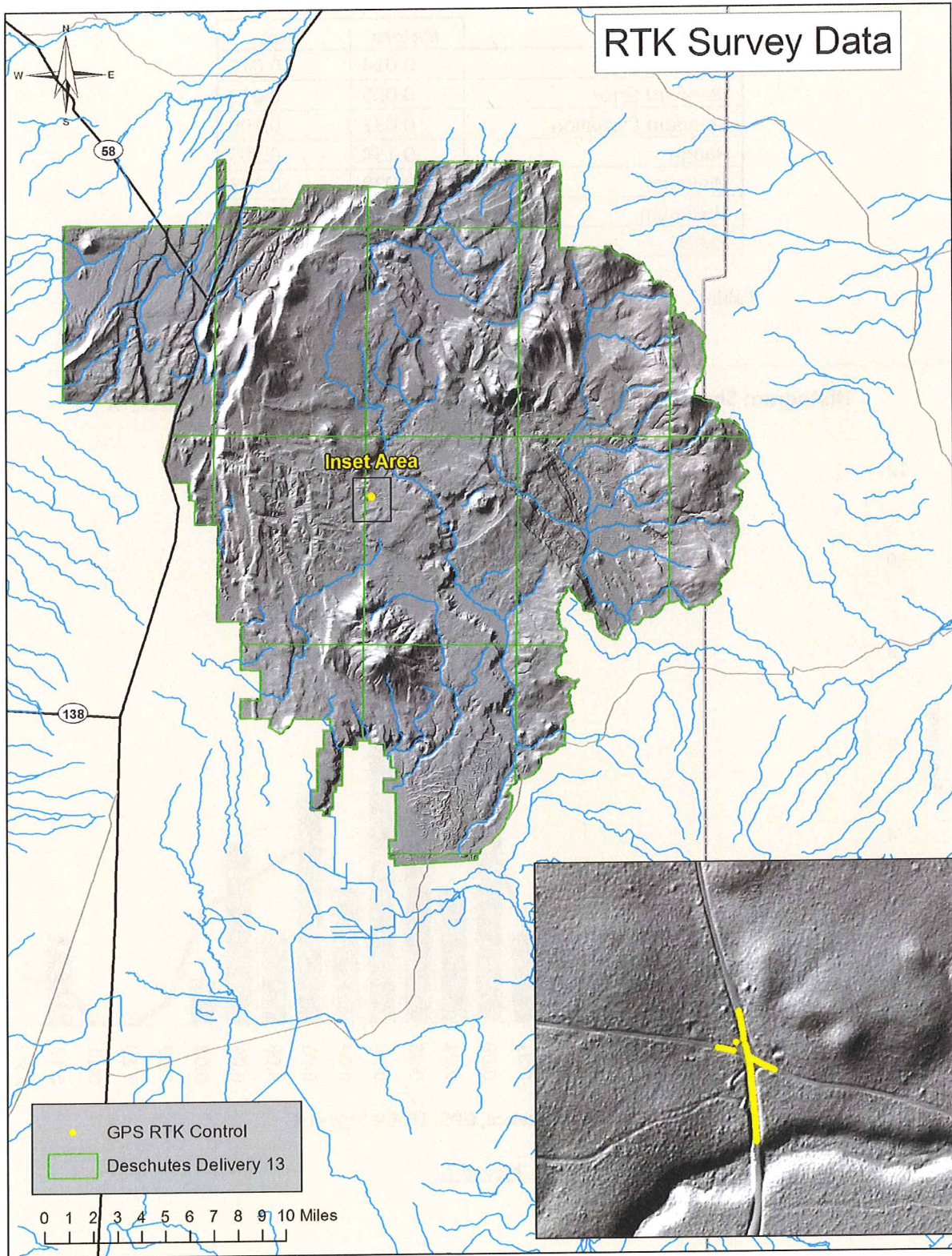
Figure 6. Locations of RTK control surveyed by DOGAMI. Data was used to test absolute accuracy for the Deschutes lidar survey within the Delivery 13 extent.
