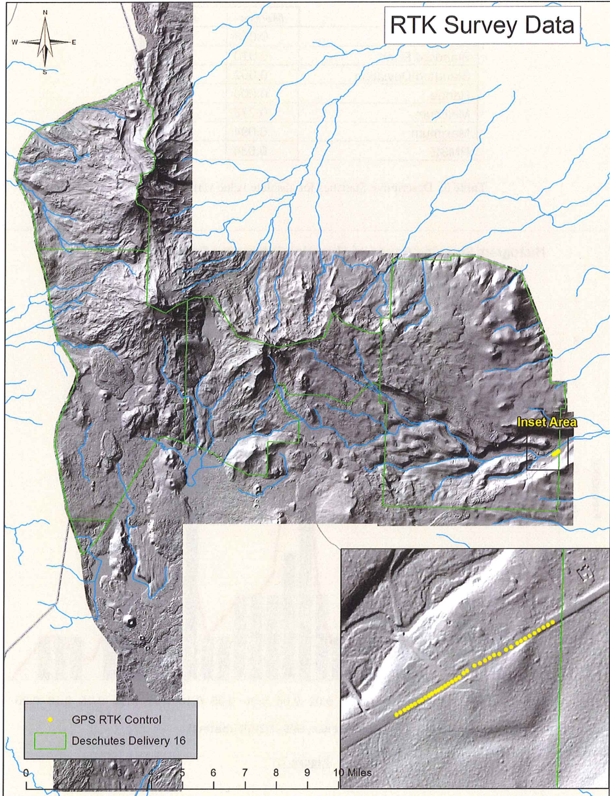
Figure 6. Locations of RTK control surveyed by DOGAMI. Data was used to test absolute accuracy for the Deschutes lidar survey within the Delivery 16 extent.
