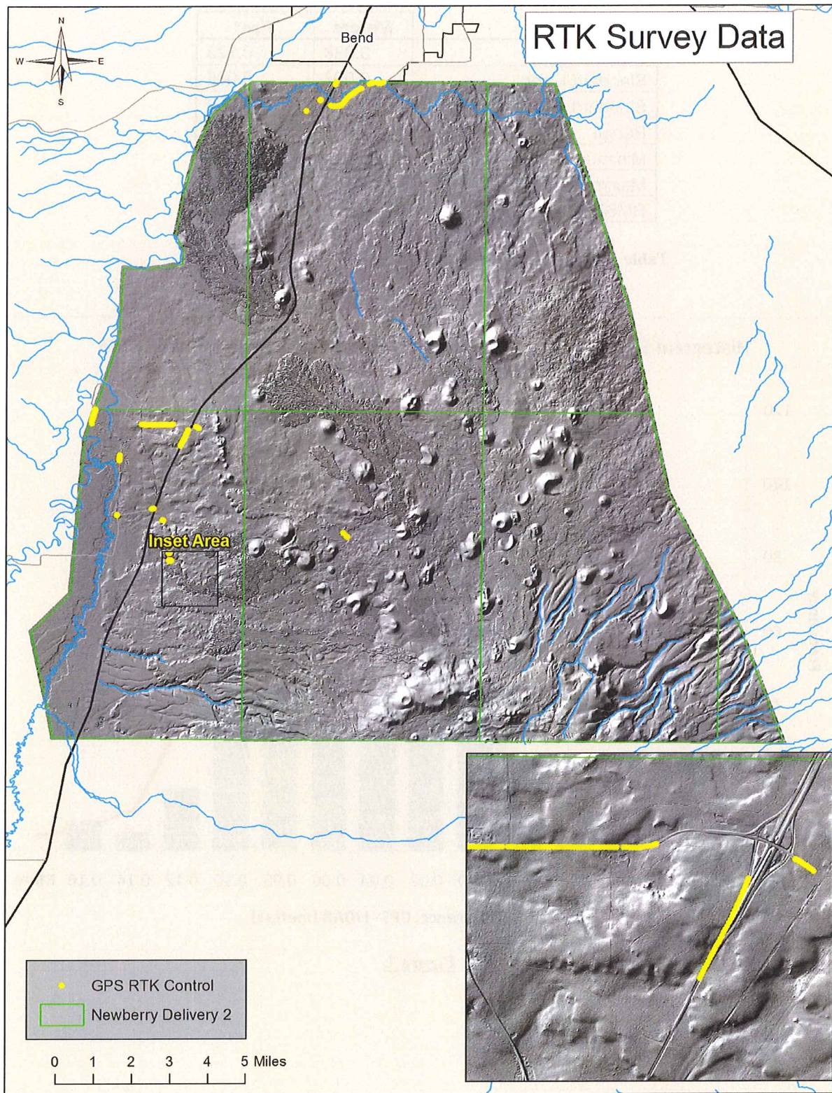
Figure 6. Locations of RTK control surveyed by DOGAMI. Data was used to test absolute accuracy for the Newberry CVO lidar survey within the Delivery 2 extent.
