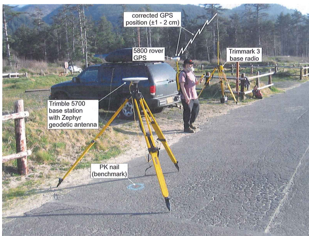
Figure 5. The Trimble 5700 base station antenna located over a known reference point at Cape Lookout State Park. Corrected GPS position and elevation information is then transmitted by a Trimmark III base radio to the 5800 GPS rover unit.
