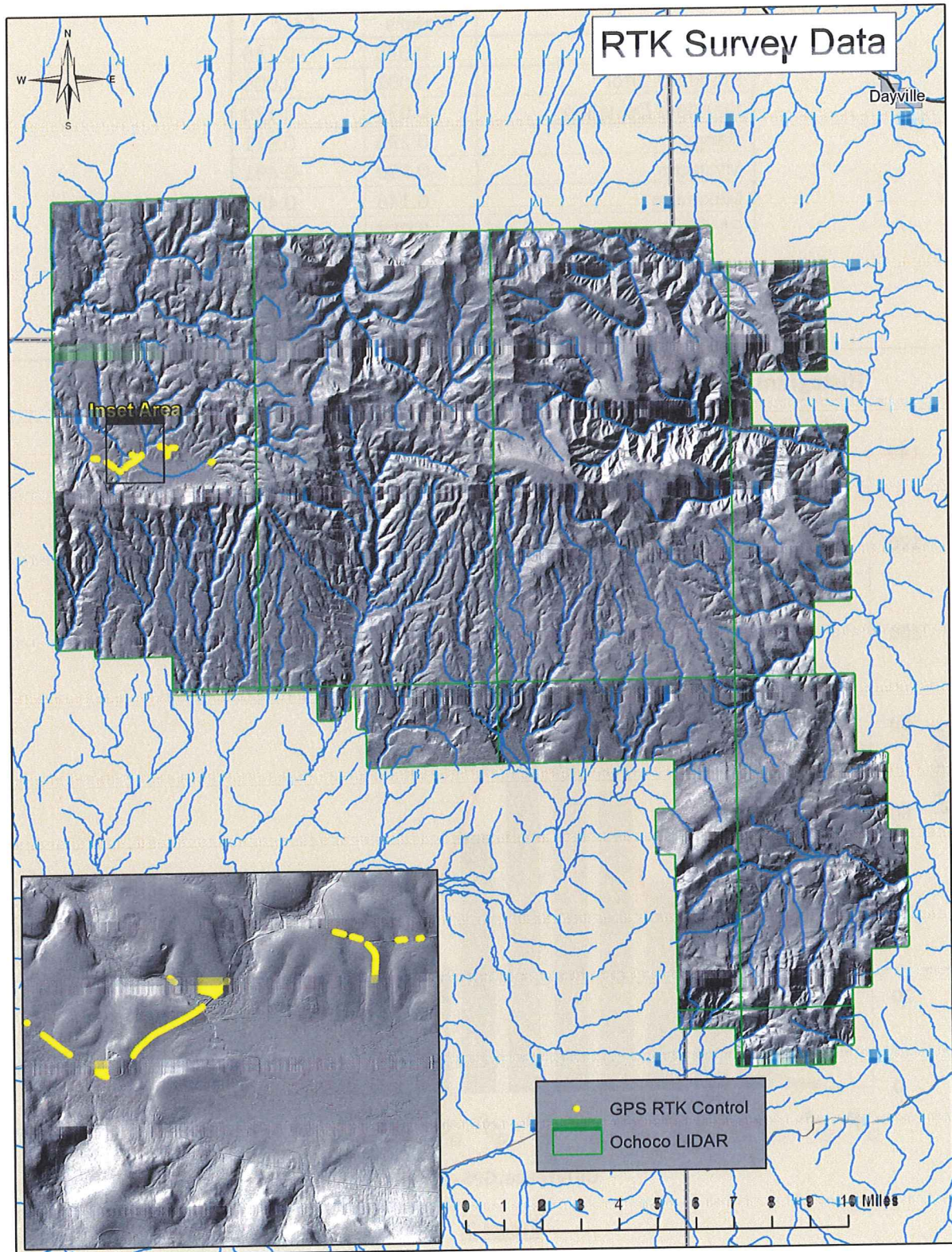
Figure 6. Locations of RTK control surveyed by DOGAMI. Data was used to test absolute accuracy for the Ochoco lidar survey within the Delivery extent.
