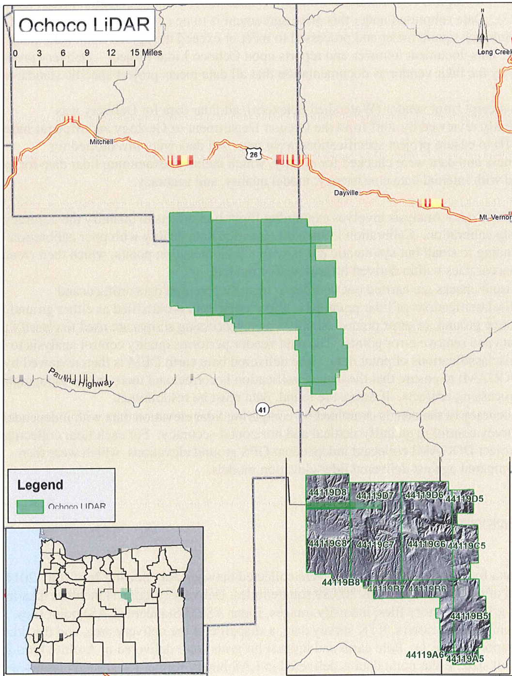
Map featuring Ochoco Delivery data extent.
