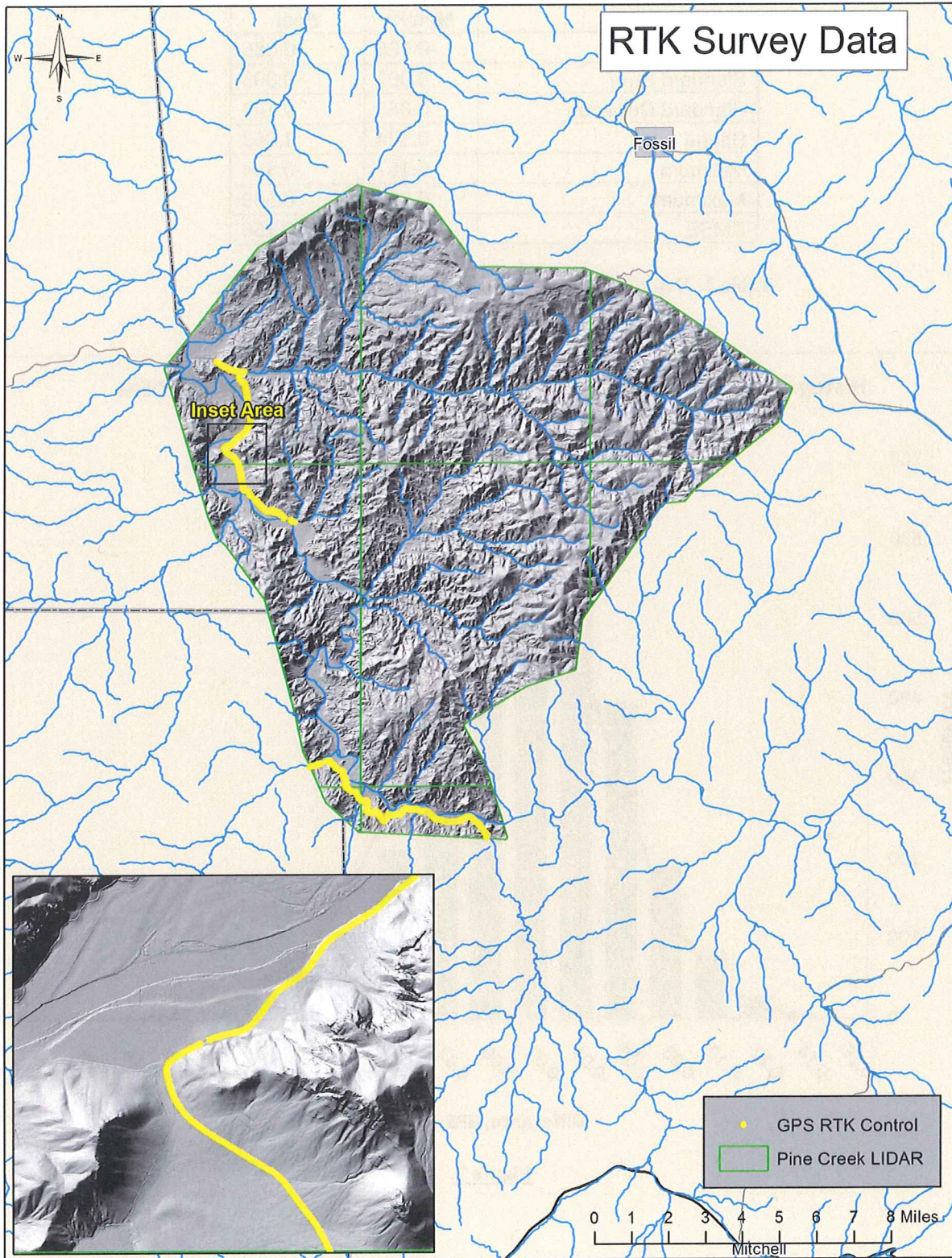
Figure 6. Locations of RTK control surveyed by DOGAMI. Data was used to test absolute accuracy for the Pine Creek lidar survey within the Delivery extent.
