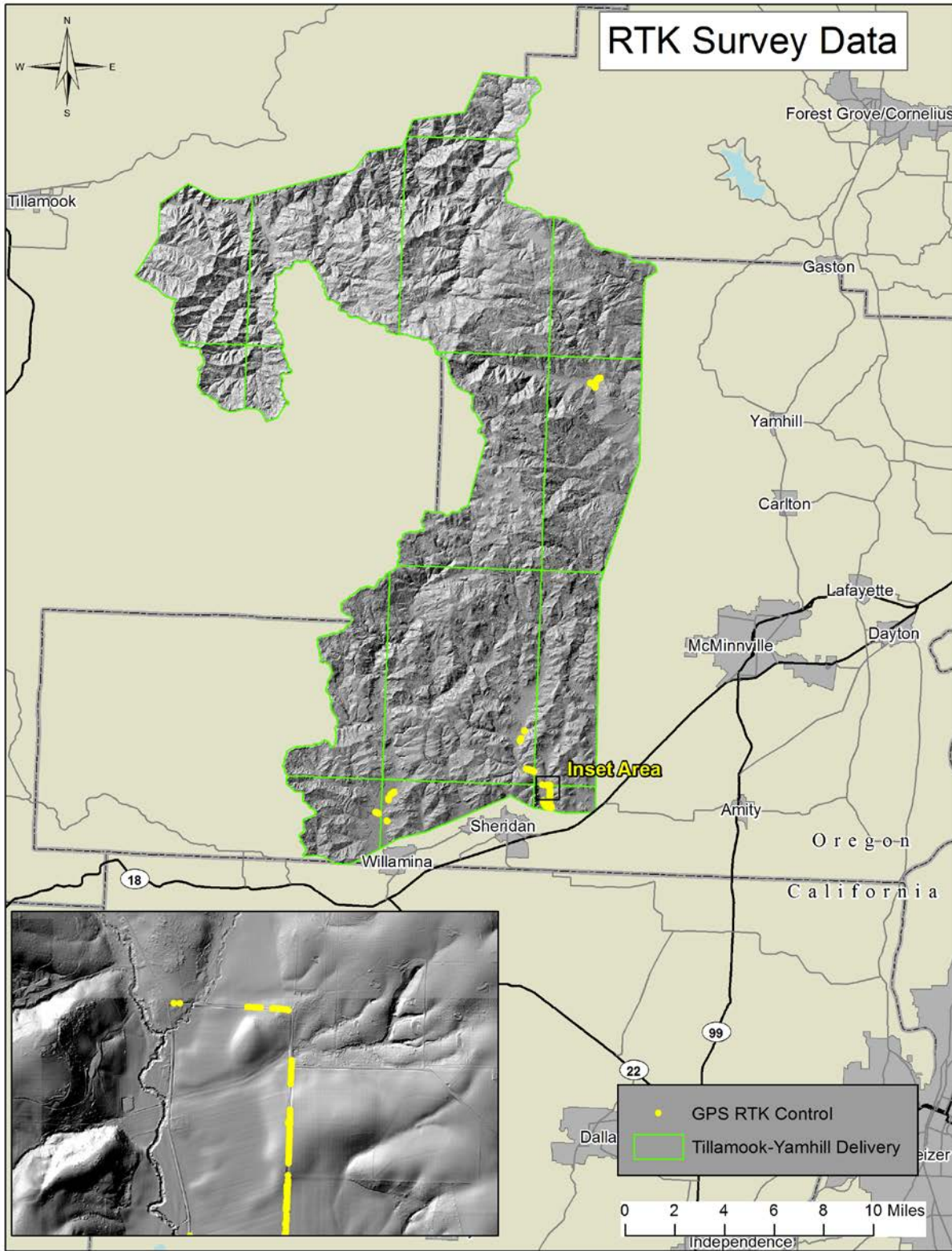
Figure 6. Locations of RTK control surveyed by DOGAMI. Data was used to test absolute accuracy for the Tillamook-Yamhill lidar survey within the Delivery extent.
