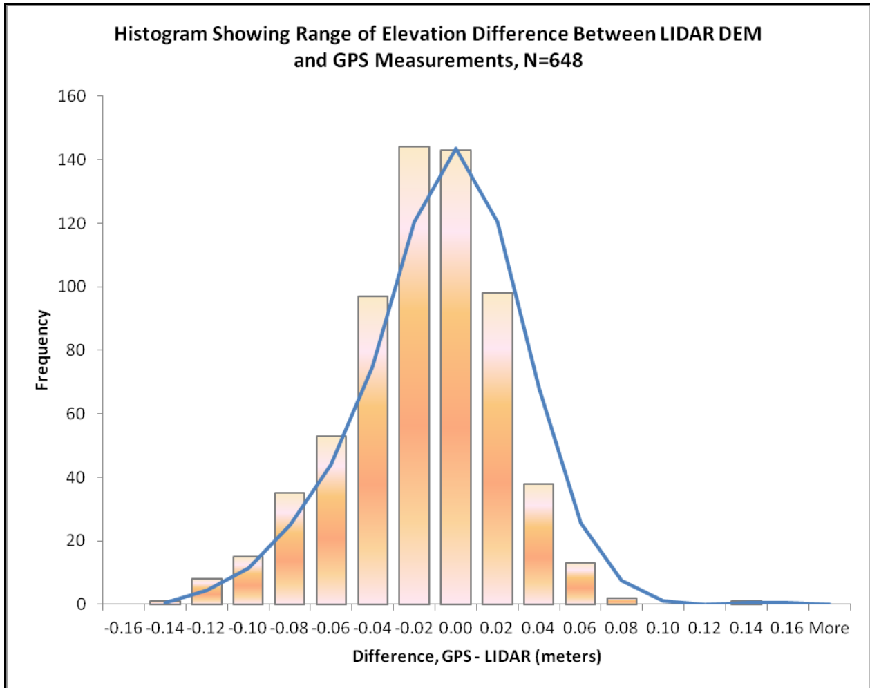
Figure 7. Histogram of absolute vertical accuracy
