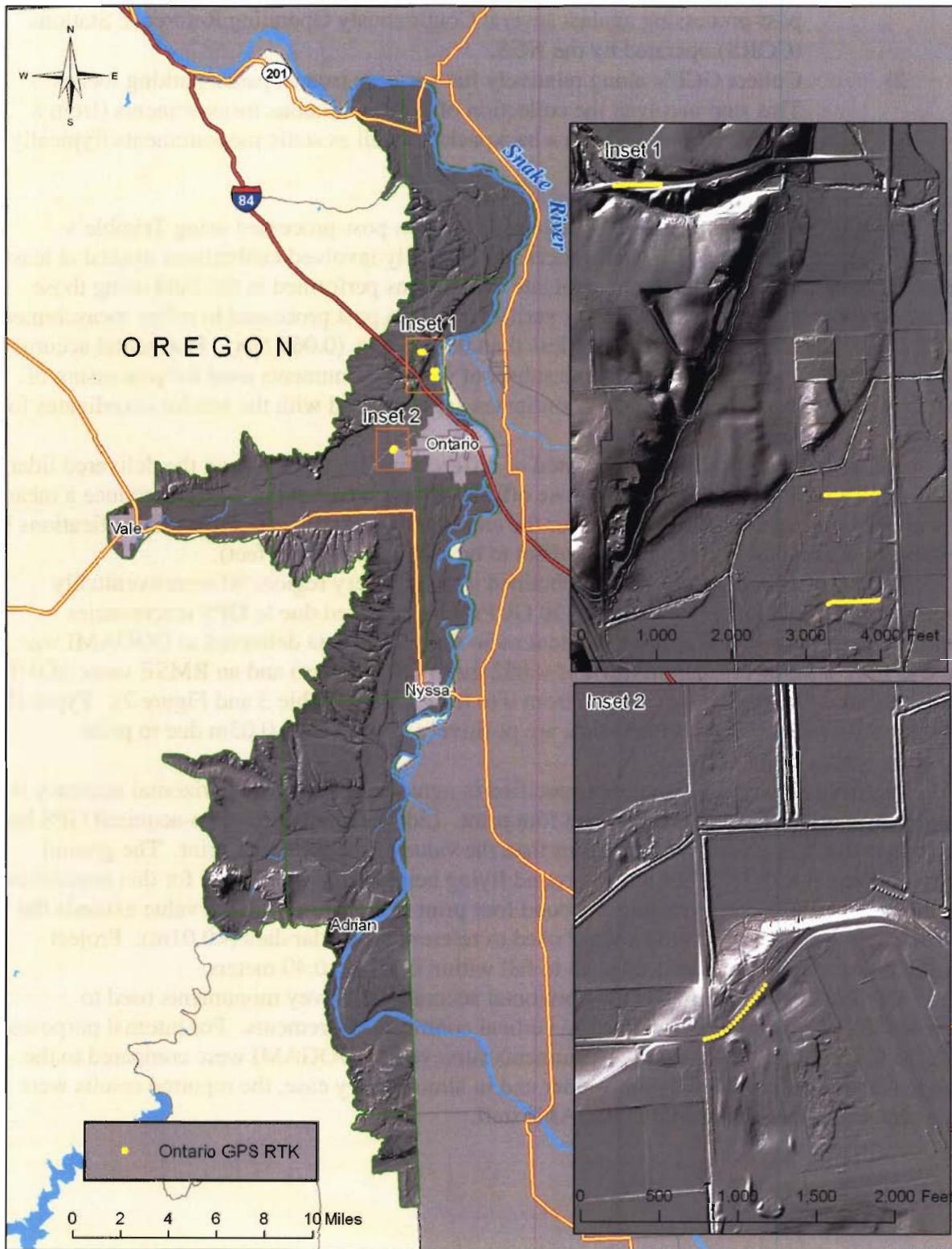
Figure 6. Locations of RTK control surveyed by DOGAMI. Data was used to test absolute accuracy for the Ontario lidar survey within the extent.
