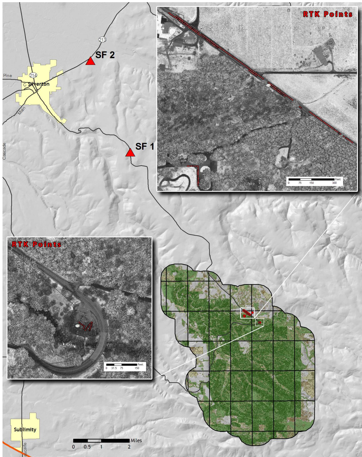
Figure 3. Locations of Base Stations and RTK Survey Point Collection in the Silver Falls State Park study area (2 Base Stations and 535 RTK Points). Details of RTK point collection locations shown on 1.5-foot resolution intensity images.
