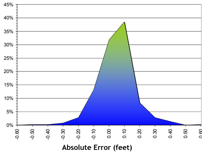
Figure 9. Point Absolute Deviation Statistics
