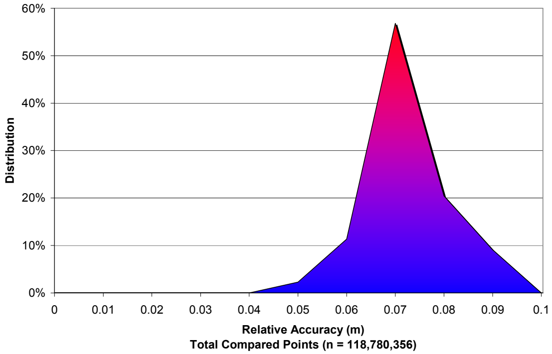
Figure 6. Distribution of relative accuracies per flight line.
