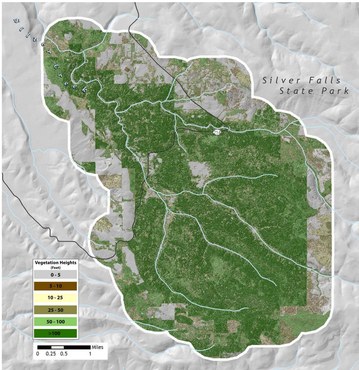
Figure 1. Full extent of Silver Falls State Park study area, covering ~15,811 acres, including a 0.5 mile buffer. Image shows 3-foot resolution Above Ground grid with 10-meter DEM in background. (To calculate vegetation heights shown in the map, the Bare Earth grid was subtracted from the Above Ground grid).
