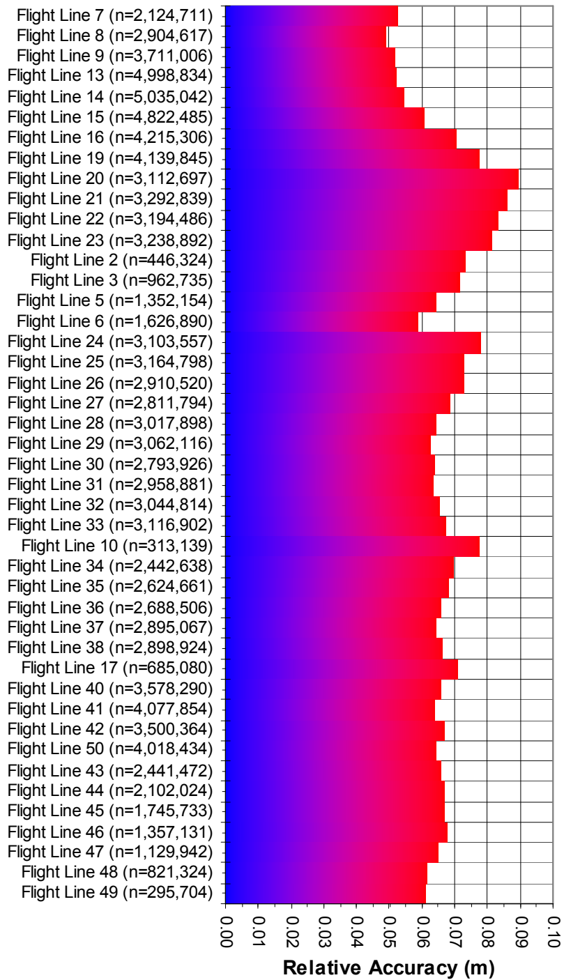
Figure 5. Relative accuracy per flight line with overlapping point totals listed as 'n'.
