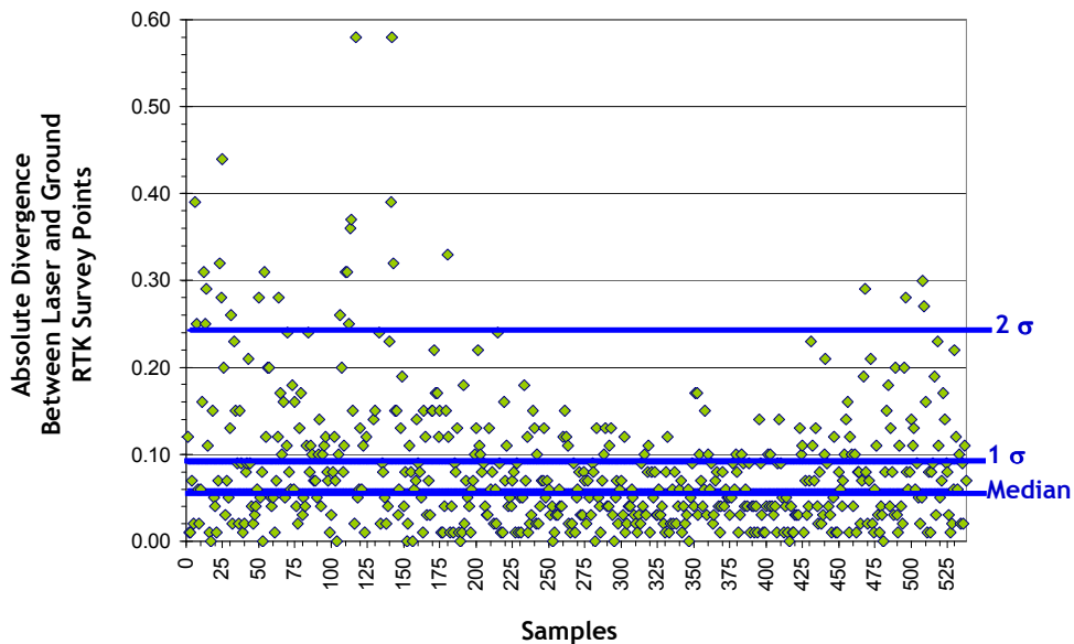
Figure 9. Point Absolute Deviation Statistics
