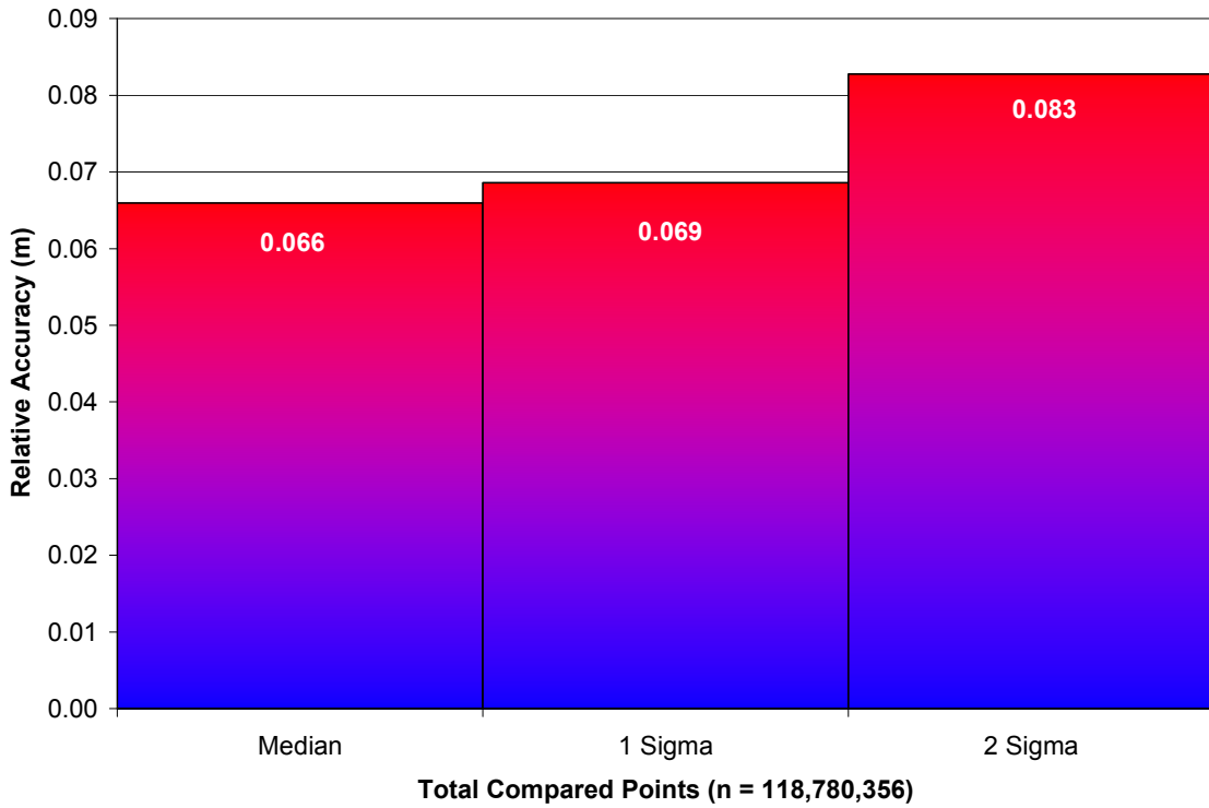
Figure 7. Statistical relative accuracies.
