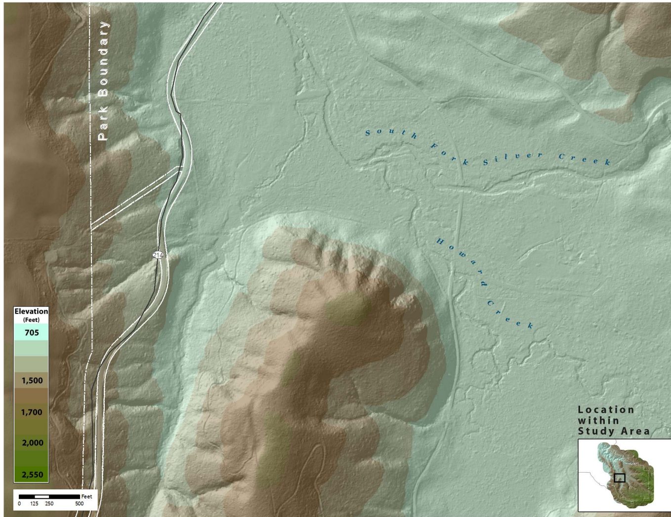
Figure 10. Bare Earth 3-foot resolution ESRI grid showing detail of the confluence of Howard Creek and South Fork Silver Creek.
