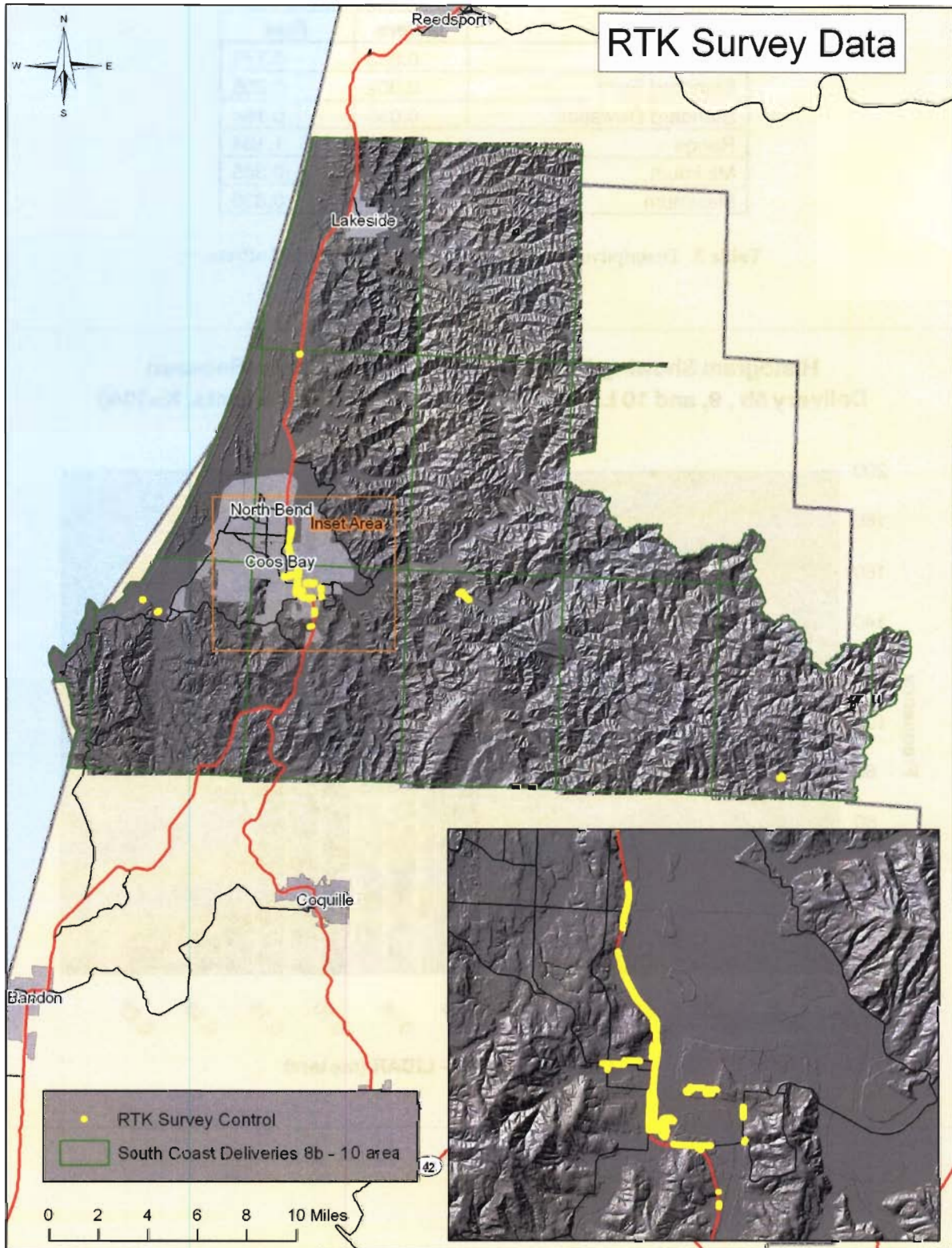
Figure 6. Locations of RTK control surveyed by DOGAMI. Data was used to test absolute accuracy for the South Coast lidar survey within the delivery extent.
